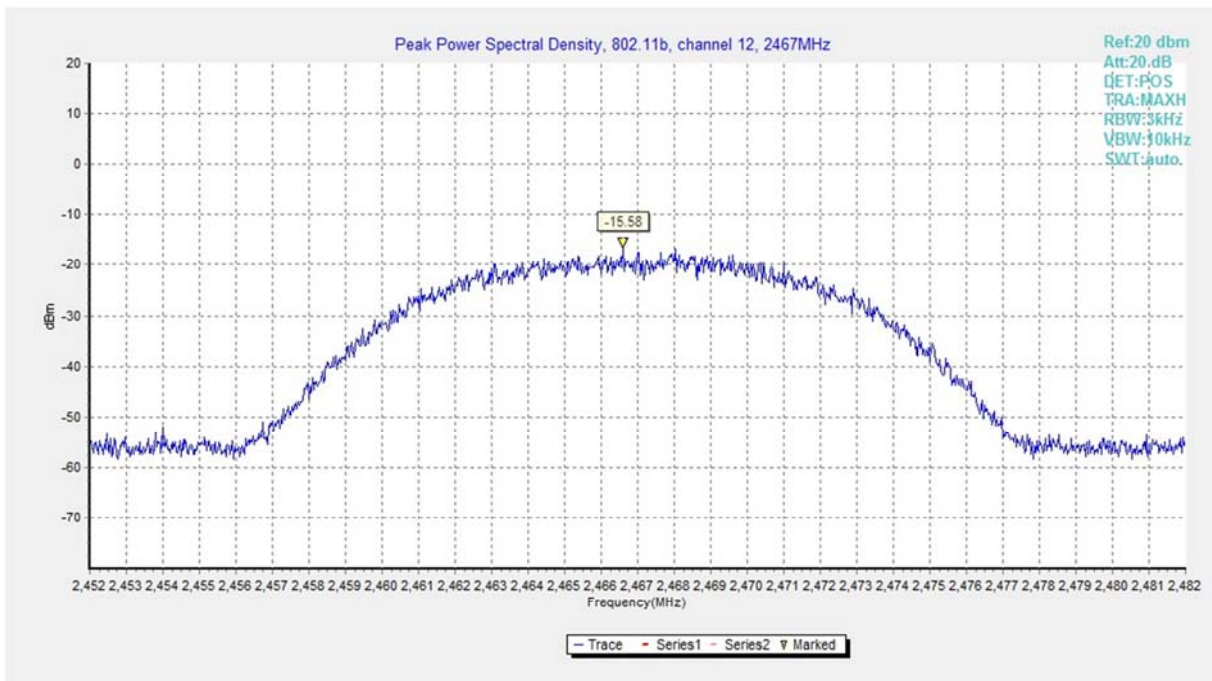
Fig.A.3.4 Power Spectral Density (802.11b, Ch 12)
