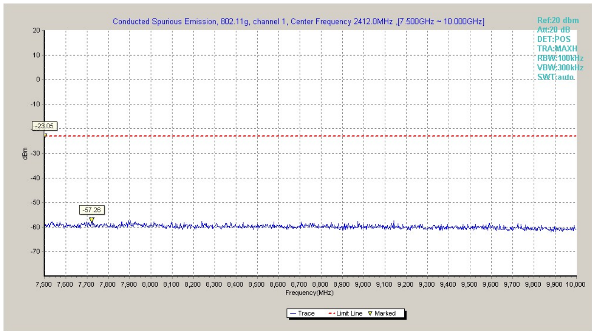
Fig.A.6.1.45 Transmitter Spurious Emission - Conducted (802.11g, Ch1, 7.5 GHz-10 GHz)
