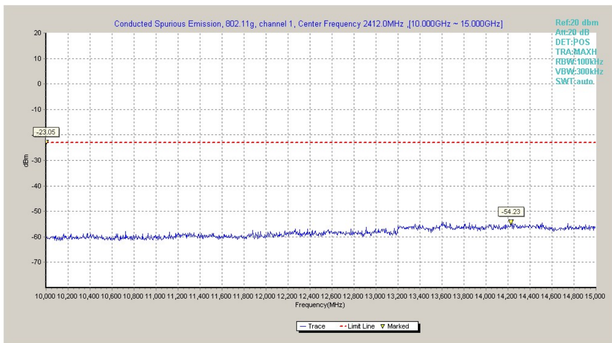
Fig.A.6.1.46 Transmitter Spurious Emission - Conducted (802.11g, Ch1, 10 GHz-15 GHz)
