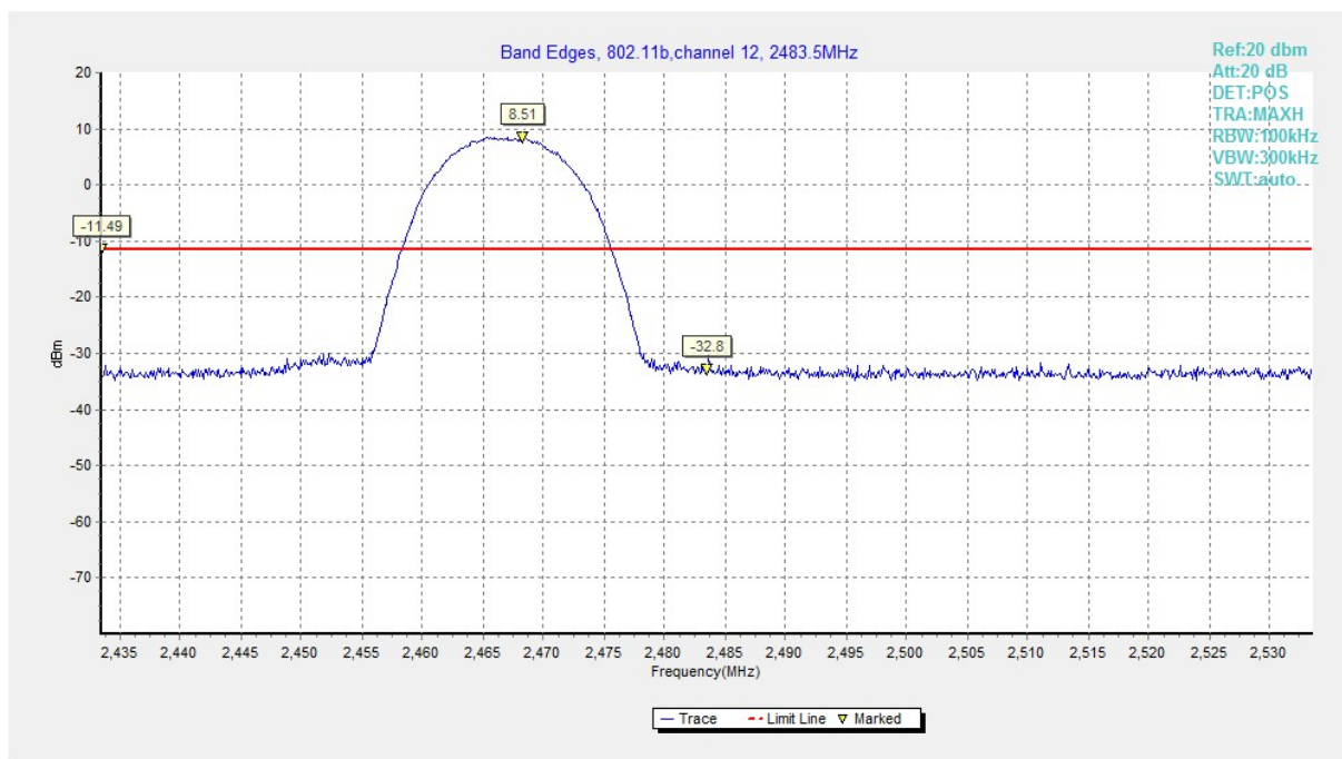
Fig.A.5.3 Band Edges (802.11b, Ch 12)
