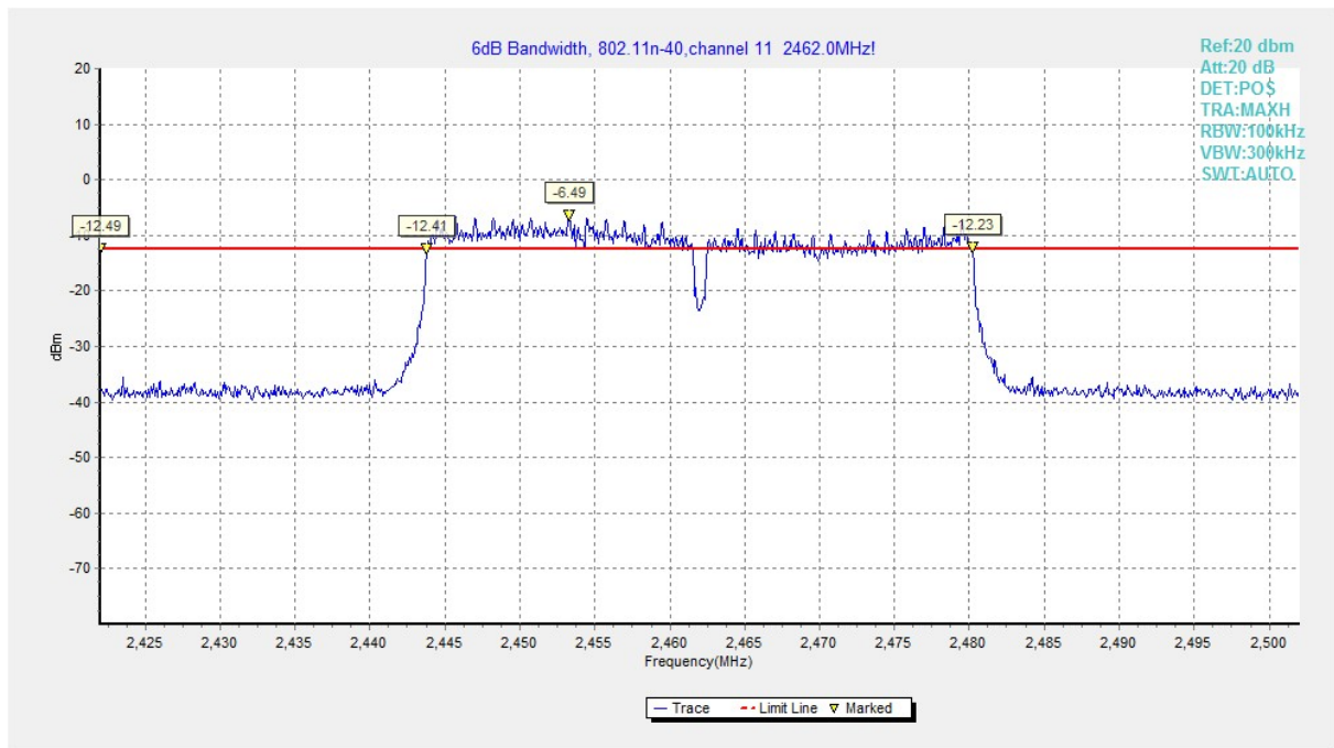
Fig.A.4.20 Occupied 6dB Bandwidth (802.11n-HT40, Ch 11)
