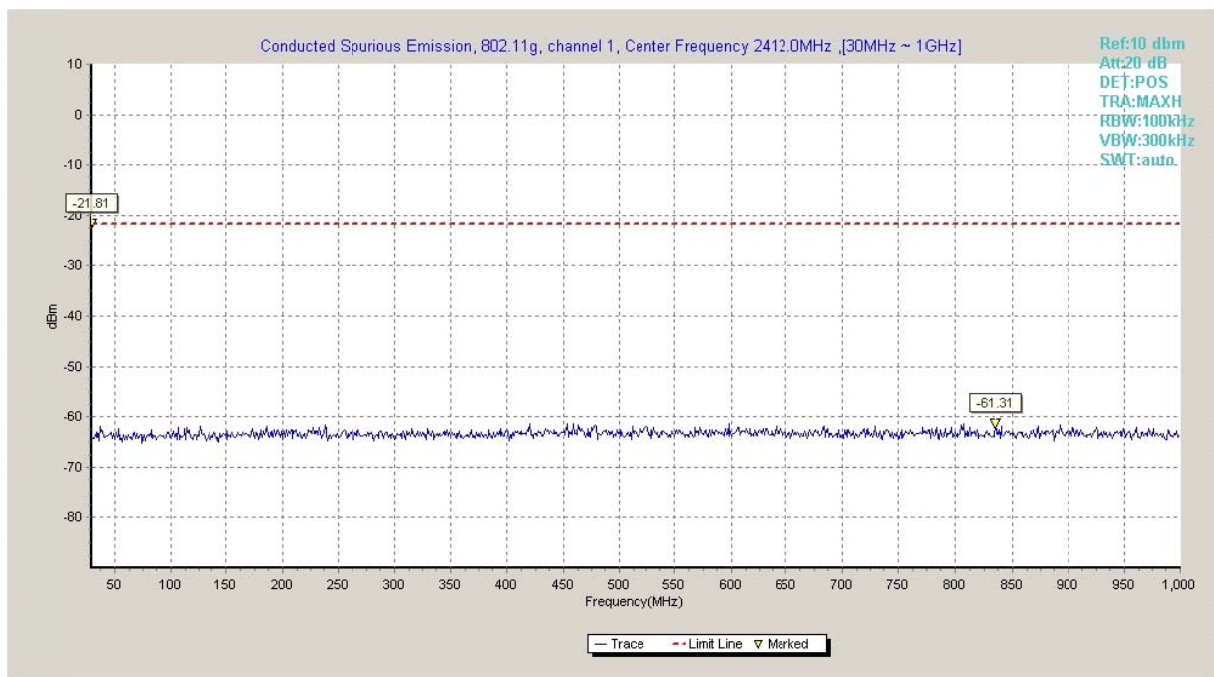
Fig.A.6.1.42 Transmitter Spurious Emission - Conducted (802.11g, Ch1, 30 MHz-1 GHz)
