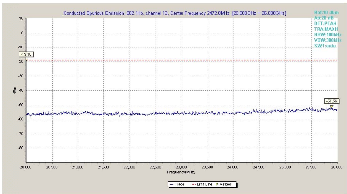
Fig.A.6.1.40 Transmitter Spurious Emission - Conducted (802.11b, Ch13, 20 GHz-26 GHz)
