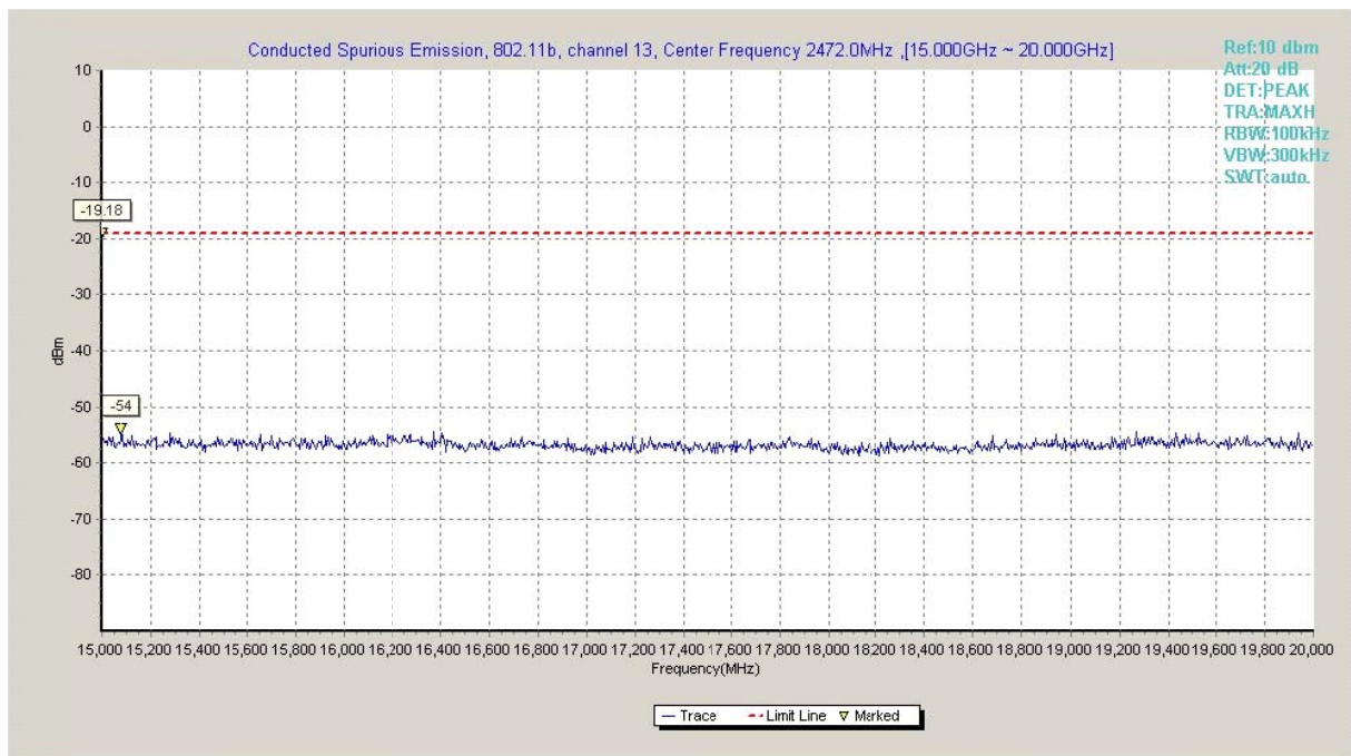
Fig.A.6.1.39 Transmitter Spurious Emission - Conducted (802.11b, Ch13, 15 GHz-20 GHz)
