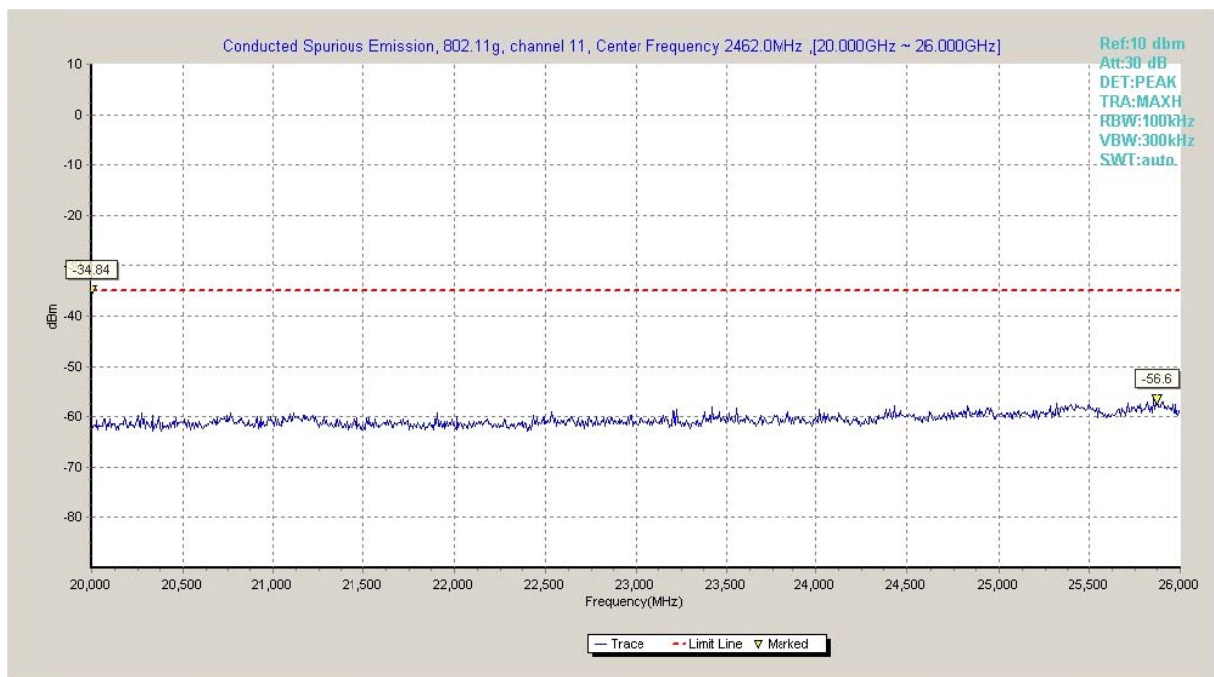
Fig.A.6.1.64 Transmitter Spurious Emission - Conducted (802.11g, Ch11, 20 GHz-26 GHz)
