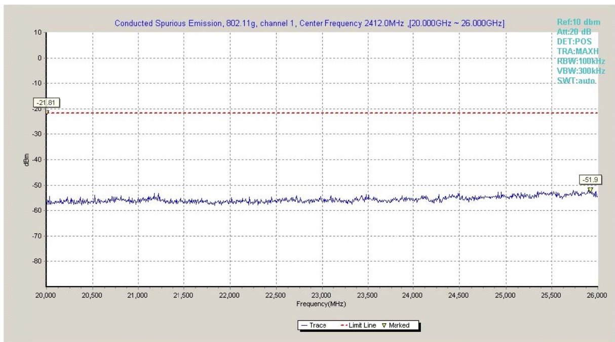
Fig.A.6.1.48 Transmitter Spurious Emission - Conducted (802.11g, Ch1, 20 GHz-26 GHz)
