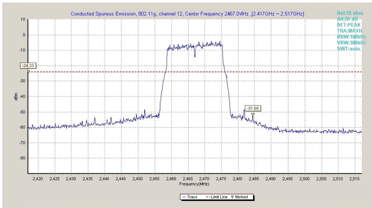
Fig.A.6.1.65 Transmitter Spurious Emission - Conducted (802.11g, Ch12, Center Frequency)
