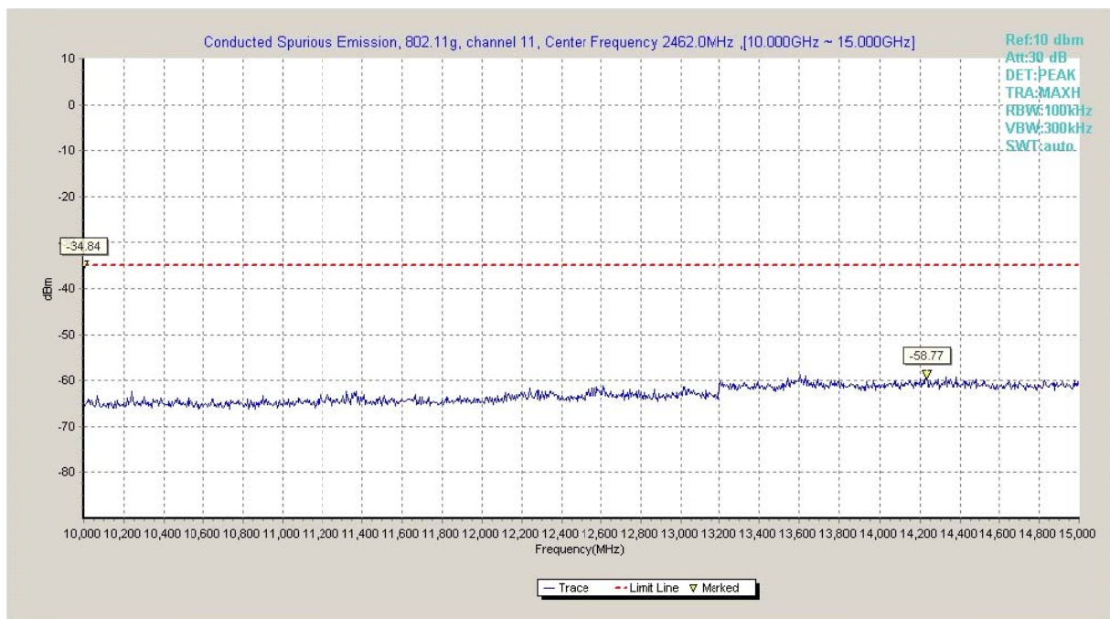
Fig.A.6.1.62 Transmitter Spurious Emission - Conducted (802.11g, Ch11, 10 GHz-15 GHz)
