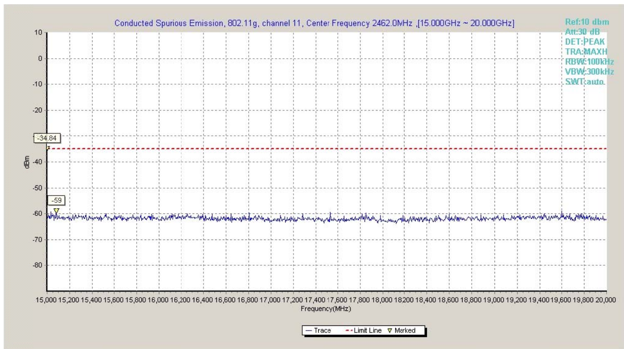
Fig.A.6.1.63 Transmitter Spurious Emission - Conducted (802.11g, Ch11, 15 GHz-20 GHz)
