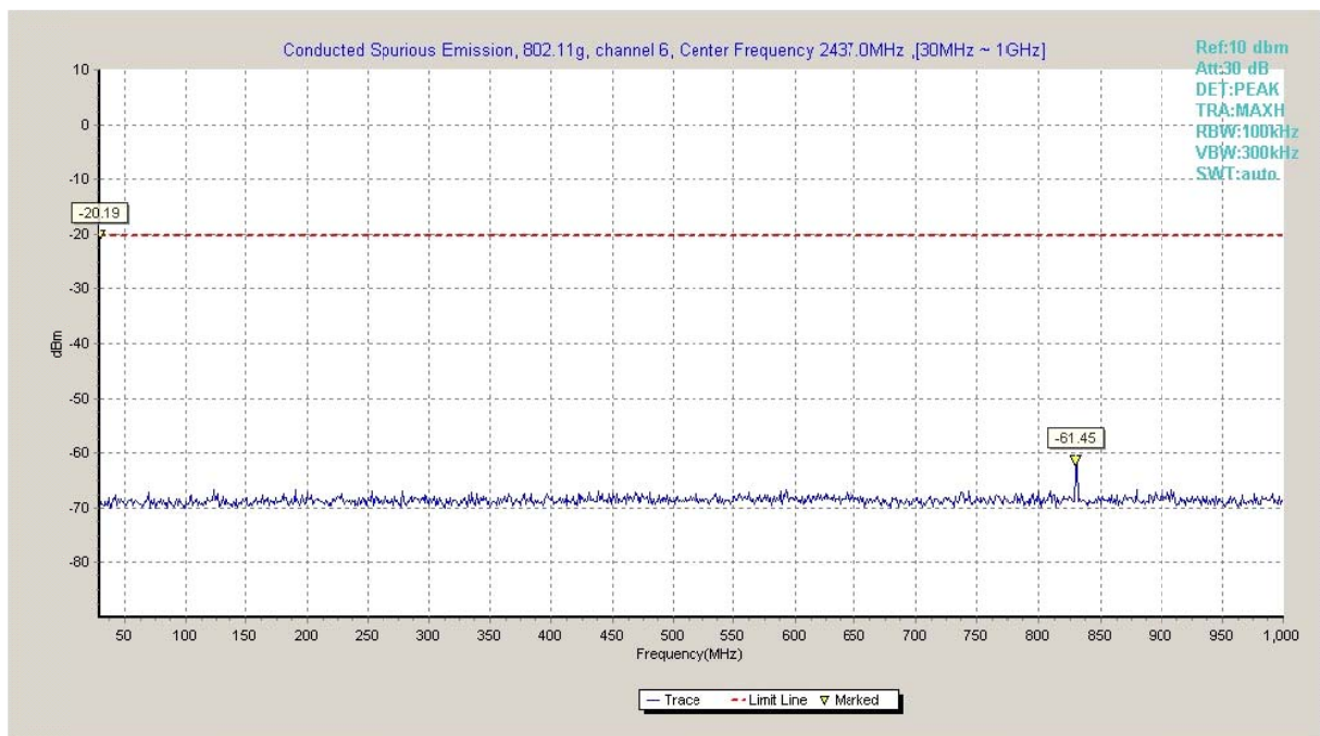
Fig.A.6.1.50 Transmitter Spurious Emission - Conducted (802.11g, Ch6, 30 MHz-1 GHz)
