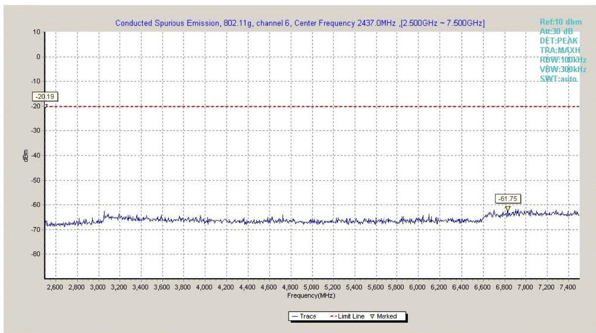
Fig.A.6.1.52 Transmitter Spurious Emission - Conducted (802.11g, Ch6, 2.5 GHz-7.5 GHz)
