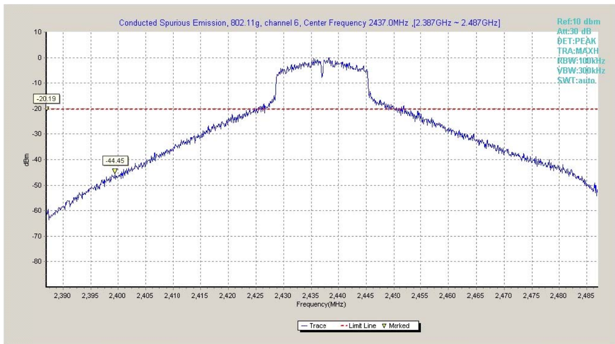
Fig.A.6.1.49 Transmitter Spurious Emission - Conducted (802.11g, Ch6, Center Frequency)
