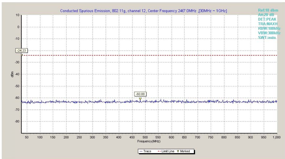
Fig.A.6.1.66 Transmitter Spurious Emission - Conducted (802.11g, Ch12, 30 MHz-1 GHz)
