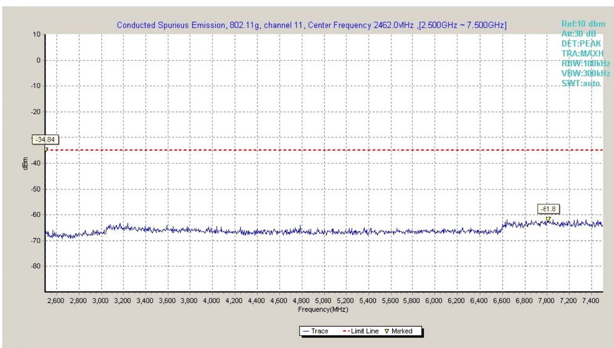
Fig.A.6.1.60 Transmitter Spurious Emission - Conducted (802.11g, Ch11, 2.5 GHz-7.5 GHz)
