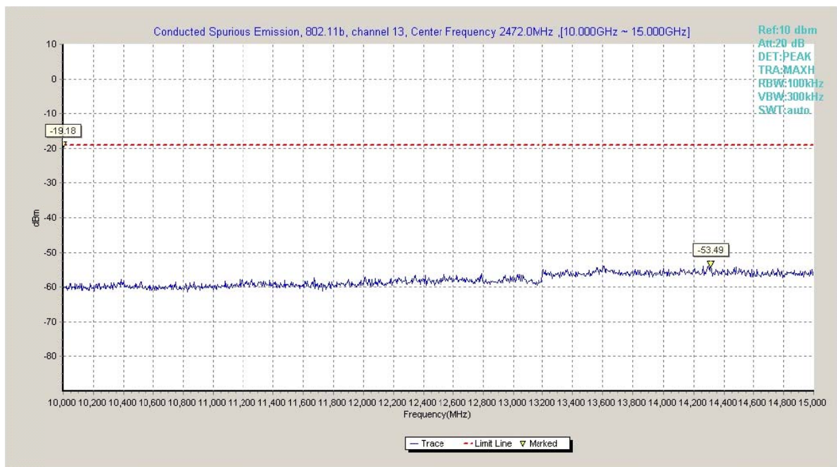
Fig.A.6.1.38 Transmitter Spurious Emission - Conducted (802.11b, Ch13, 10 GHz-15 GHz)
