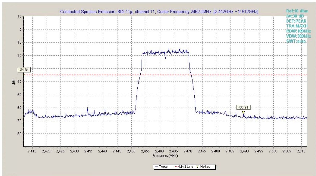
Fig.A.6.1.57 Transmitter Spurious Emission - Conducted (802.11g, Ch11, Center Frequency)
