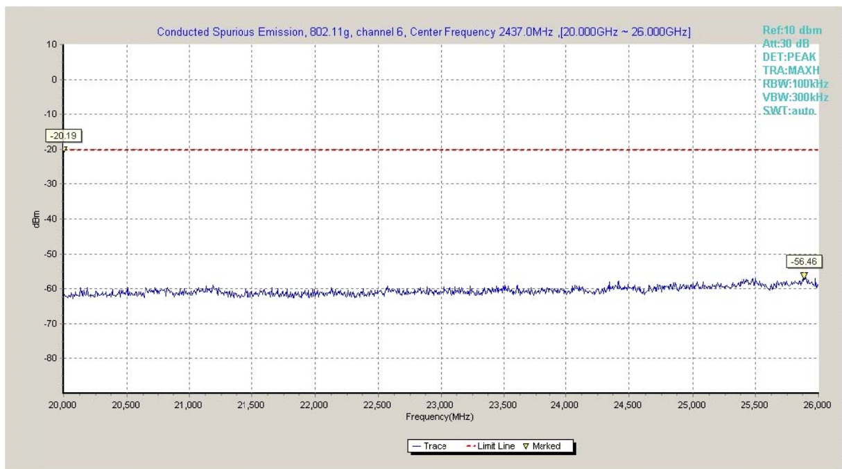
Fig.A.6.1.56 Transmitter Spurious Emission - Conducted (802.11g, Ch6, 20 GHz-26 GHz)
