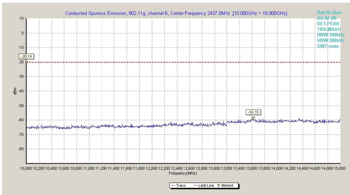
Fig.A.6.1.54 Transmitter Spurious Emission - Conducted (802.11g, Ch6, 10 GHz-15 GHz)
