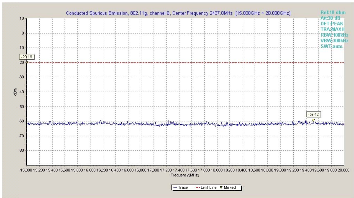
Fig.A.6.1.55 Transmitter Spurious Emission - Conducted (802.11g, Ch6, 15 GHz-20 GHz)
