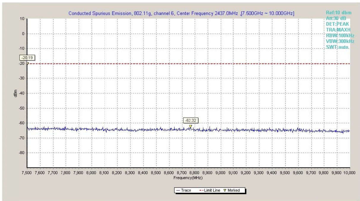
Fig.A.6.1.53 Transmitter Spurious Emission - Conducted (802.11g, Ch6, 7.5 GHz-10 GHz)
