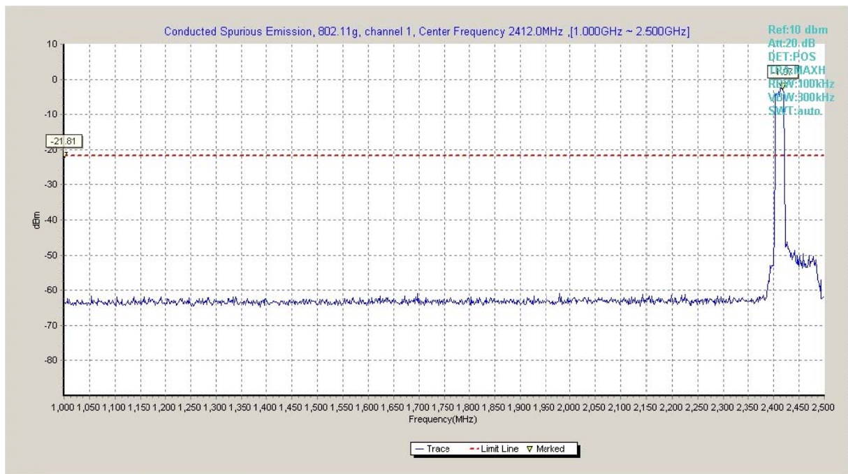
Fig.A.6.1.43 Transmitter Spurious Emission - Conducted (802.11g, Ch1, 1 GHz-2.5 GHz)
