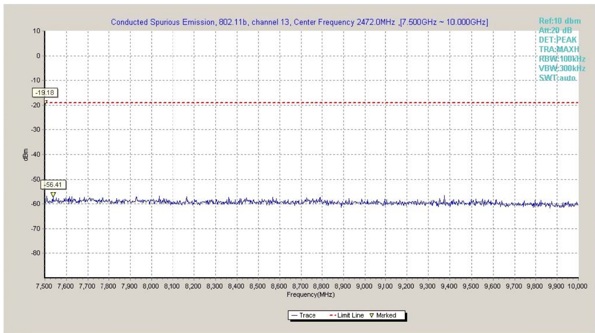
Fig.A.6.1.37 Transmitter Spurious Emission - Conducted (802.11b, Ch13, 7.5 GHz-10 GHz)
