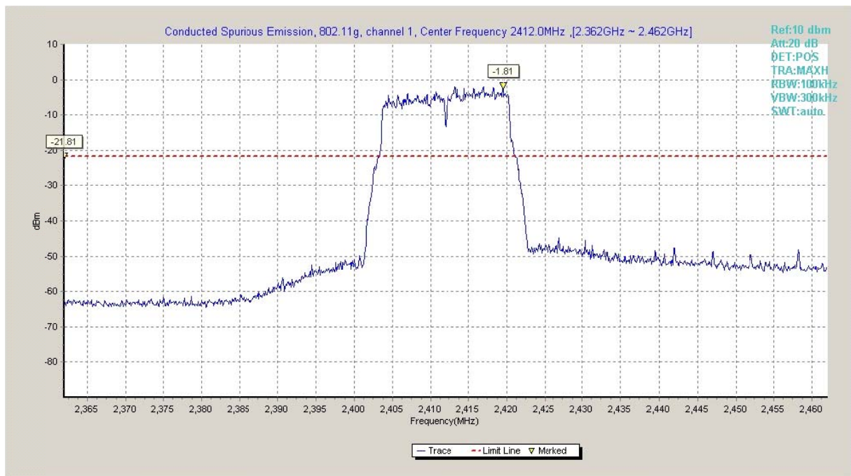
Fig.A.6.1.41 Transmitter Spurious Emission - Conducted (802.11g, Ch1, Center Frequency)
