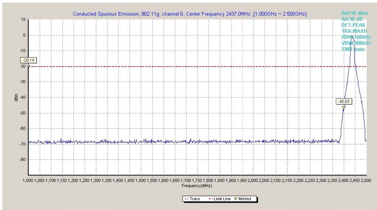
Fig.A.6.1.51 Transmitter Spurious Emission - Conducted (802.11g, Ch6, 1 GHz-2.5 GHz)
