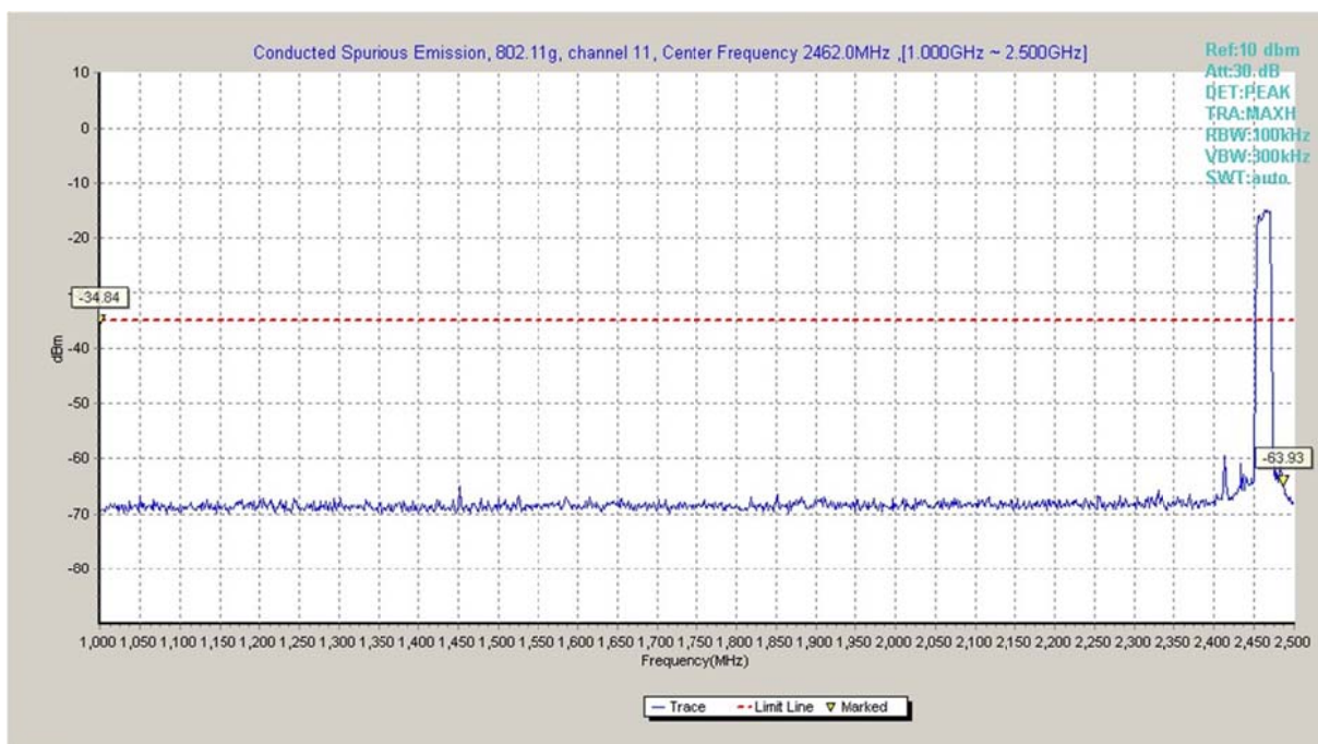
Fig.A.6.1.59 Transmitter Spurious Emission - Conducted (802.11g, Ch11, 1 GHz-2.5 GHz)
