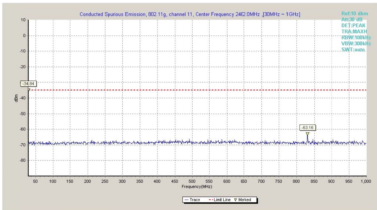
Fig.A.6.1.58 Transmitter Spurious Emission - Conducted (802.11g, Ch11, 30 MHz-1 GHz)
