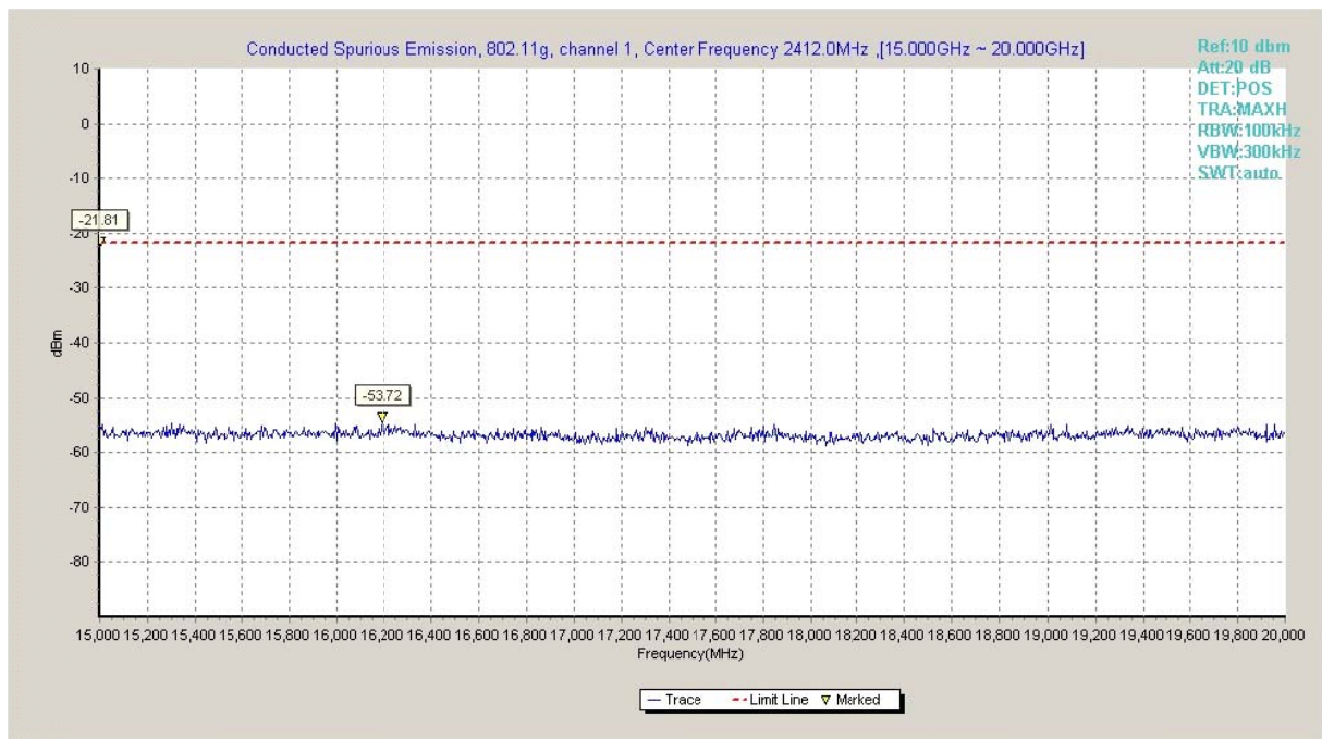
Fig.A.6.1.47 Transmitter Spurious Emission - Conducted (802.11g, Ch1, 15 GHz-20 GHz)
