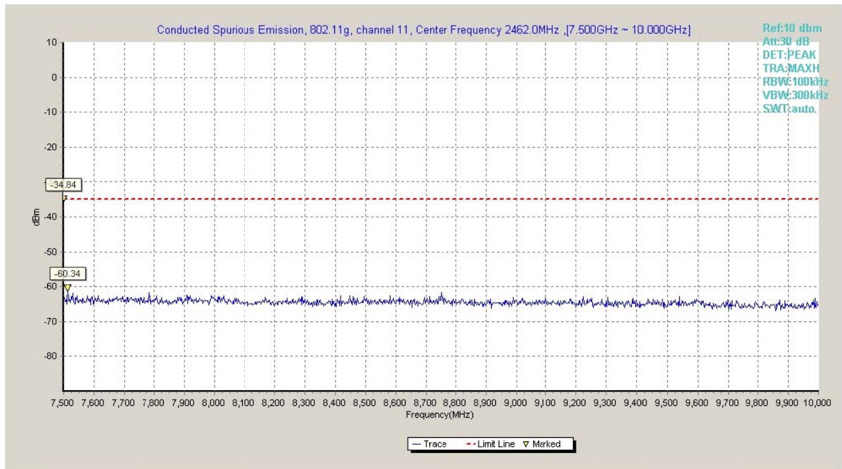
Fig.A.6.1.61 Transmitter Spurious Emission - Conducted (802.11g, Ch11, 7.5 GHz-10 GHz)
