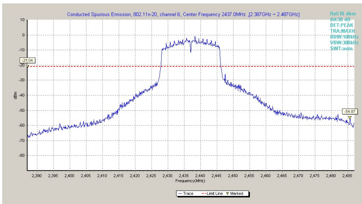
Fig.A.6.1.89 Transmitter Spurious Emission - Conducted (802.11n-HT20, Ch6, Center Frequency)
