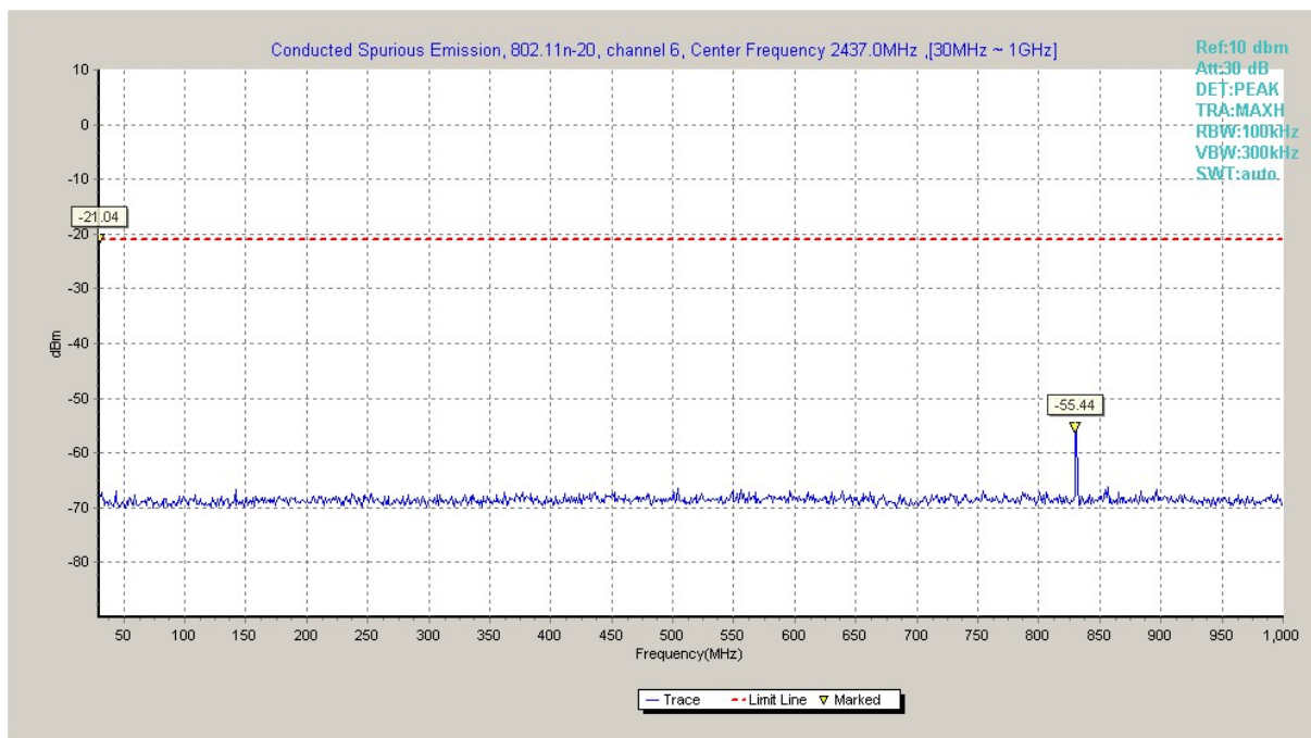
Fig.A.6.1.90 Transmitter Spurious Emission - Conducted (802.11n-HT20, Ch6, 30 MHz-1 GHz)
