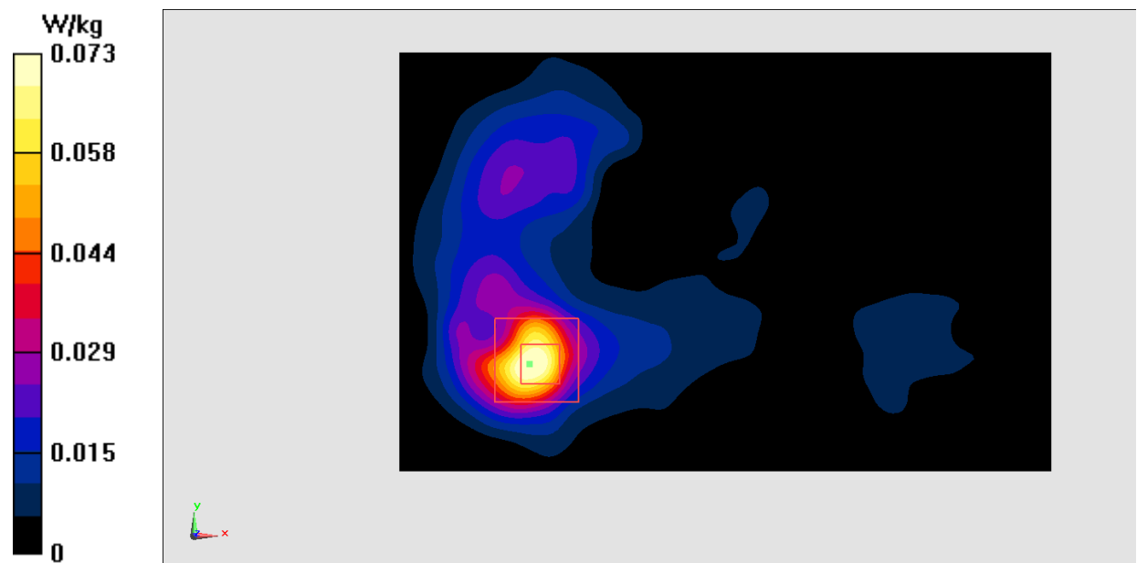
Fig.10 2450 MHz
