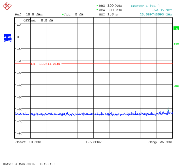
Fig.12. Transmitter Spurious Emission - Conducted: GFSK, 2440 MHz, 10GHz – 26GHz
