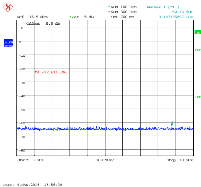
Fig.11. Transmitter Spurious Emission - Conducted: GFSK, 2440 MHz, 3GHz – 10GHz
