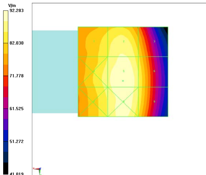
Fig B.3 HAC RF E-Field GSM 850 Low
