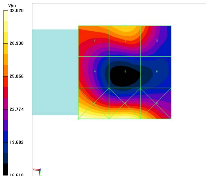
Fig B.4 HAC RF E-Field GSM 1900 High
