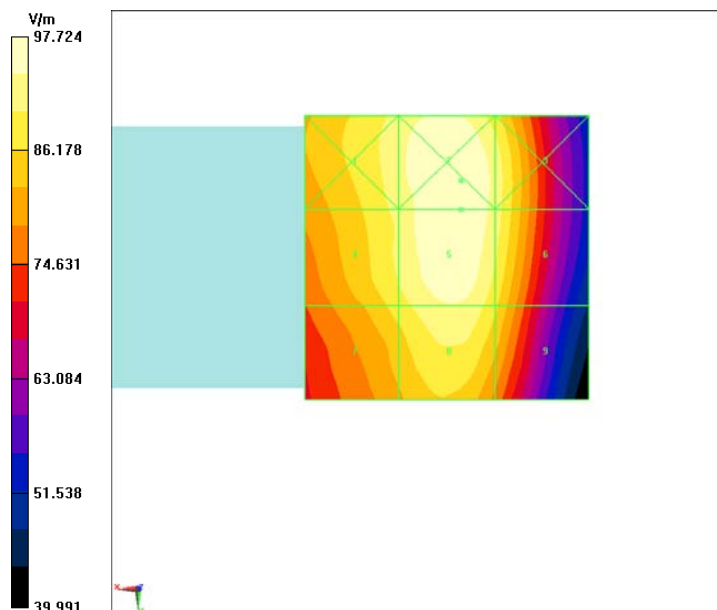
Fig B.2 HAC RF E-Field GSM 850 Middle
