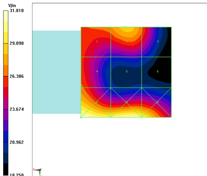
Fig B.5 HAC RF E-Field GSM 1900 Middle
