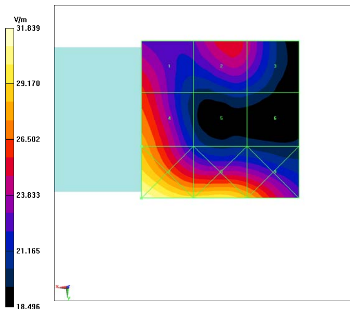
Fig B.6 HAC RF E-Field GSM 1900 Low
