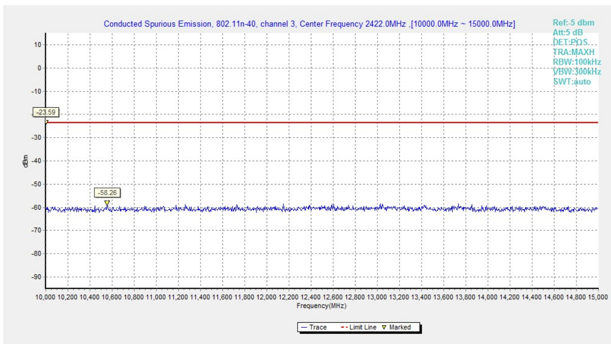
Fig.A.6.1.78 Transmitter Spurious Emission - Conducted (802.11n-HT40, Ch3, 10 GHz-15 GHz)
