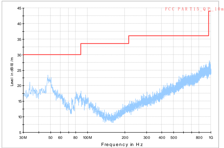
Normal RE_30MHz-1GHz_10m_FP52
