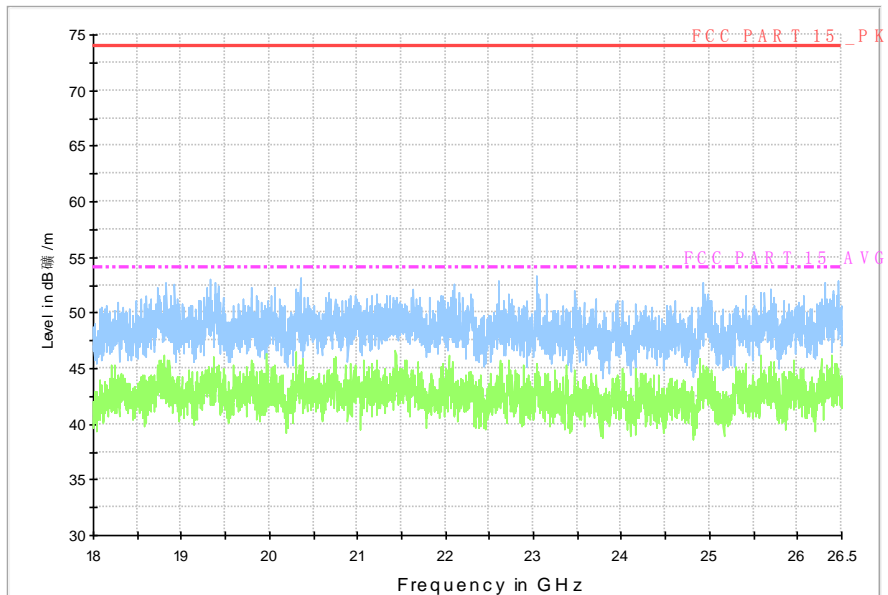
Normal RE_18G-26.5GHz
