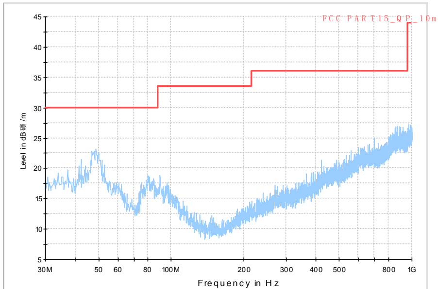
Normal RE_30MHz-1GHz_10m_FP52
