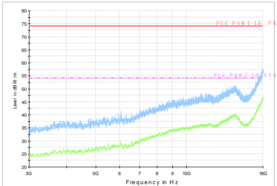
Normal RE_3G-18GHz_filter
