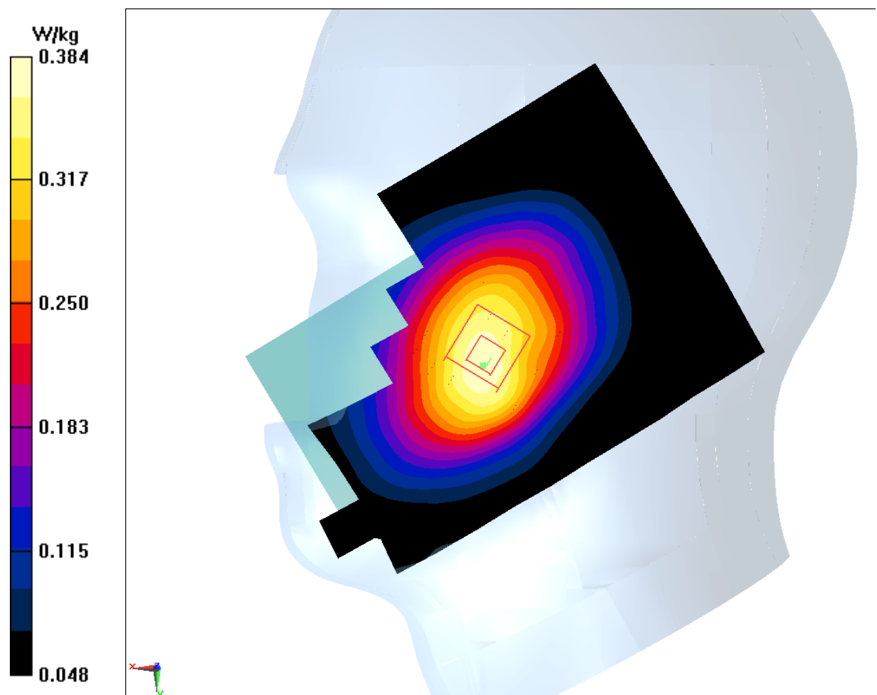
Fig.1 850MHz
