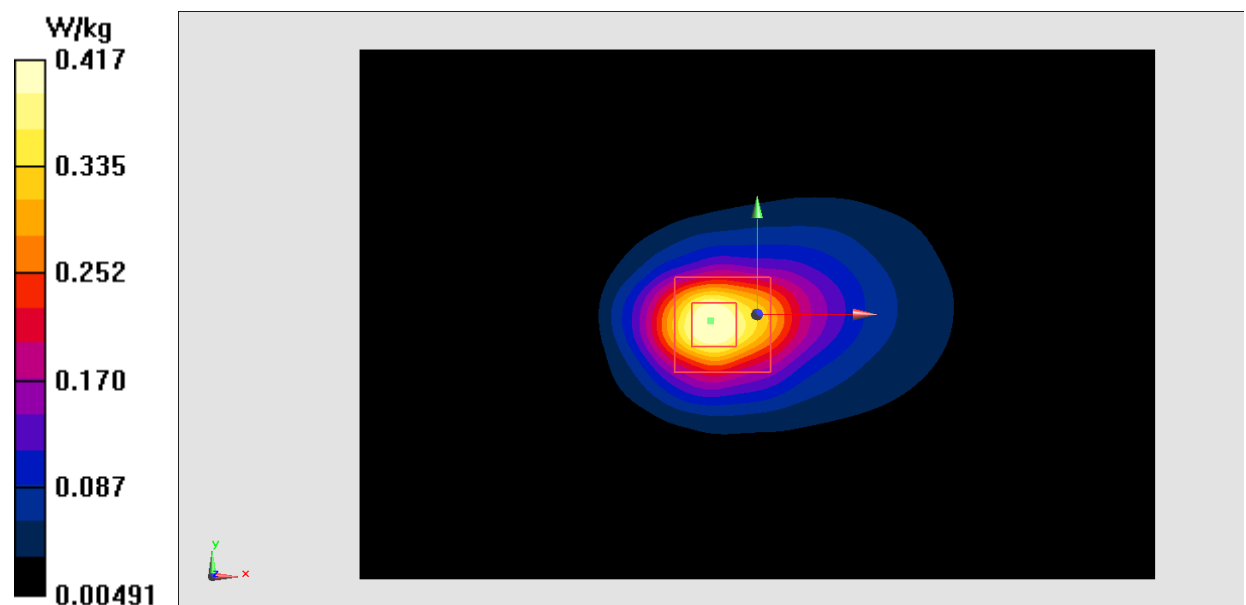
Fig.4 1900 MHz
