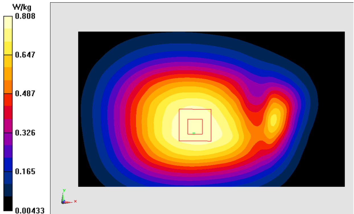
Fig.2 850 MHz
