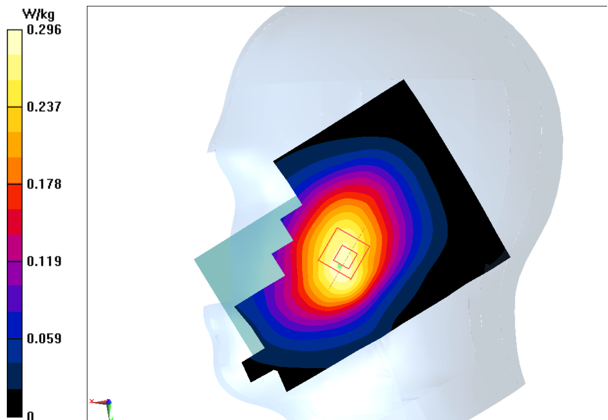
Fig.1 850MHz
