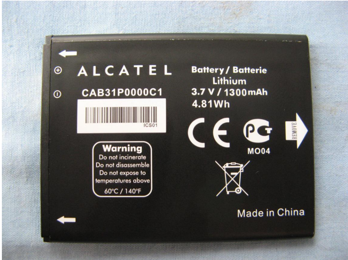
Battery AE12
