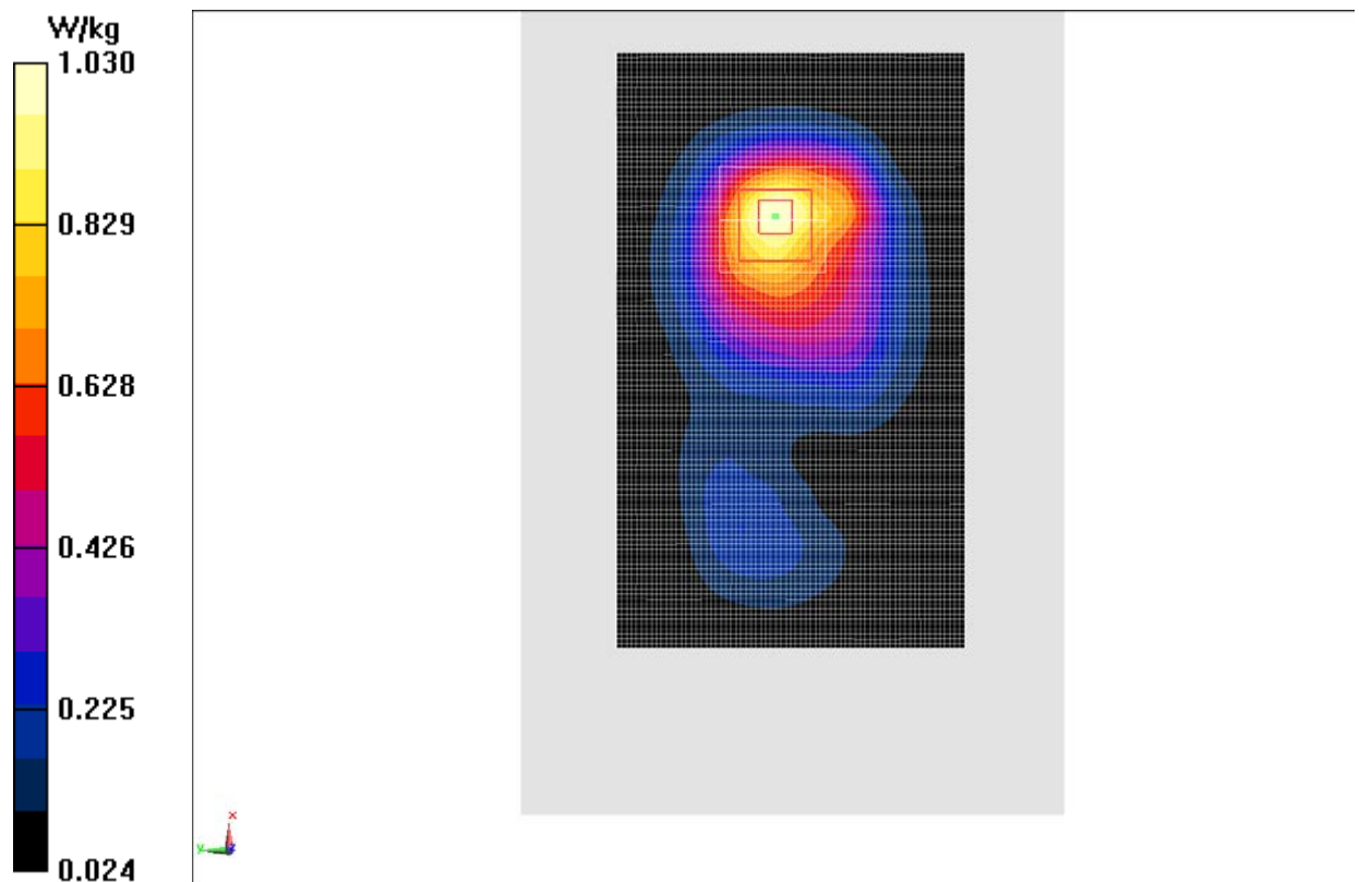
Fig.4 1900 MHz
