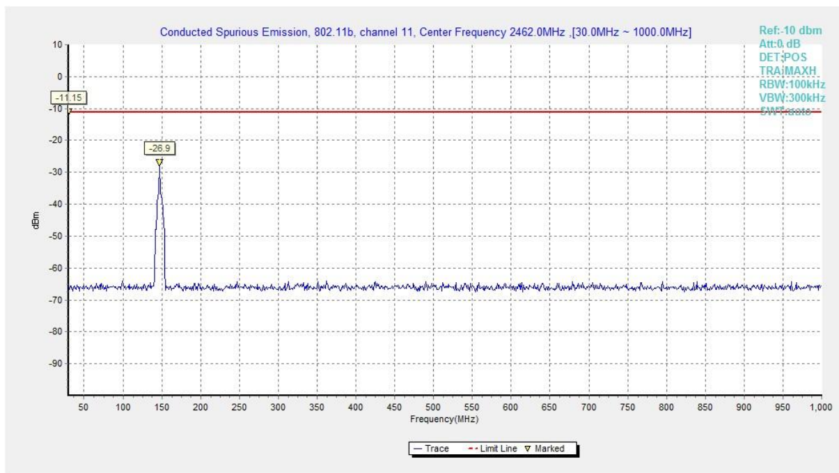
Fig.A.6.1.18 Transmitter Spurious Emission - Conducted (802.11b, Ch11, 30 MHz-1 GHz)
