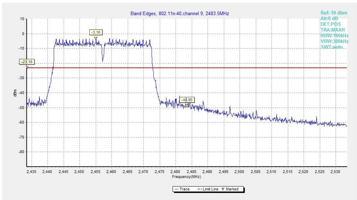
Fig.A.5.8 Band Edges (802.11n-HT40, Ch 9)
