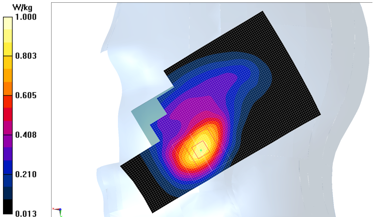
Fig.I.7 WCDMA 1900 CH9538
