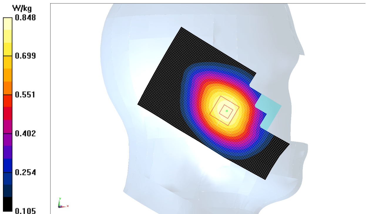
Fig.I.1 850MHz CH251
