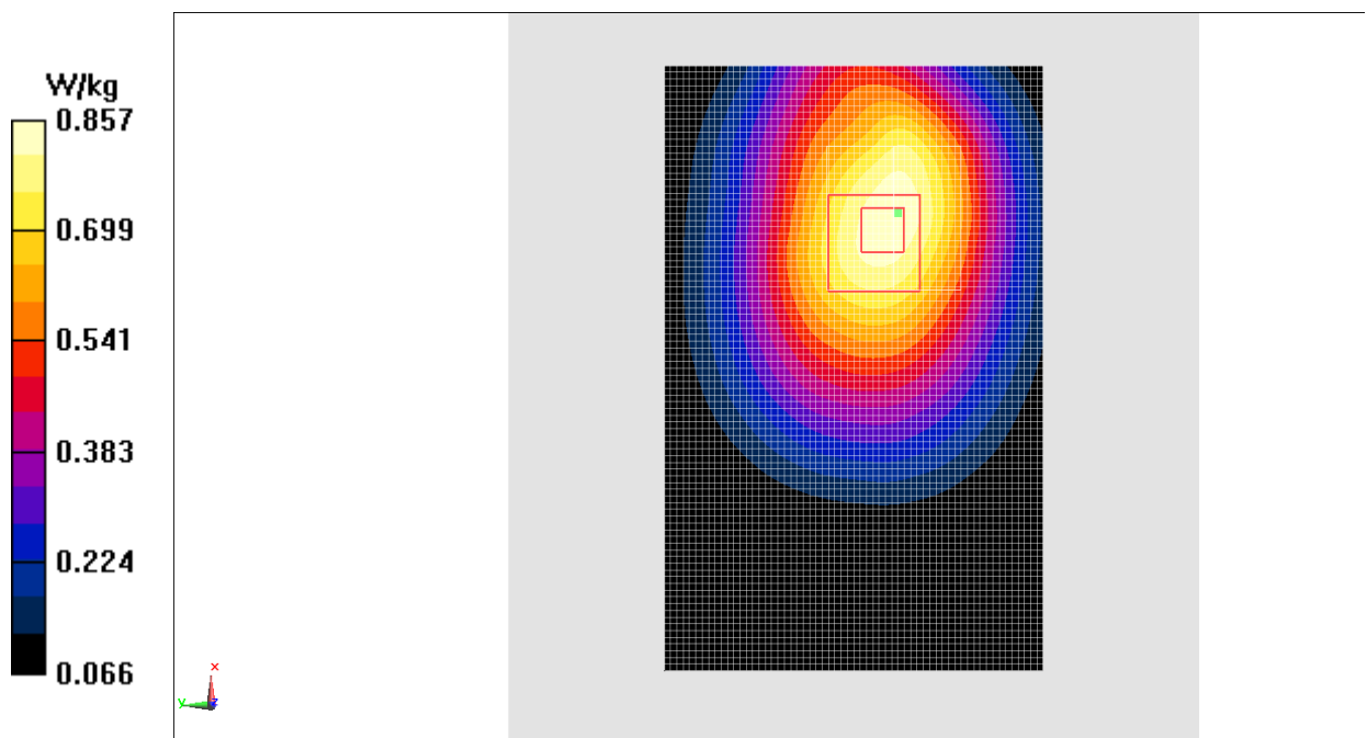
Fig.I.2 850 MHz CH251
