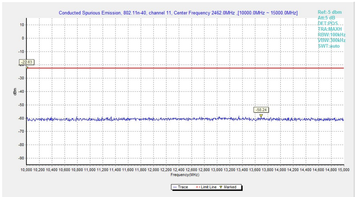
Fig.A.6.1.150 Transmitter Spurious Emission - Conducted (802.11n-HT40, Ch11, 10 GHz-15 GHz)
