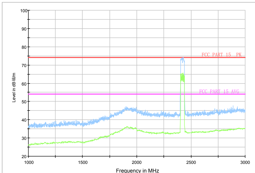
Fig.A.6.2.51 Transmitter Spurious Emission - Radiated (802.11n-HT40, ch3, 1 GHz-3 GHz)
