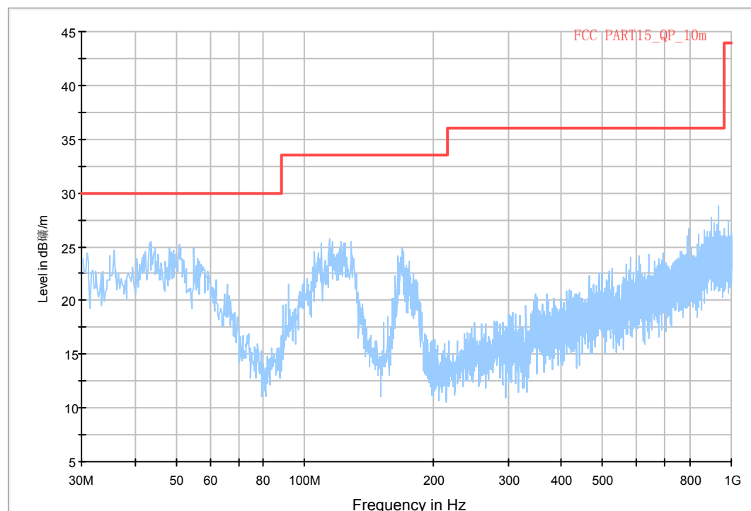
Fig.A.6.2.53 Transmitter Spurious Emission - Radiated (802.11n-HT40, Ch6, 30 MHz-1 GHz)
