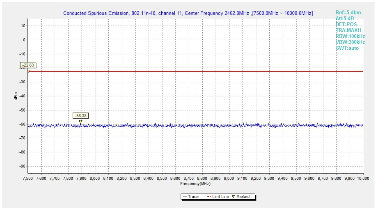
Fig.A.6.1.149 Transmitter Spurious Emission - Conducted (802.11n-HT40, Ch11, 7.5 GHz-10 GHz)
