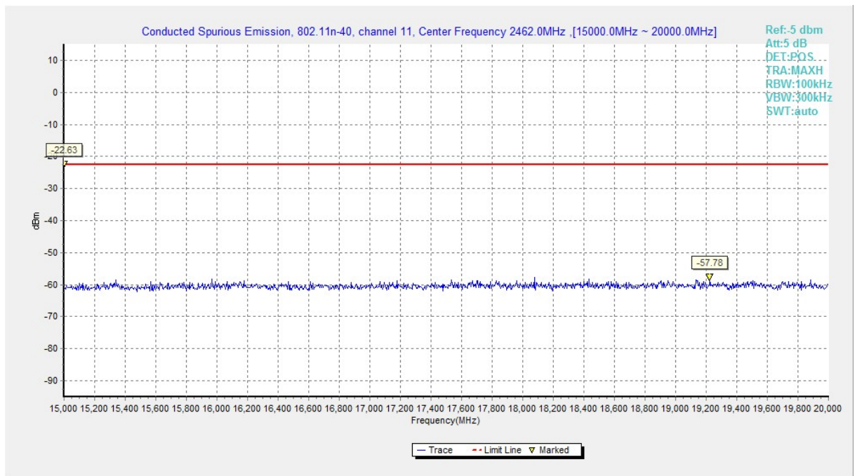
Fig.A.6.1.151 Transmitter Spurious Emission - Conducted (802.11n-HT40, Ch11, 15 GHz-20 GHz)
