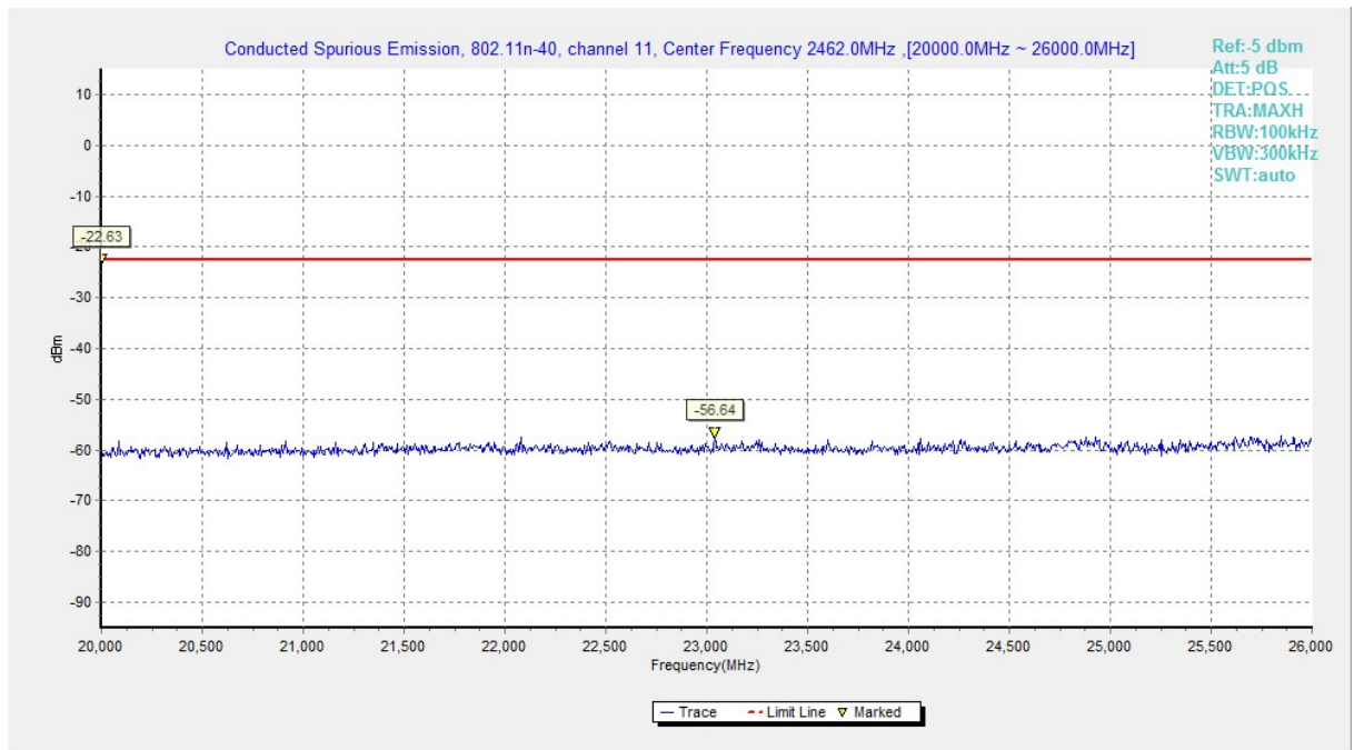
Fig.A.6.1.152 Transmitter Spurious Emission - Conducted (802.11n-HT40, Ch11, 20 GHz-26 GHz)
