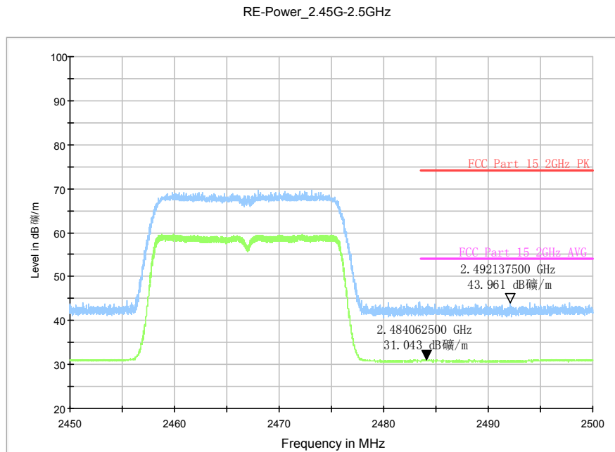
Fig.A.6.2.44 Transmitter Spurious Emission - Radiated (Power): 802.11n-HT20, ch12, 2.45 GHz - 2.50GHz
