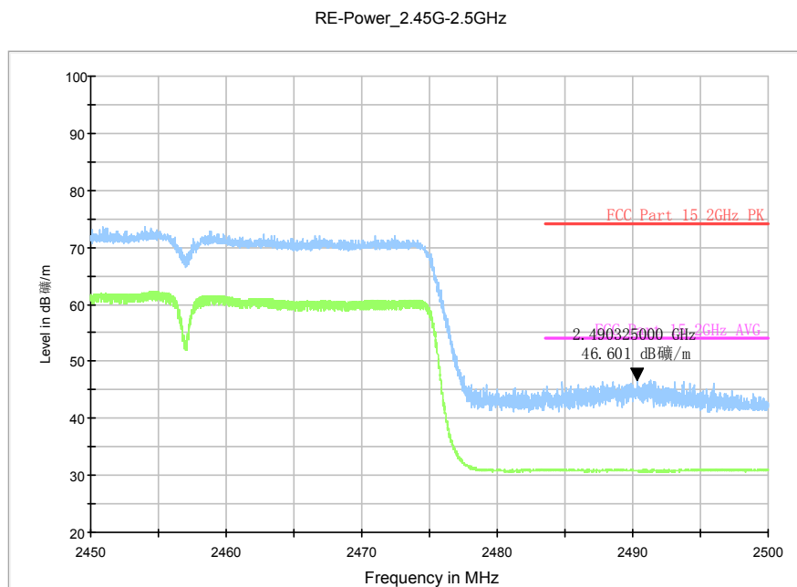
Fig.A.6.2.60 Transmitter Spurious Emission - Radiated (Power): 802.11n-HT40, ch10, 2.45 GHz - 2.50GHz
