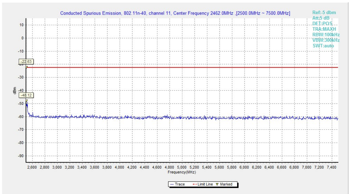
Fig.A.6.1.148 Transmitter Spurious Emission - Conducted (802.11n-HT40, Ch11, 2.5 GHz-7.5 GHz)
