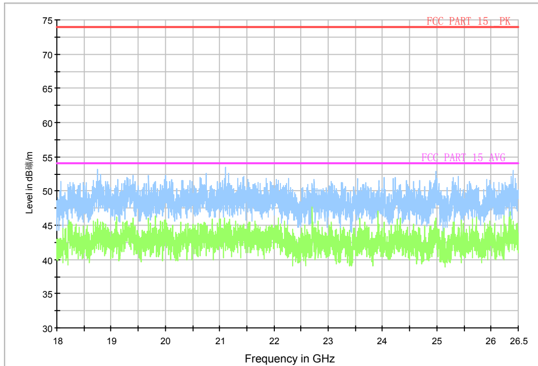
Fig.A.6.2.56 Transmitter Spurious Emission - Radiated (802.11n-HT40, Ch6, 18GHz - 26.5GHz)
