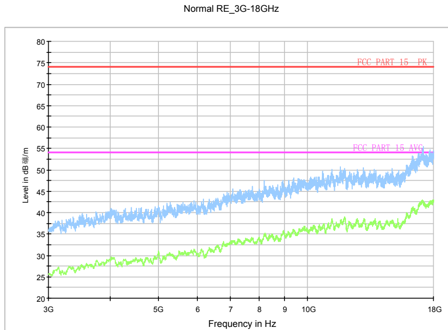
Fig.A.6.2.62 Transmitter Spurious Emission - Radiated (802.11n-HT40, Ch10, 3 GHz-18 GHz)
