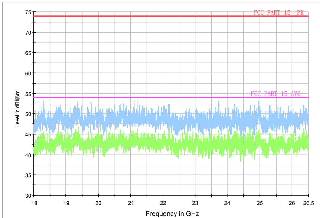
Fig.A.6.2.40 Transmitter Spurious Emission - Radiated (802.11n-HT20, Ch6, 18GHz - 26.5GHz)
