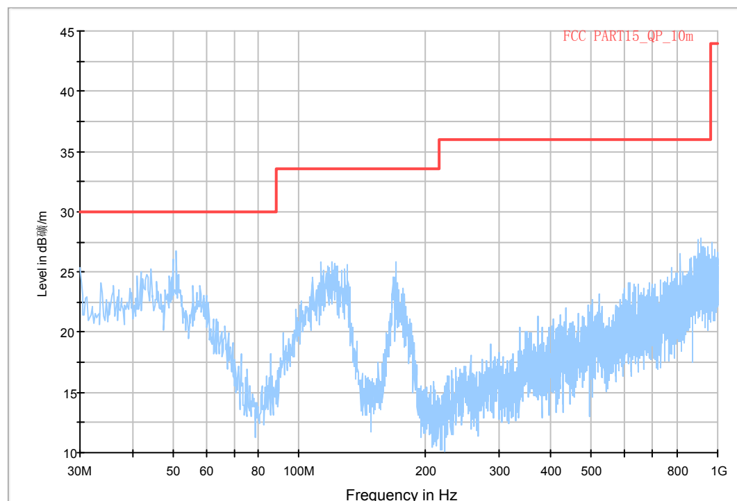
Fig.A.6.2.37 Transmitter Spurious Emission - Radiated (802.11n-HT20, Ch6, 30 MHz-1 GHz)
