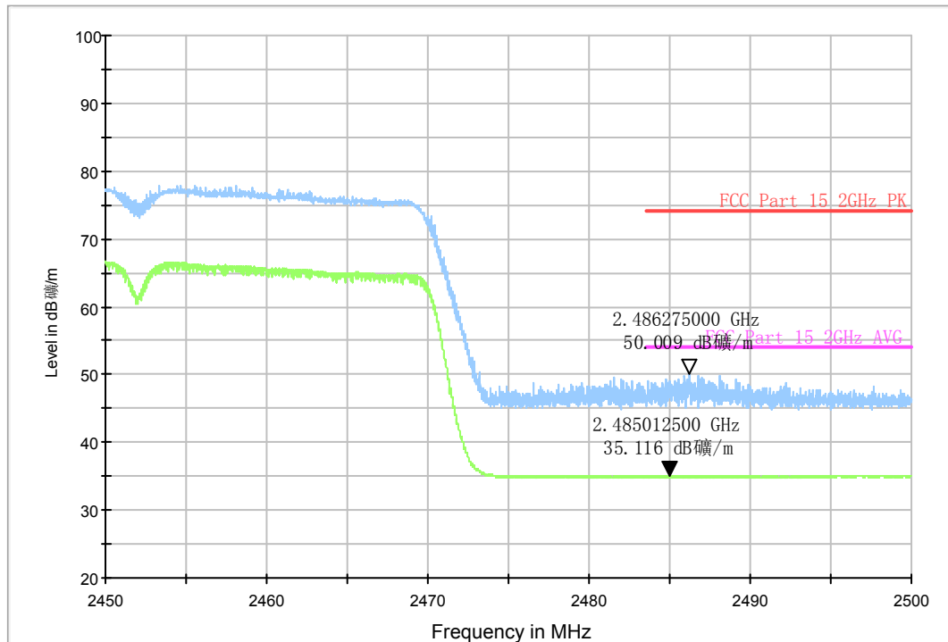
Fig.A.6.2.57 Transmitter Spurious Emission - Radiated (Power): 802.11n-HT40, ch9, 2.45 GHz - 2.50GHz
