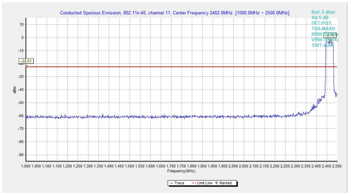
Fig.A.6.1.147 Transmitter Spurious Emission - Conducted (802.11n-HT40, Ch11, 1 GHz-2.5 GHz)
