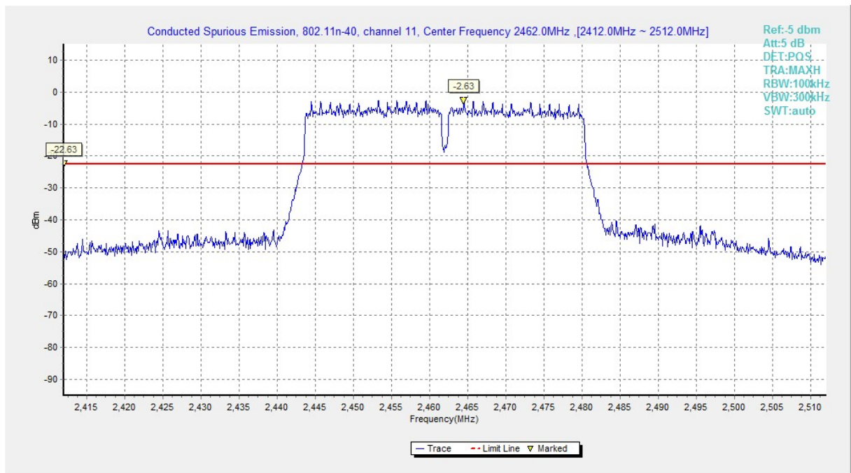
Fig.A.6.1.145 Transmitter Spurious Emission - Conducted (802.11n-HT40, Ch11, Center Frequency)
