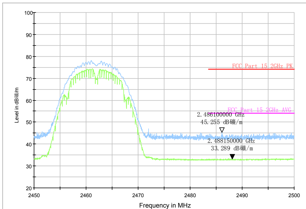
Fig.A.6.2.9 Transmitter Spurious Emission - Radiated (Power): 802.11b, ch11, 2.45
