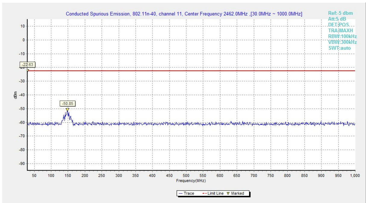
Fig.A.6.1.146 Transmitter Spurious Emission - Conducted (802.11n-HT40, Ch11, 30 MHz-1 GHz)
