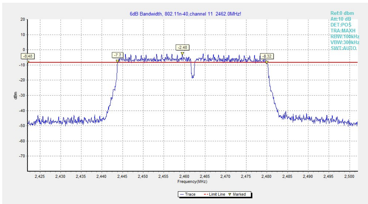
Fig.A.4.19 Occupied 6dB Bandwidth (802.11n-HT40, Ch 11)
