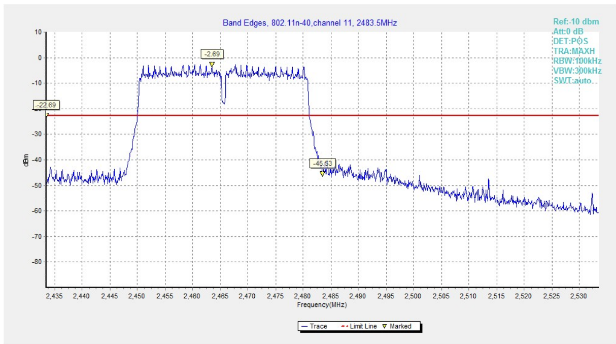
Fig.A.5.15 Band Edges (802.11n-HT40, Ch 11)
