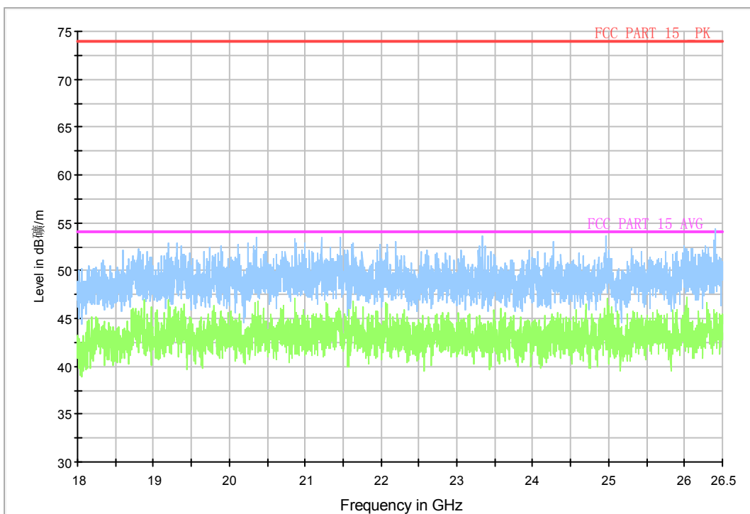
Fig.78. Radiated emission: \pi/4 DQPSK, 18 GHz - 26 GHz
