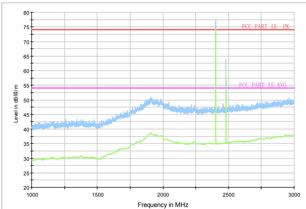
Fig.79. Radiated emission: 8DPSK, Channel 0, 1 GHz - 3 GHz
