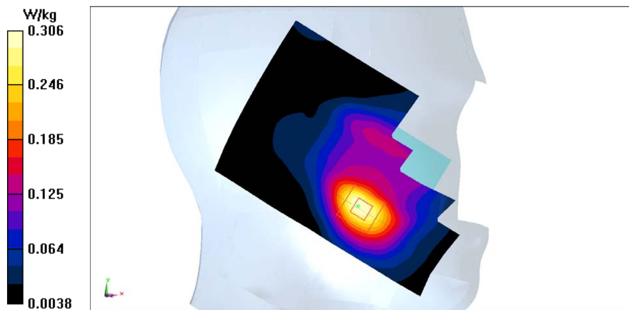
Fig.3 1900 MHz Head
