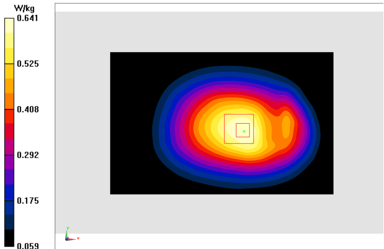
Fig.2 850 MHz Body
