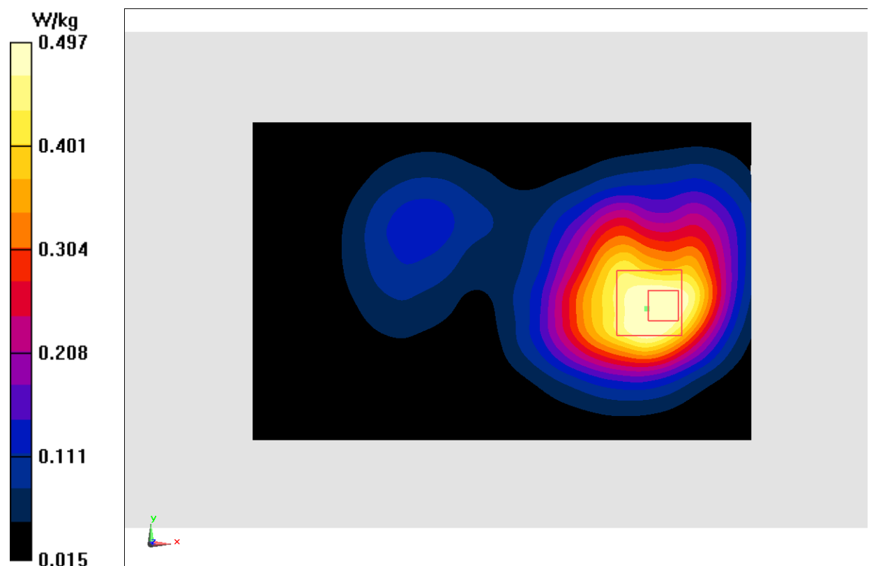
Fig.4 1900 MHz Body
