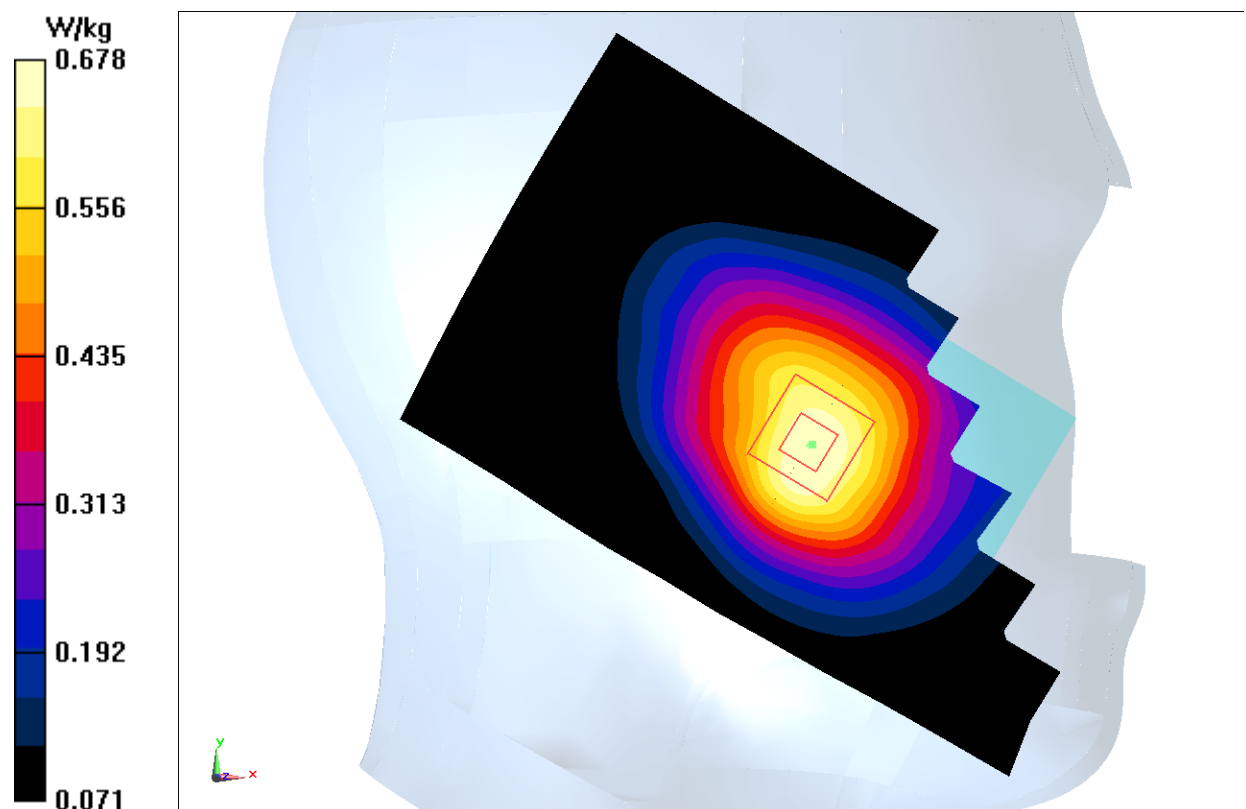
Fig.1 850MHz Head
