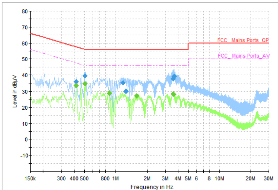
Fig. 95 AC Power line Conducted Emission (Traffic)
