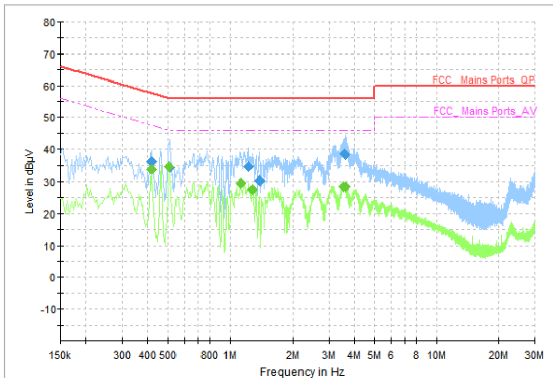
Fig. 96 AC Power line Conducted Emission (Idle)
