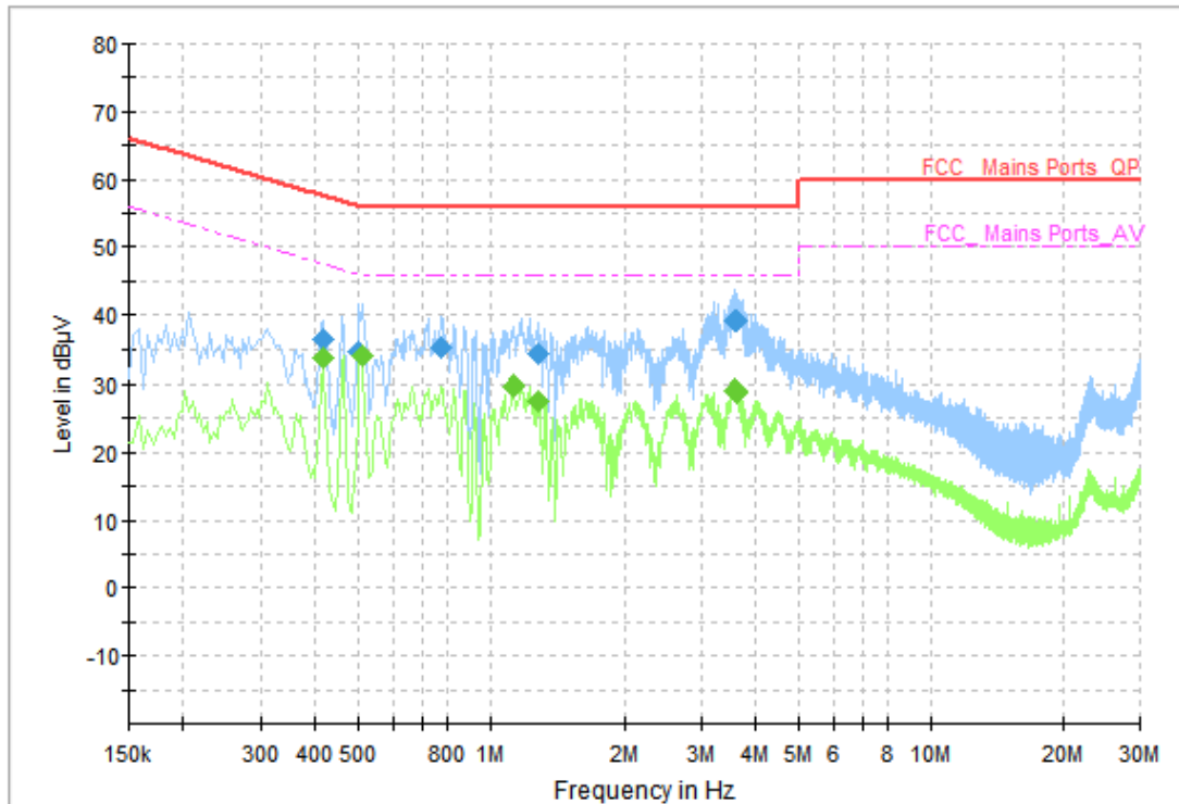
Fig.33 AC Power line Conducted Emission (Traffic, AE2-2, 120V), 1M
