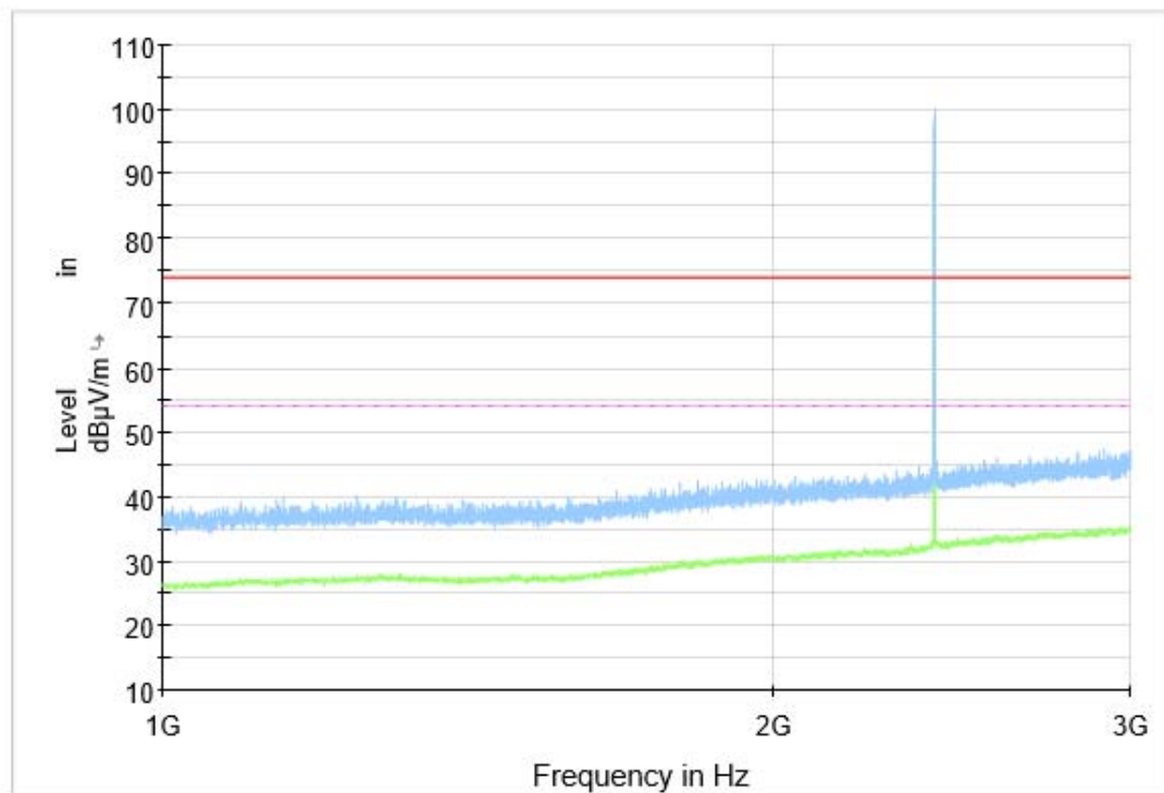
Fig.20 Radiated Spurious Emission (Ch0, 1 GHz - 3 GHz), 1M
