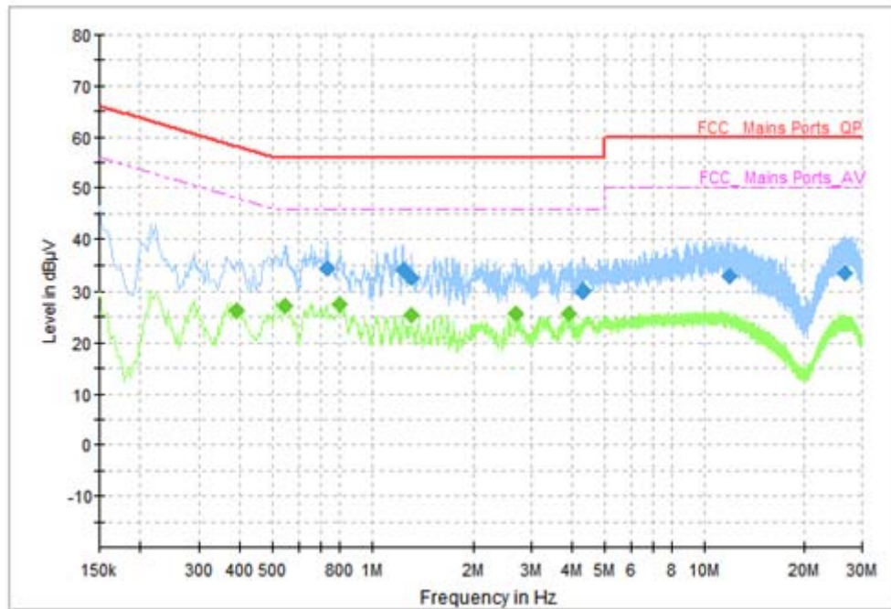
Fig.32 AC Power line Conducted Emission (Idle, AE2-1, 120V), 1M
