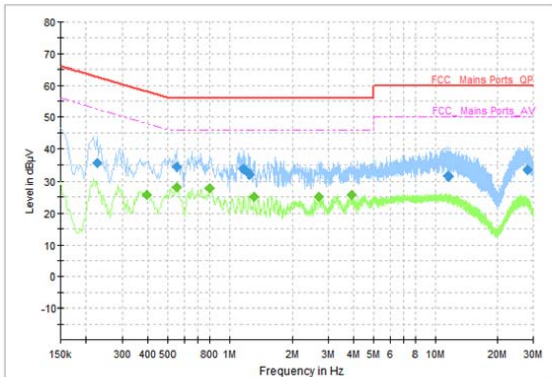
Fig.31 AC Power line Conducted Emission (Traffic, AE2-1, 120V), 1M
