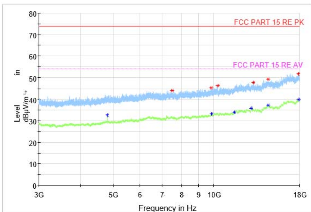
Fig.21 Radiated Spurious Emission (Ch0, 3 GHz - 18 GHz), 1M
