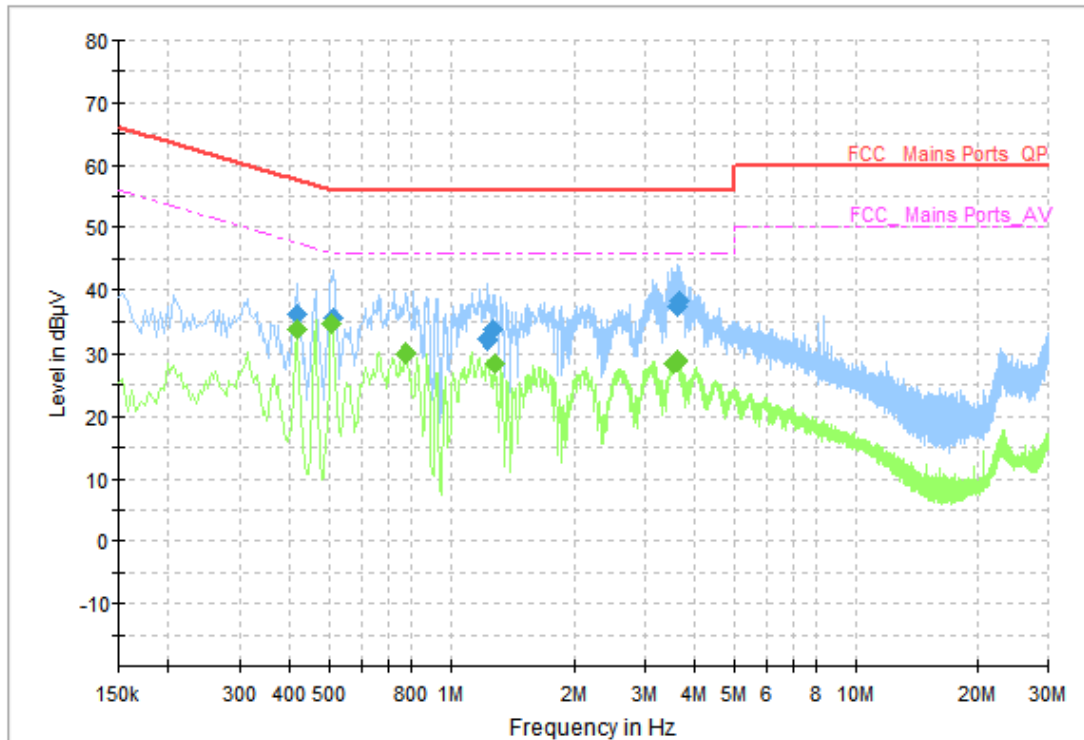
Fig.34 AC Power line Conducted Emission (Idle, AE2-2, 120V), 1M
