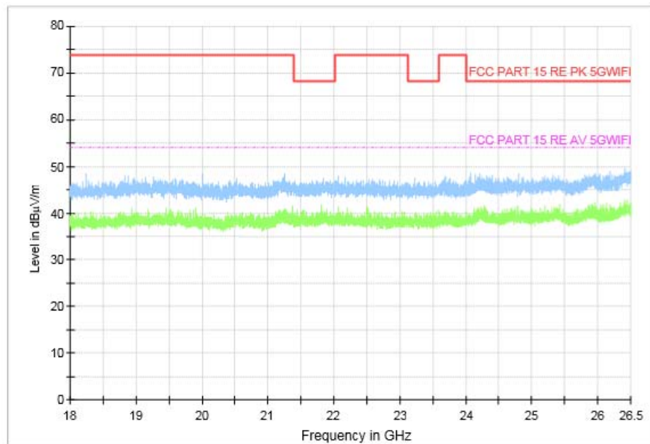
Fig. 103 Transmitter Spurious Emission (All channel, 18GHz~26.5GHz)
