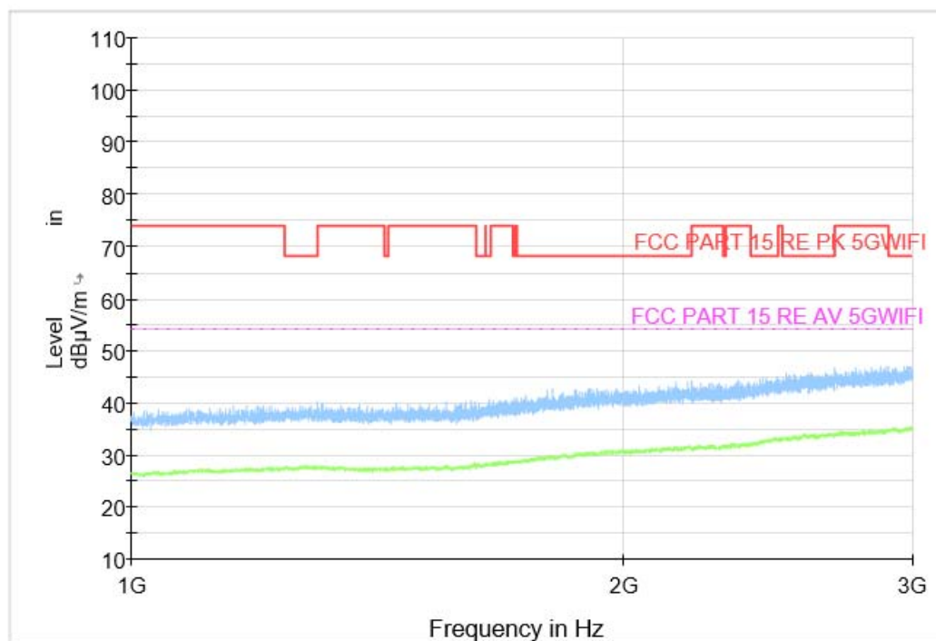
Fig. 102 Transmitter Spurious Emission (All channel, 1GHz ~3GHz)
