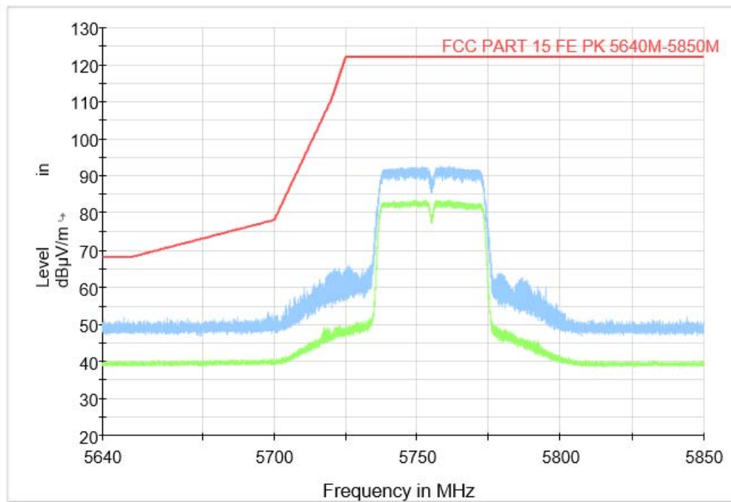
Fig. 51 Band Edges (802.11n-HT40, CH151 5755MHz)
