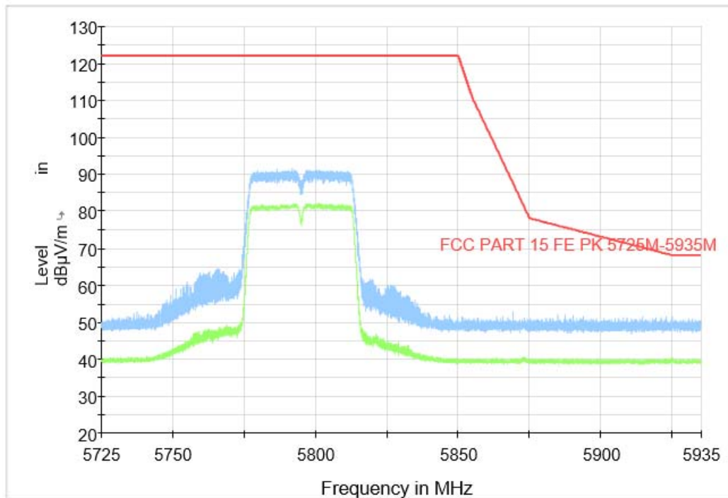
Fig. 52 Band Edges (802.11n-HT40, CH159 5795MHz)
