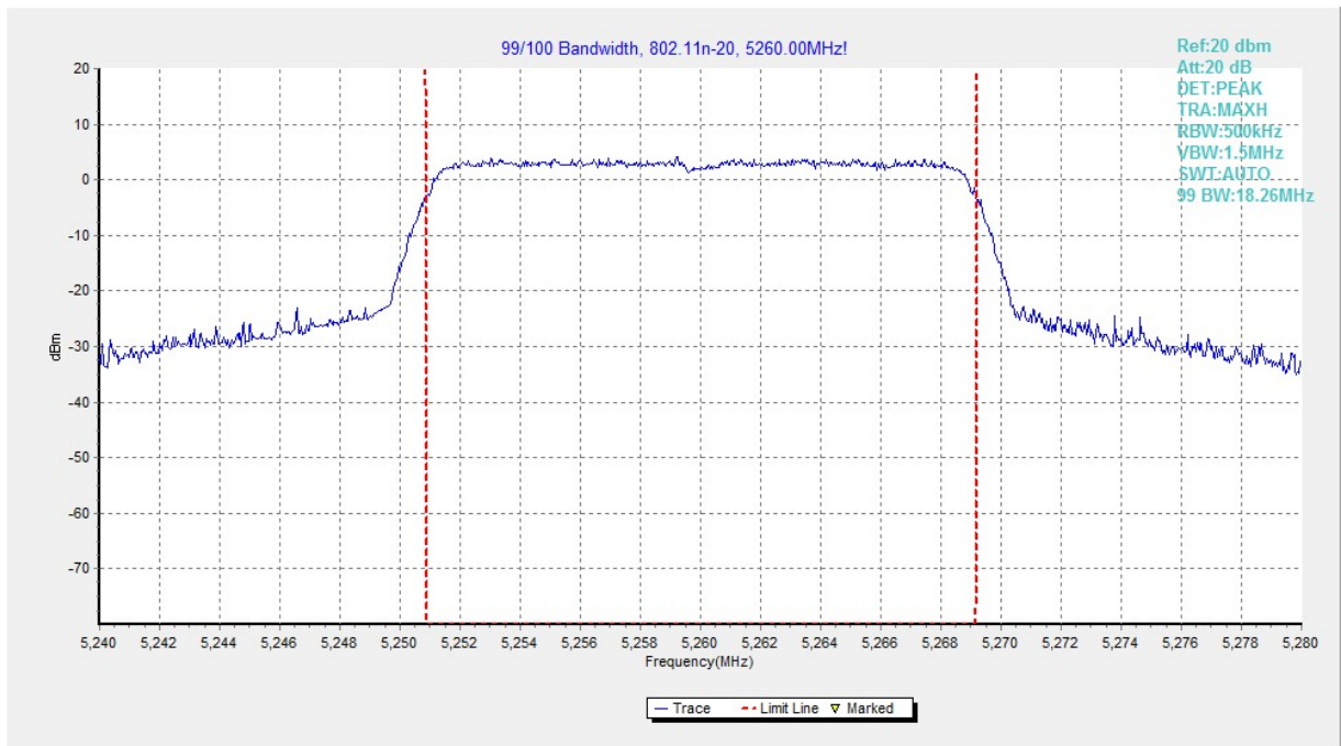
Fig. 34 99% Occupied Bandwidth (802.11n-HT20, 5260MHz)
