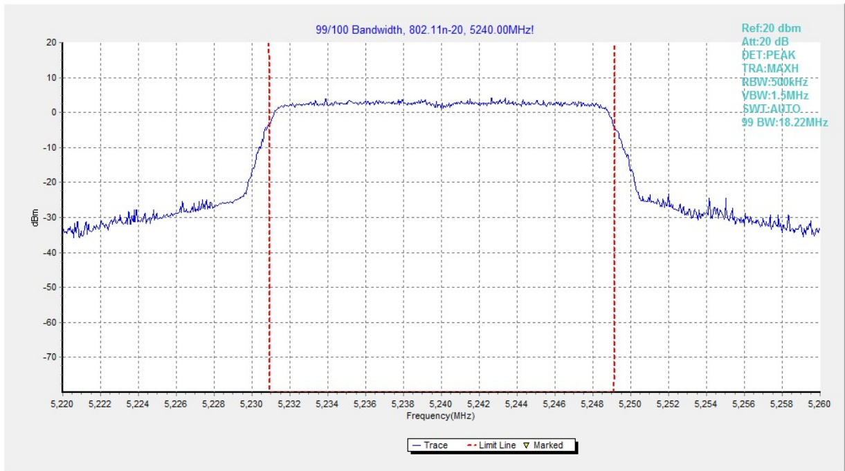
Fig. 33 99% Occupied Bandwidth (802.11n-HT20, 5240MHz)
