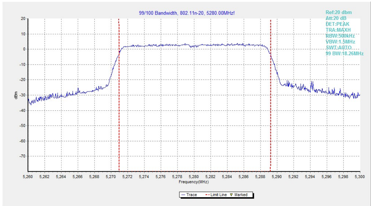
Fig. 35 99% Occupied Bandwidth (802.11n-HT20, 5280MHz)
