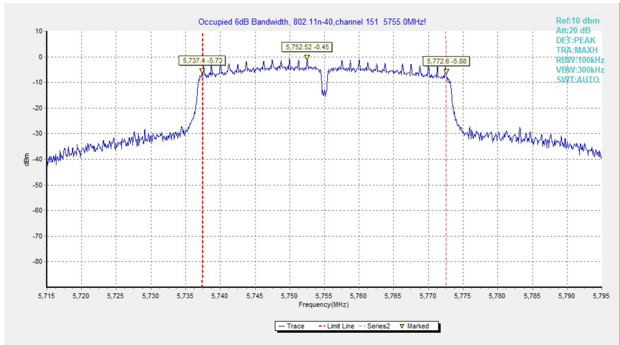
Fig. 23 Occupied 6dB Bandwidth (802.11n-HT40, 5755MHz)
