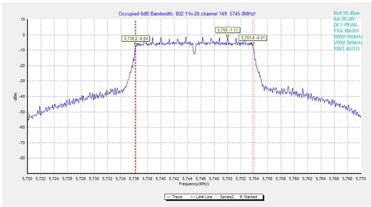
Fig. 20 Occupied 6dB Bandwidth (802.11n-HT20, 5745MHz)
