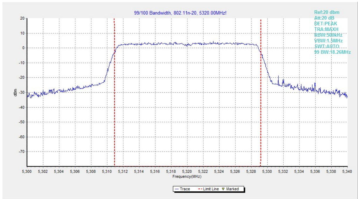
Fig. 36 99% Occupied Bandwidth (802.11n-HT20, 5320MHz)
