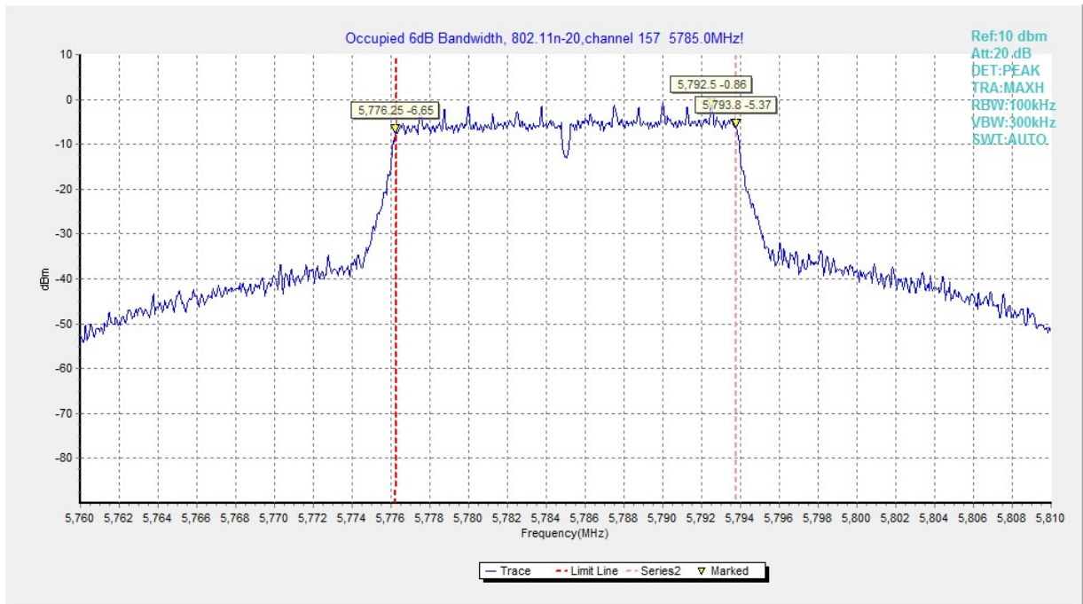
Fig. 21 Occupied 6dB Bandwidth (802.11n-HT20, 5785MHz)
