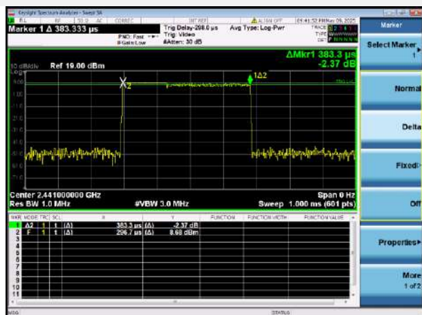
8-DPSK 3DH1
