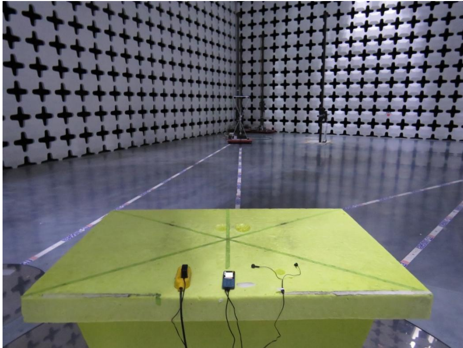
RE 30MHz-1GHz
