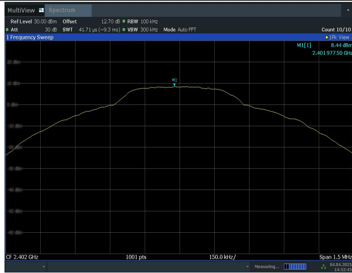
DH5_2402_0~Reference
