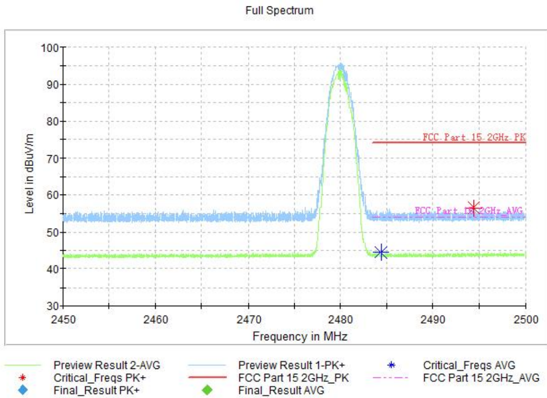
Fig.6. Frequency Band Edges: 8DPSK, Channel 78, 2.45 GHz - 2.50GHz
