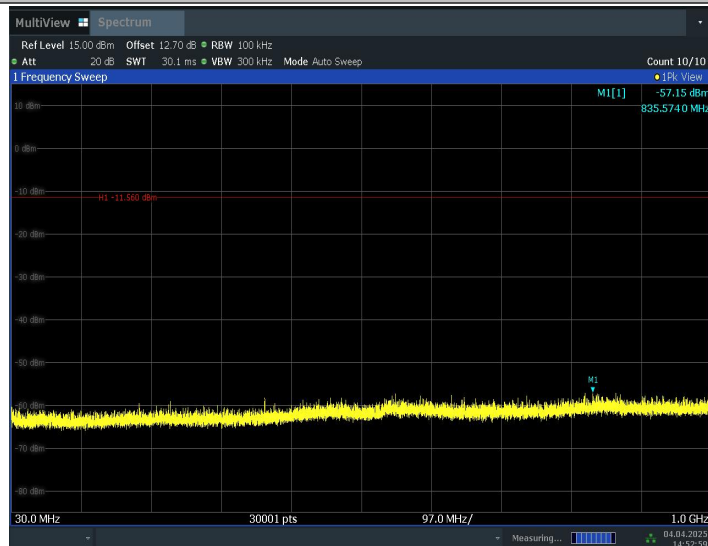
DH5_2402_30~1000
