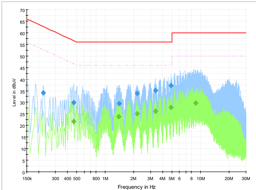
Fig. 13 AC Powerline Conducted Emission-802.11a CH149
