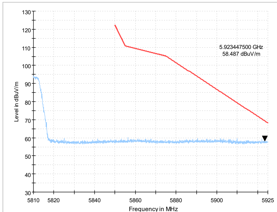
Fig. 6 Band Edges (802.11n-HT40 Ch159, 5795MHz)
