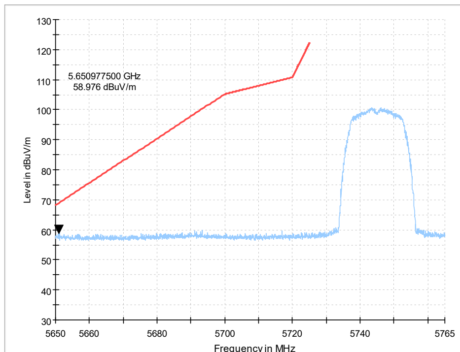
Fig. 1 Band Edges (802.11a Ch149,5745MHz)
