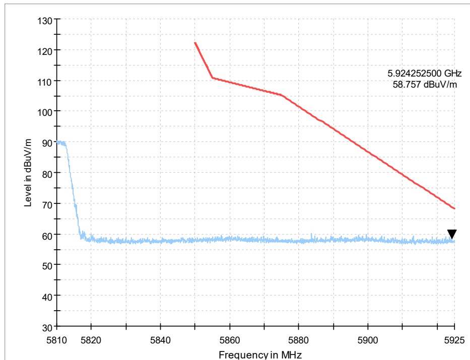
Fig. 12 Band Edges (802.11ac-HT80, 5775MHz)
