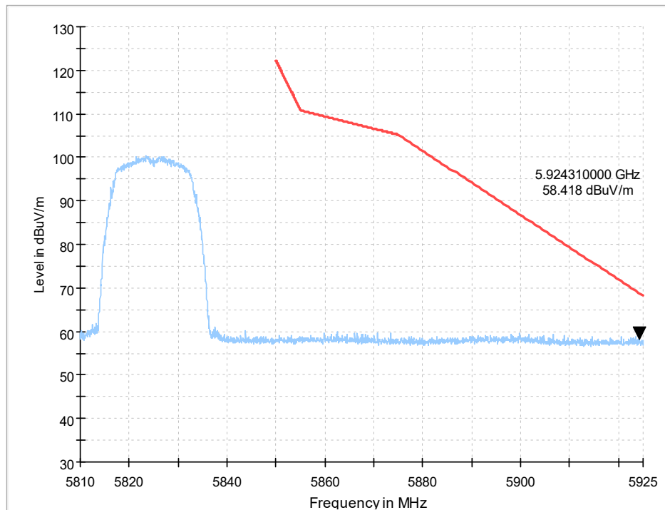
Fig. 2 Band Edges (802.11a Ch165, 5825MHz)
