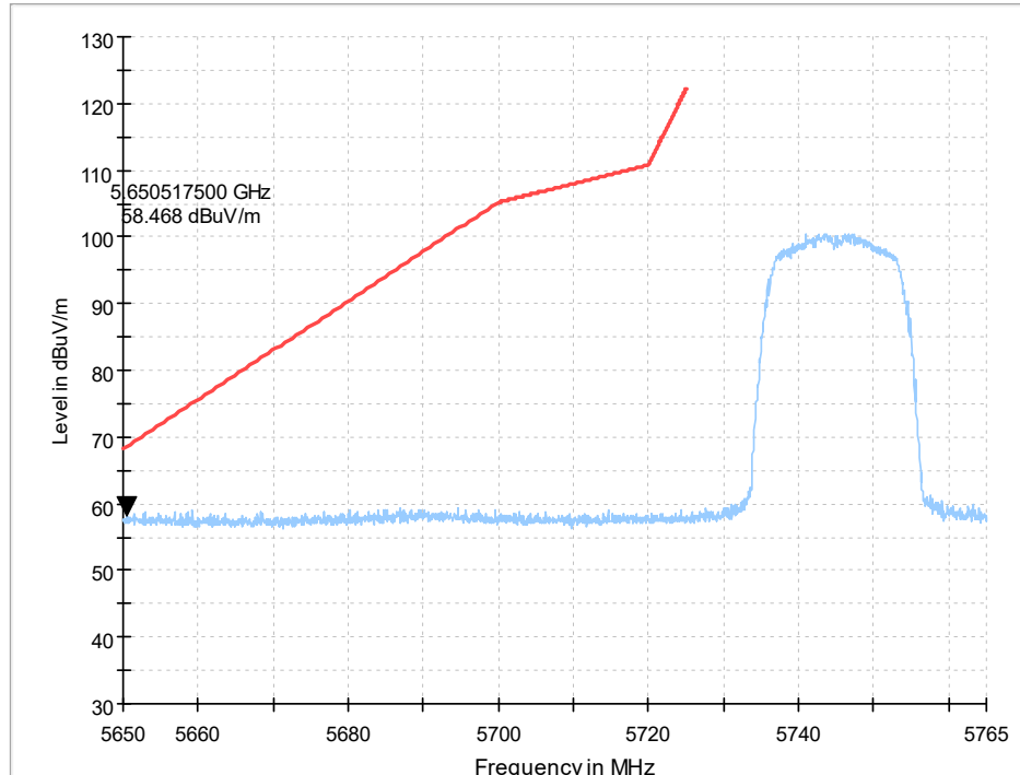
Fig. 7 Band Edges (802.11ac-HT20 Ch149, 5745MHz)
