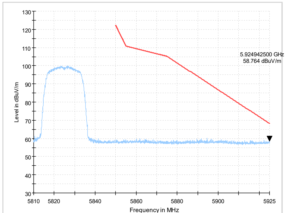
Fig. 8 Band Edges (802.11ac-HT20 Ch165, 5825MHz)
