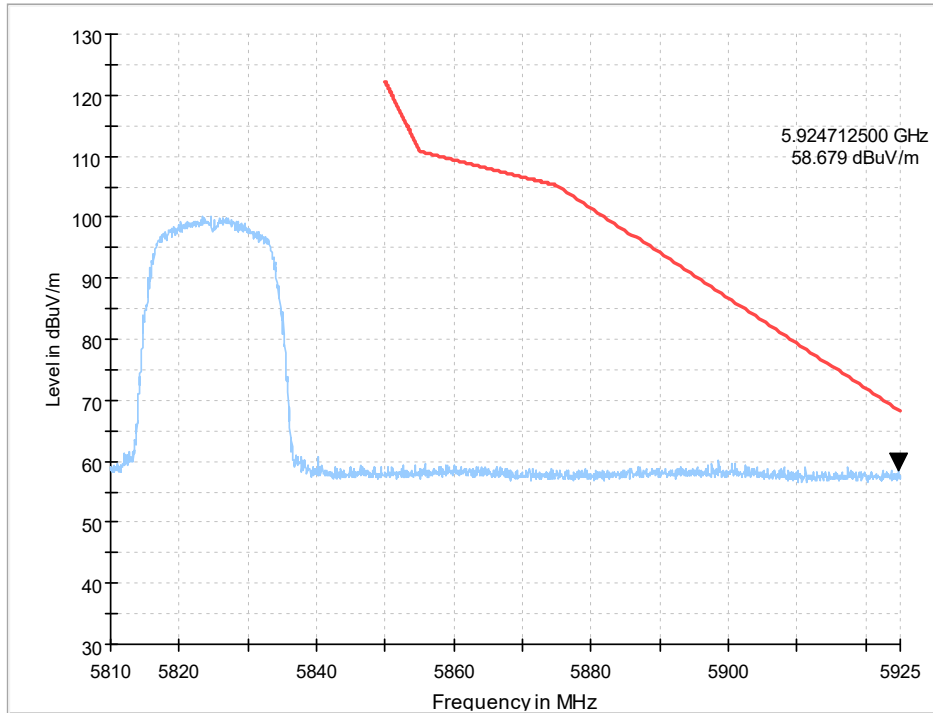
Fig. 4 Band Edges (802.11n-HT20 Ch165, 5825MHz)
