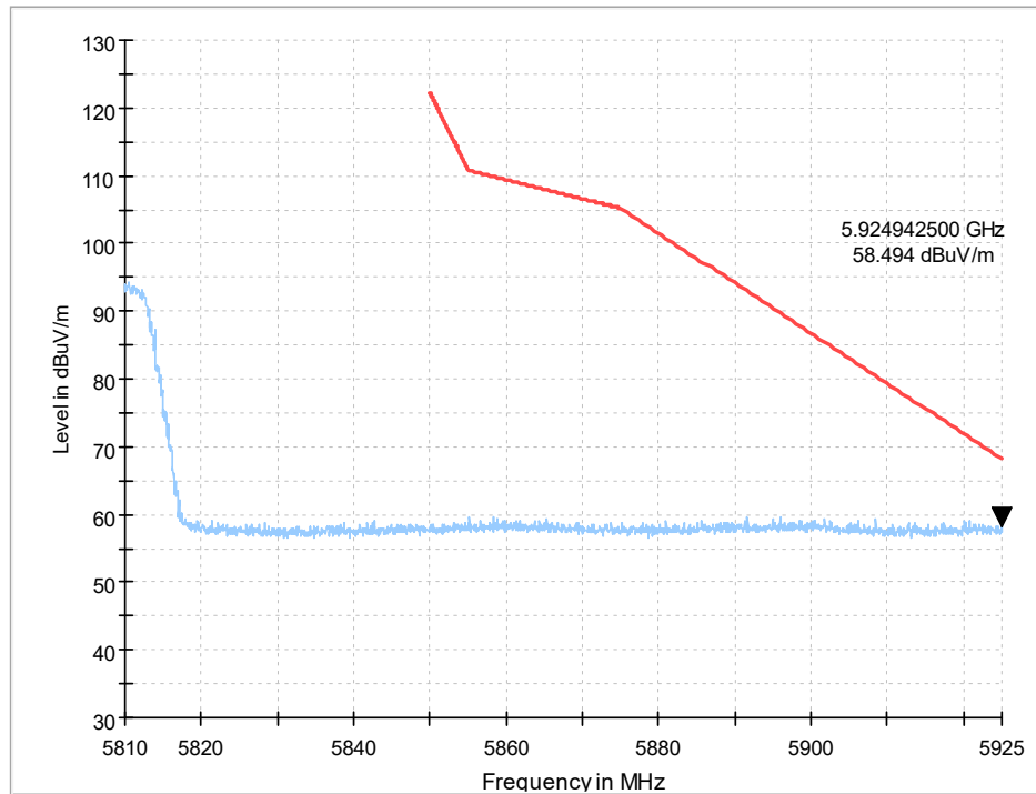
Fig. 10 Band Edges (802.11ac-HT40 Ch159, 5795MHz)
