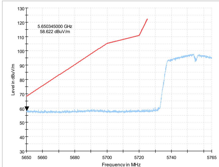
Fig. 9 Band Edges (802.11ac-HT40 Ch151, 5755MHz)
