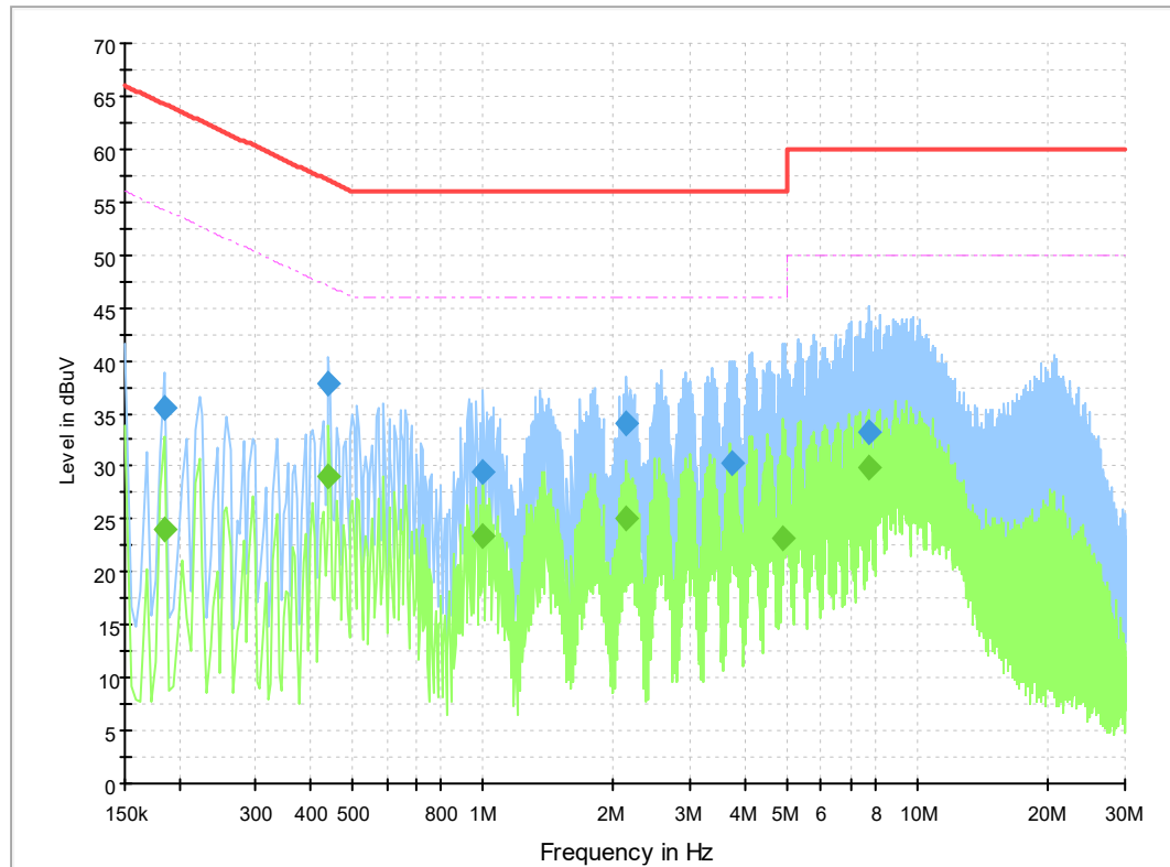
Fig. 14 AC Powerline Conducted Emission-Idle
