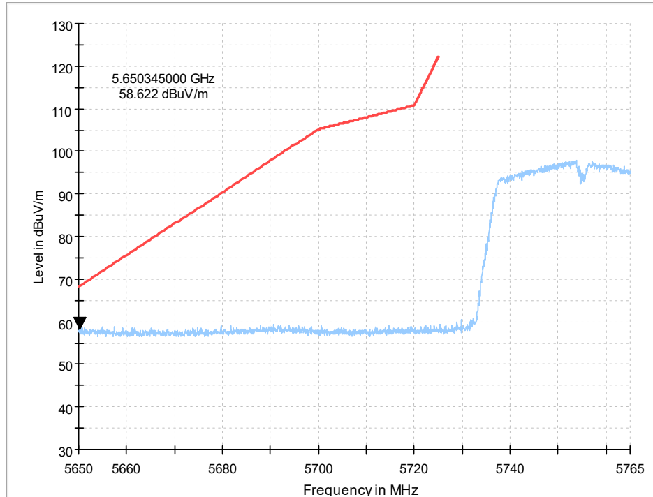
Fig. 9 Band Edges (802.11ac-HT40 Ch151, 5755MHz)
