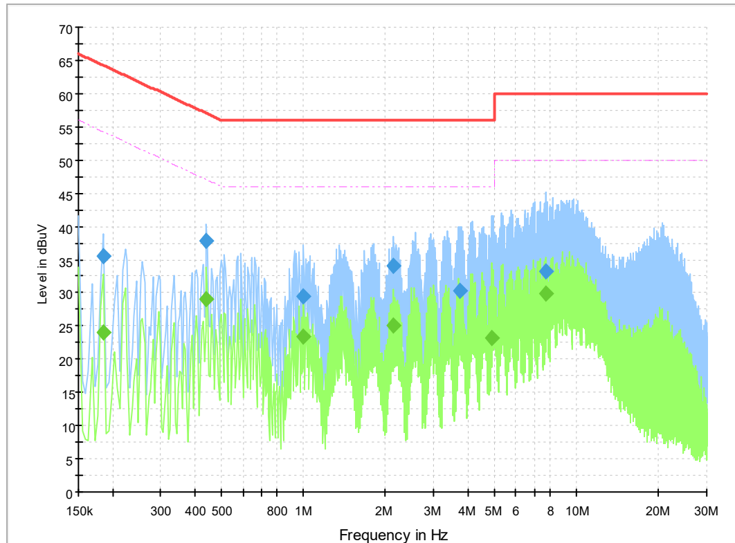
Fig. 14 AC Powerline Conducted Emission-Idle
