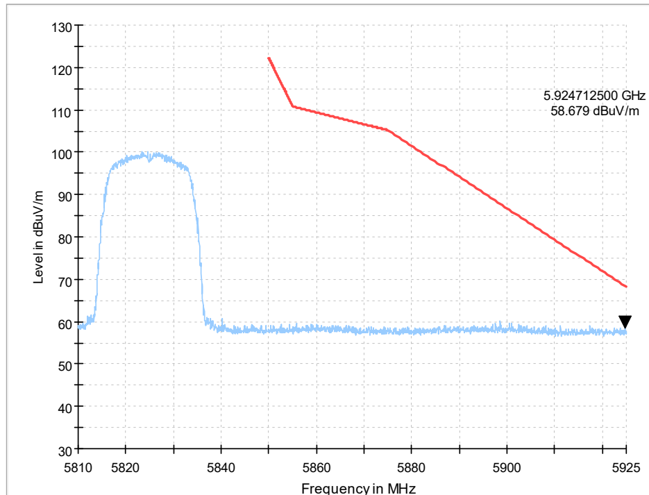
Fig. 4 Band Edges (802.11n-HT20 Ch165, 5825MHz)
