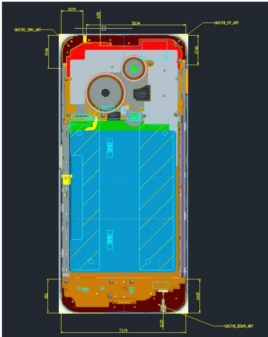
Picture 12: Antenna Locations
