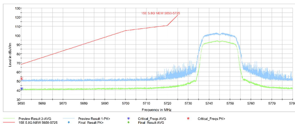
Fig. 1 Band Edges (802.11a Ch149,5745MHz)
