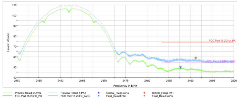
Fig. 7.2 Transmitter Spurious Emission - Radiated (Power): 802.11b, ch11, 2.45 GHz - 2.50GHz
