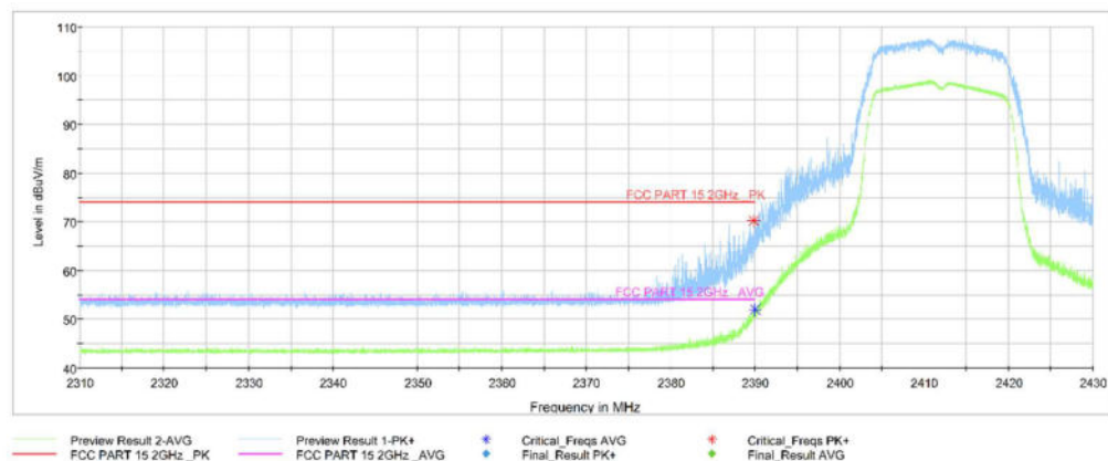
Fig. 7.3 Transmitter Spurious Emission - Radiated (Power): 802.11g, ch1, 2.31 GHz - 2.43GHz
