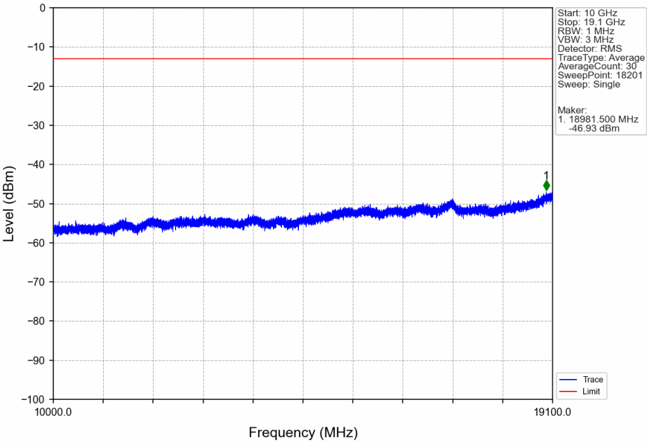
BandII_RMC_HCH_1907.6MHz_12.2kbps_RMC_NTNV
