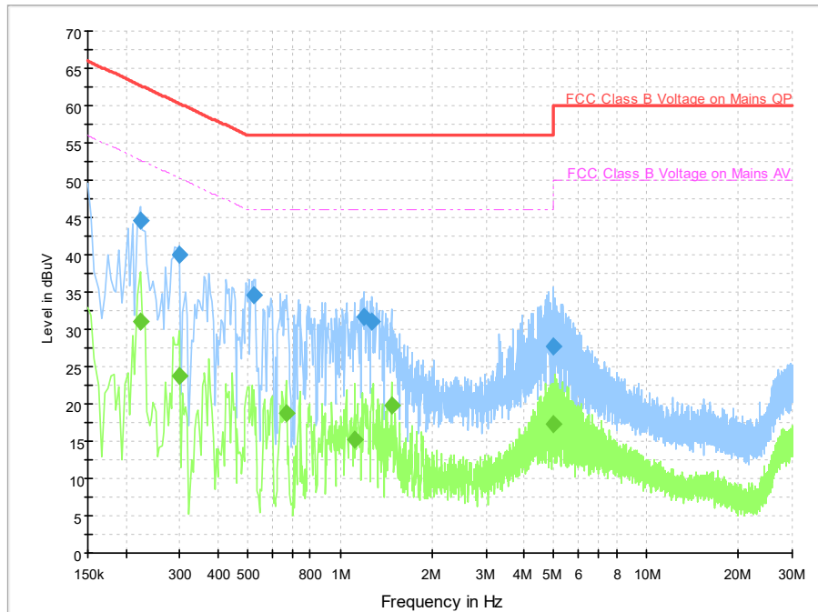
Figure A.12 Conducted Emission
