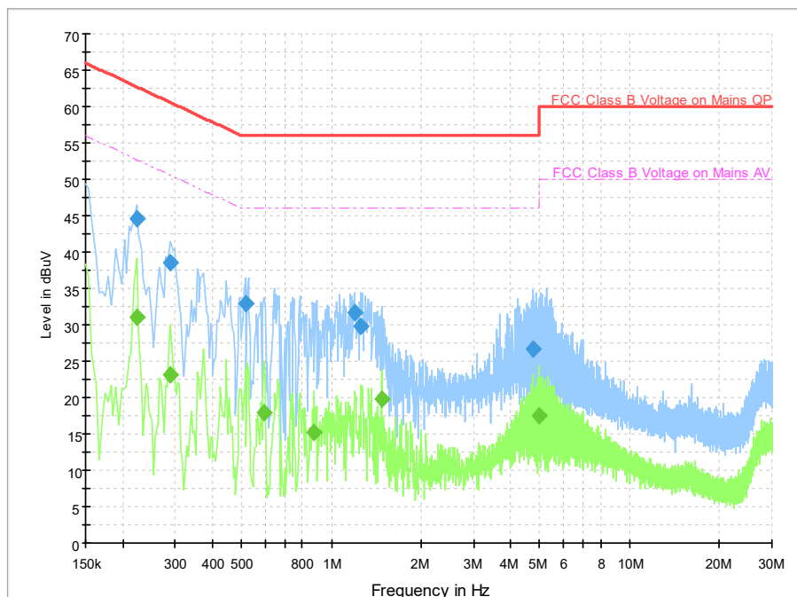
Figure A.13 Conducted Emission
