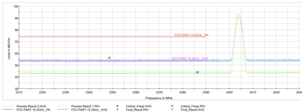
Fig.1. Frequency Band Edges: GFSK, 2404 MHz, Hopping Off, 2.31 GHz – 2.43GHz
