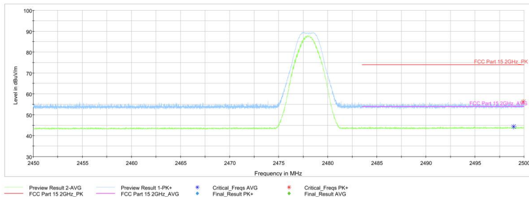
Fig.2. Frequency Band Edges: GFSK, 2478 MHz, Hopping Off, 2.45 GHz - 2.50GHz
