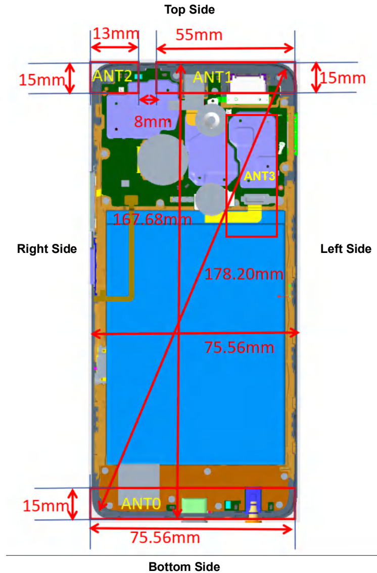
Picture 11.1 Antenna Locations (Back View)
