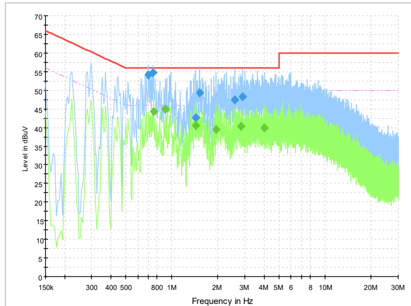
Fig.A.8.2 AC Powerline Conducted Emission-Iidle
