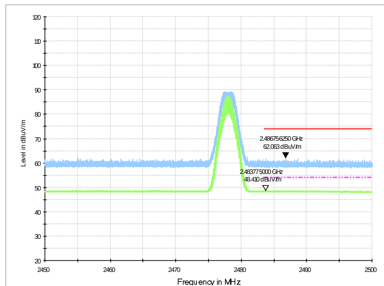
Fig.19. Frequency Band Edges: GFSK, 2478MHz, Hopping Off, 2.45 GHz - 2.50GHz
