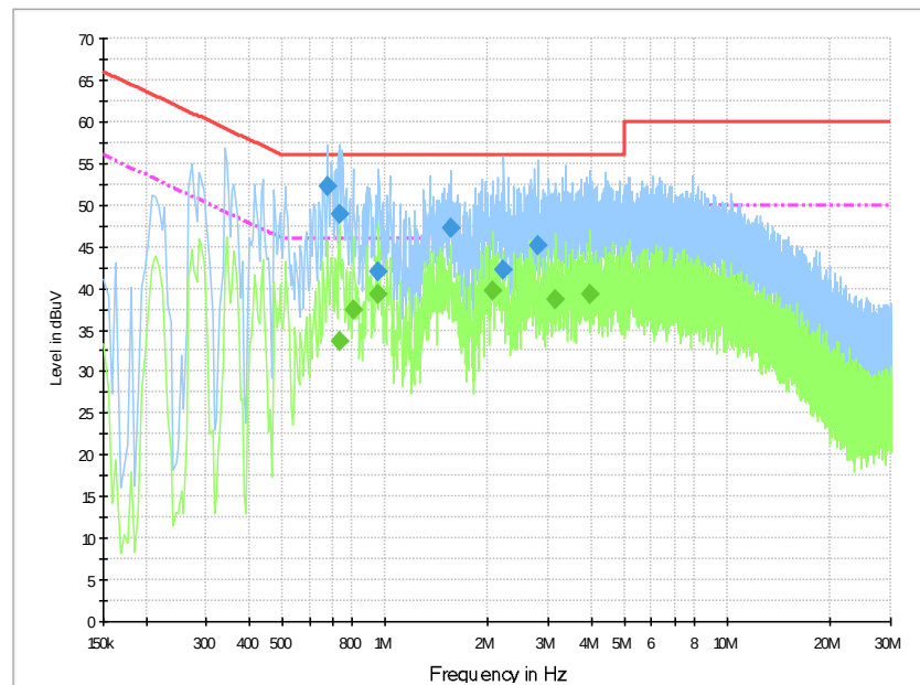
Fig.B.8.1 AC Powerline Conducted Emission- bluetooth
