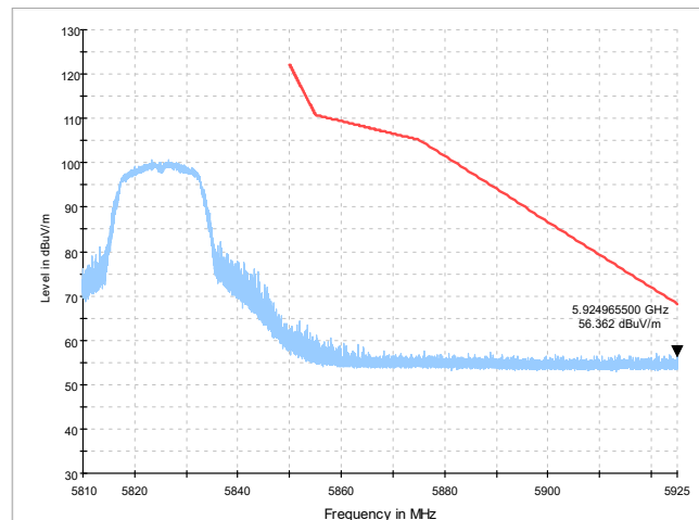
Fig. 2 Band Edges (802.11a Ch165, 5825MHz)
