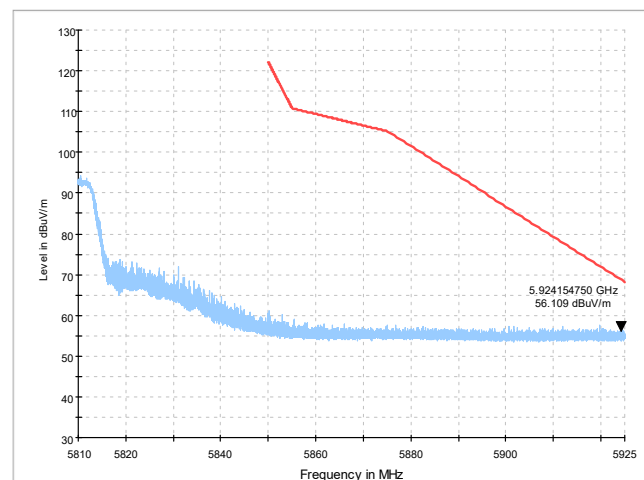
Fig. 9 Band Edges (802.11ac-HT40 Ch151, 5755MHz)
