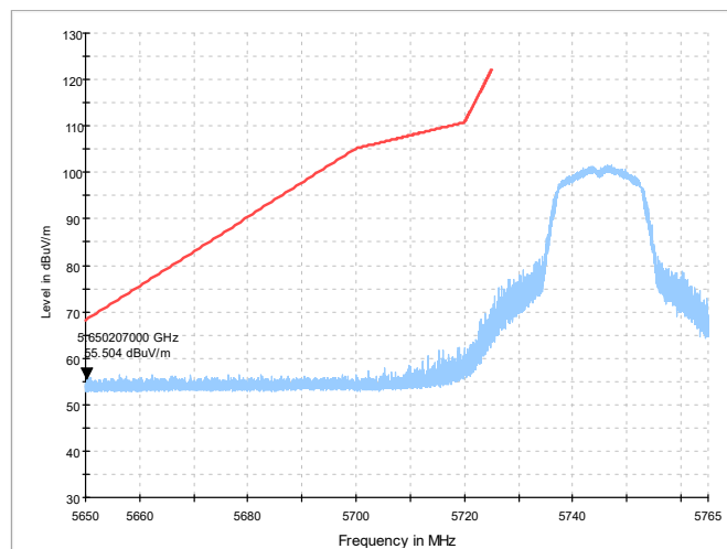
Fig. 1 Band Edges (802.11a Ch149,5745MHz)
