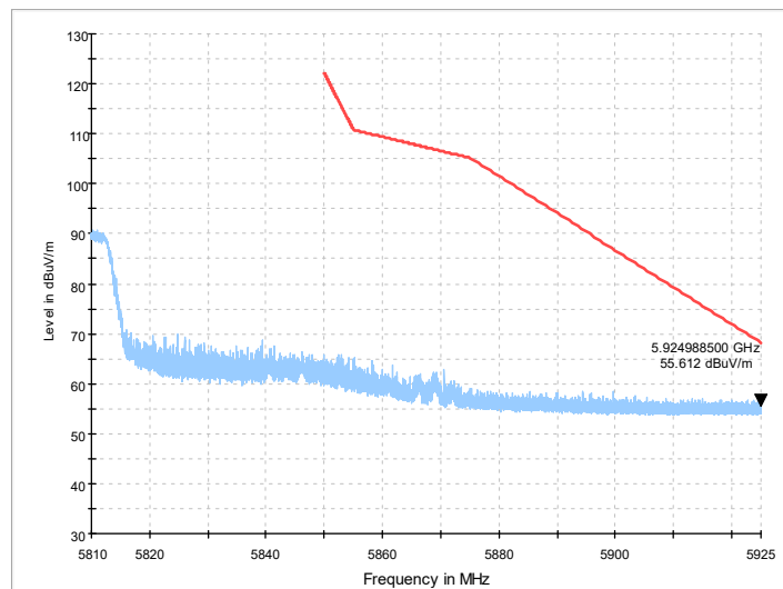
Fig. 12 Band Edges (802.11ac-HT80, 5775MHz)
