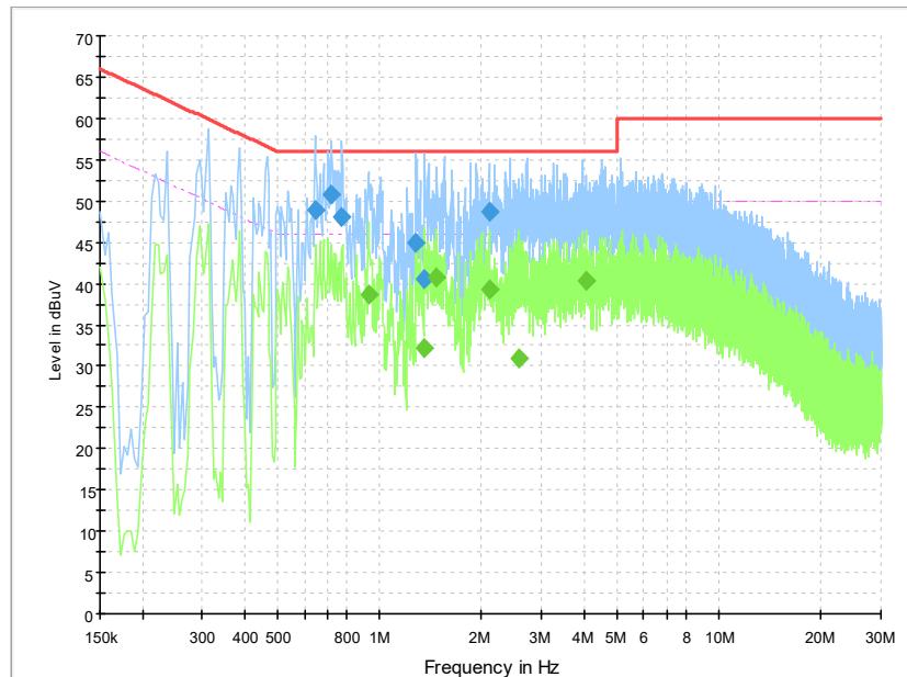
Fig.A.6.1. AC Powerline Conducted Emission-Ide
