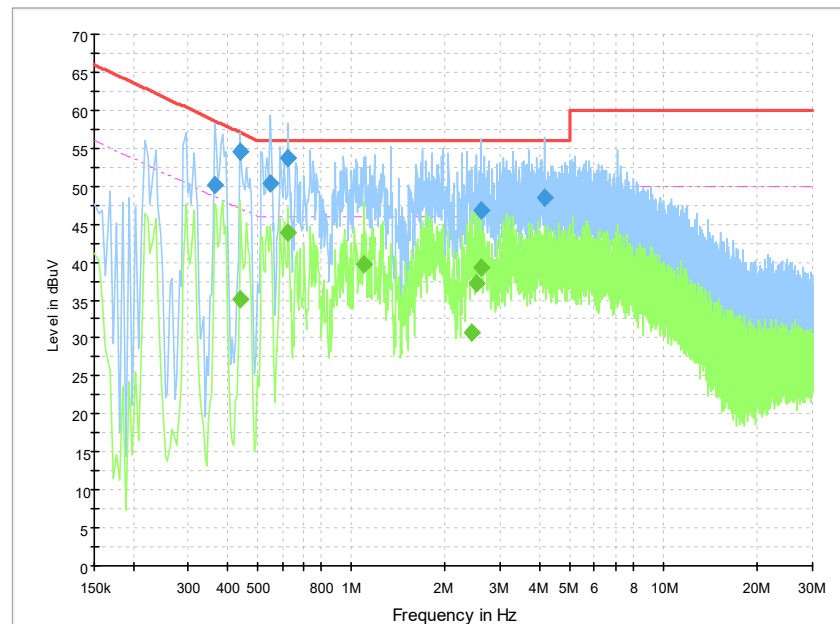
Fig.A.6.2. AC Powerline Conducted Emission-Ide
