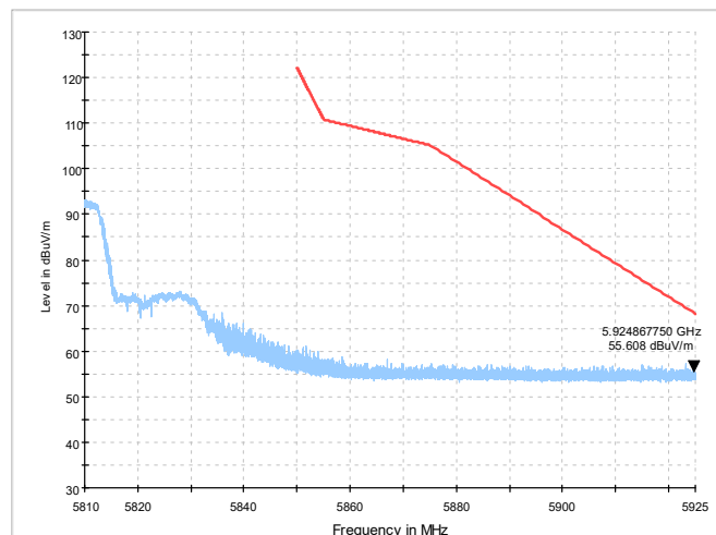
Fig. 6 Band Edges (802.11n-HT40 Ch159, 5795MHz)
