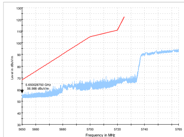
Fig. 11 Band Edges (802.11ac-HT80 Ch155, 5775MHz)
