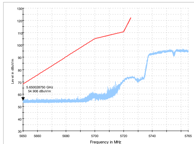
Fig. 5 Band Edges (802.11n-HT40 Ch151, 5755MHz)
