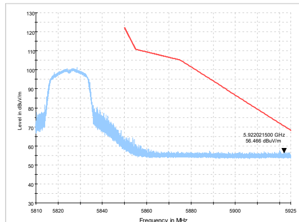
Fig. 8 Band Edges (802.11ac-HT20 Ch165, 5825MHz)
