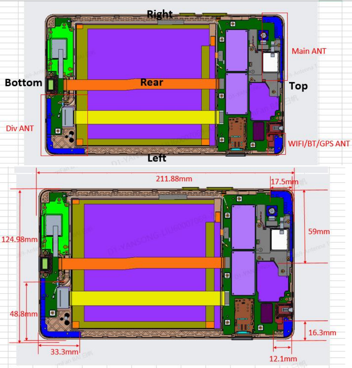
Antenna area diagram
