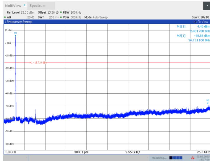
11N40SISO_Ant1_2452_0~Reference
