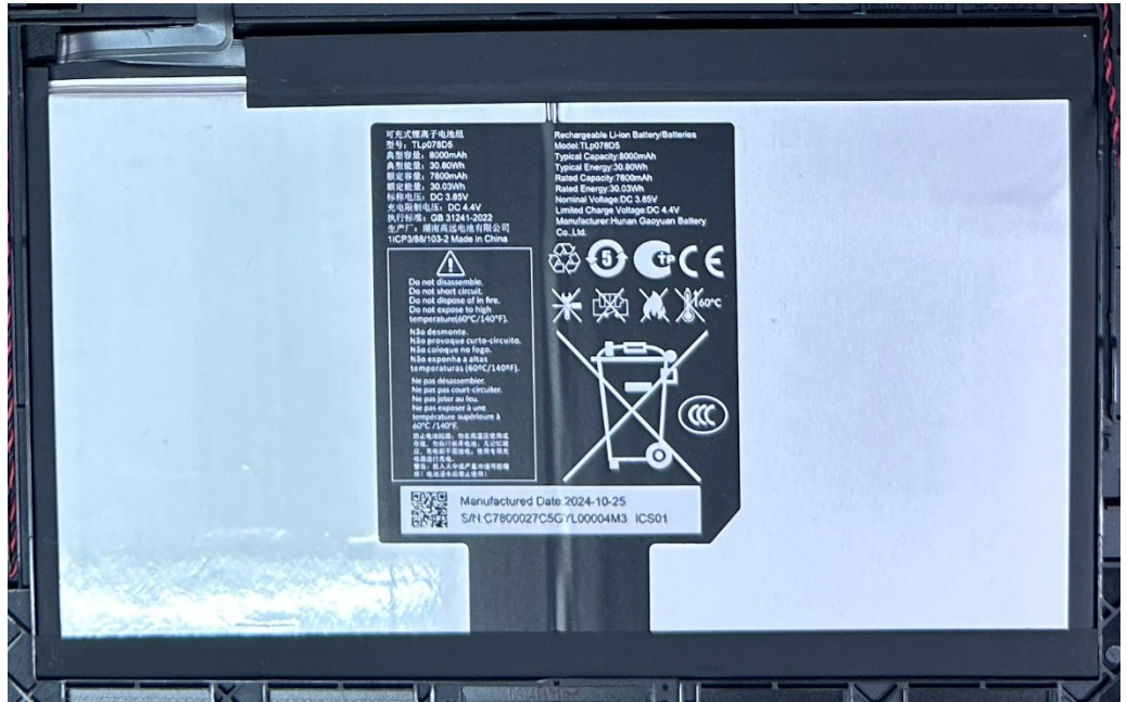
Battery TLp078D5
