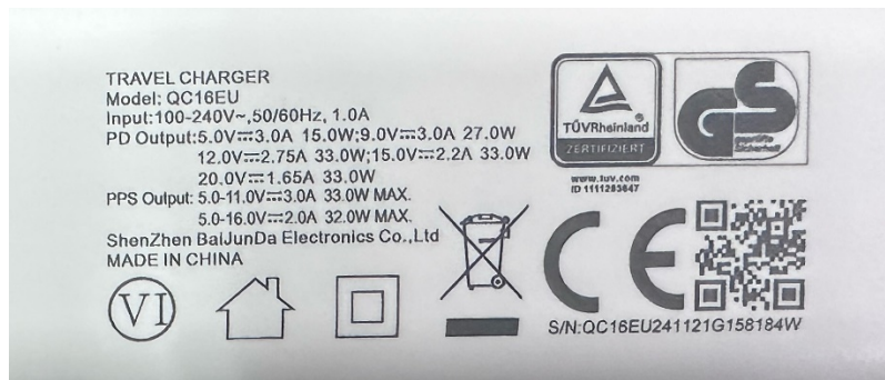
Charger QC16EU_label
