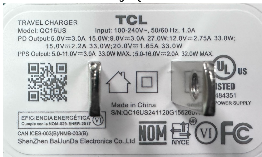
Charger QC16US_label
