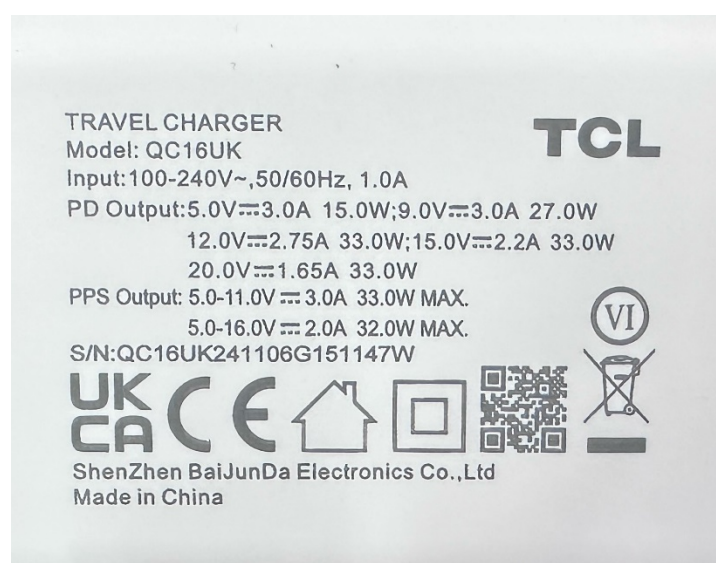
Charger QC16UK_label
