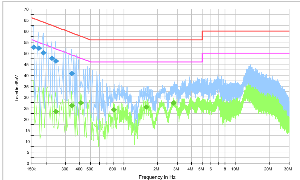
Fig.A.6.1. AC Powerline Conducted Emission-Iidle
