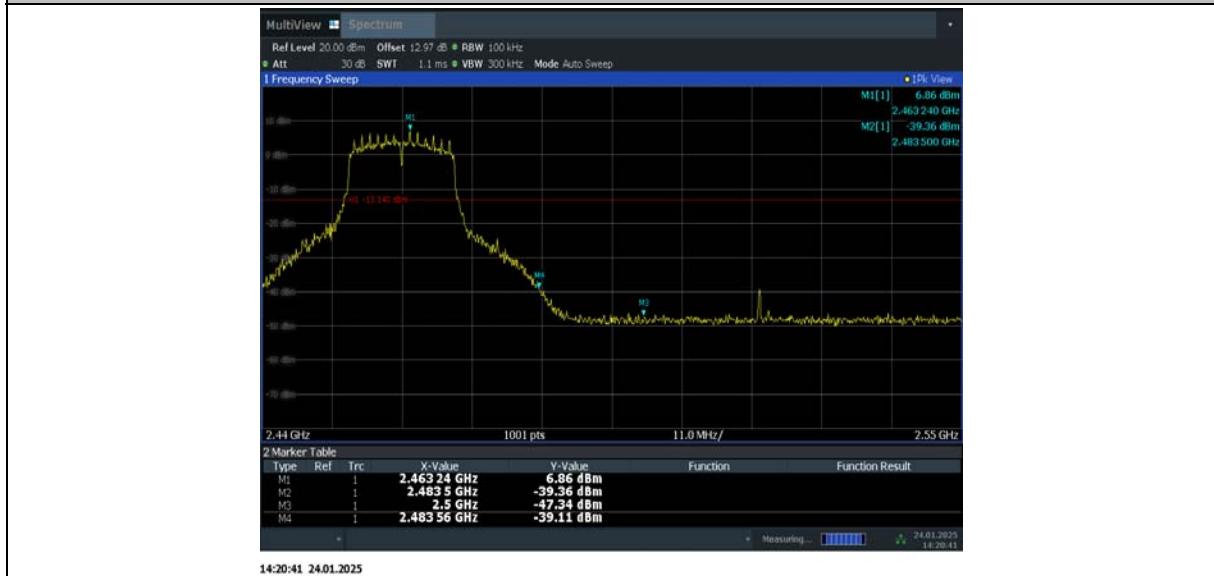
11N20SISO_Ant1_Low_2412
