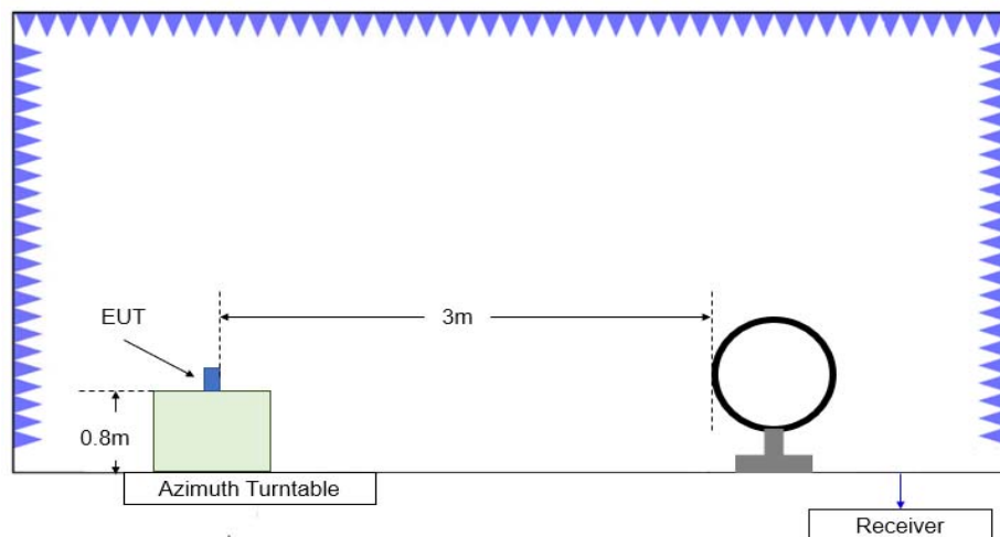
Figure B.5.1. Test Site Diagram (9kHz-30MHz)
