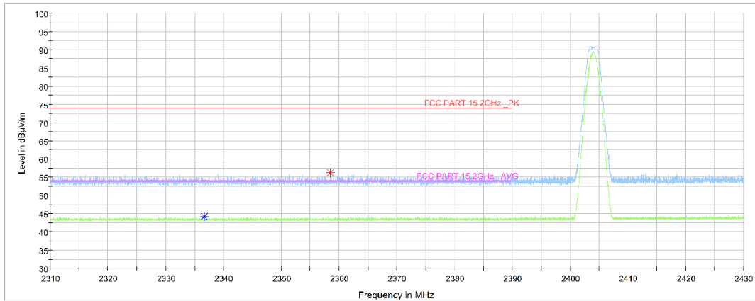
Fig.18. Frequency Band Edges: GFSK, 2404 MHz, Hopping Off, 2.31 GHz – 2.43GHz
