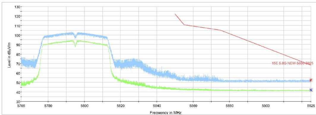
Fig. 6 Band Edges (802.11n-HT40 Ch159, 5795MHz)
