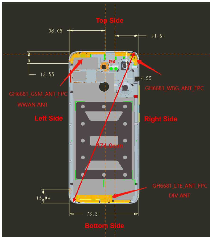
Picture 11.1 Antenna Locations (Front View)
