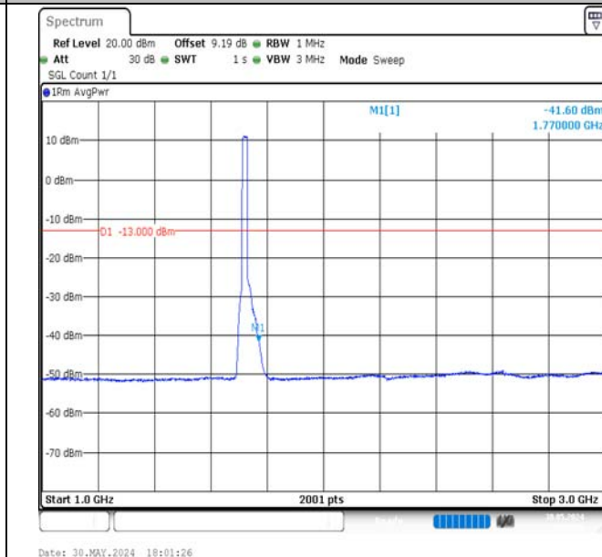
Band4-20MHz-16QAM-20050-100RB#0-1000~3000-PASS
