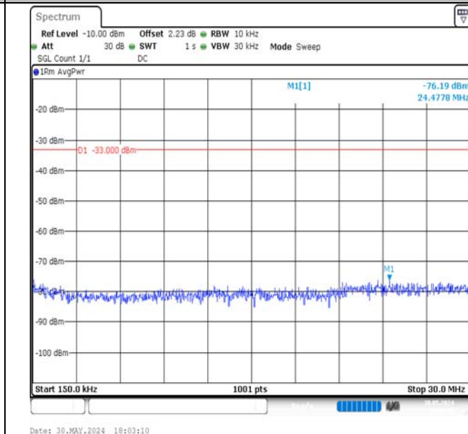
Band4-20MHz-QPSK-20175-100RB#0-0.15~30-PASS
