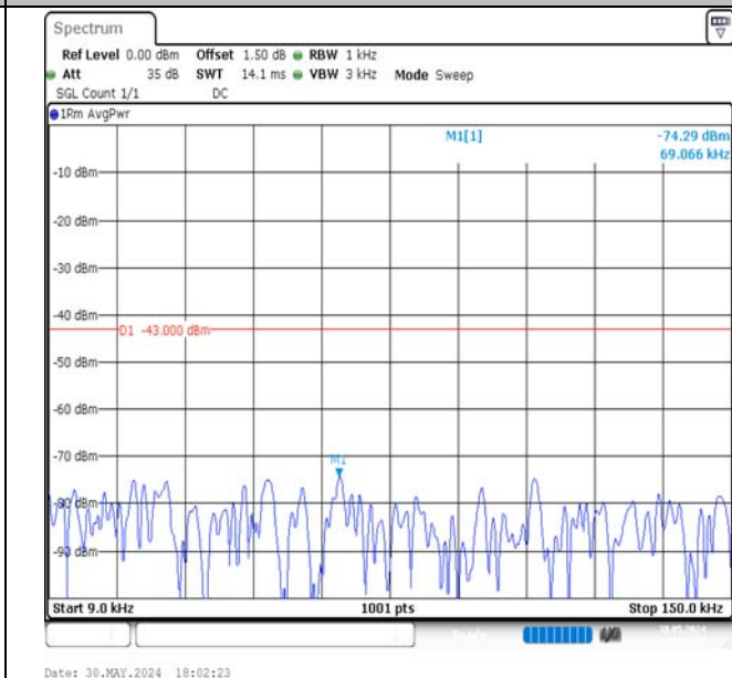
Band4-20MHz-QPSK-20175-1RB#99-0.009~0.15-PASS
