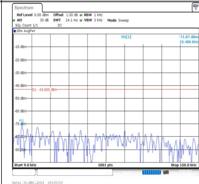
Band4-20MHz-QPSK-20050-100RB#0-0.009~0.15-PASS
