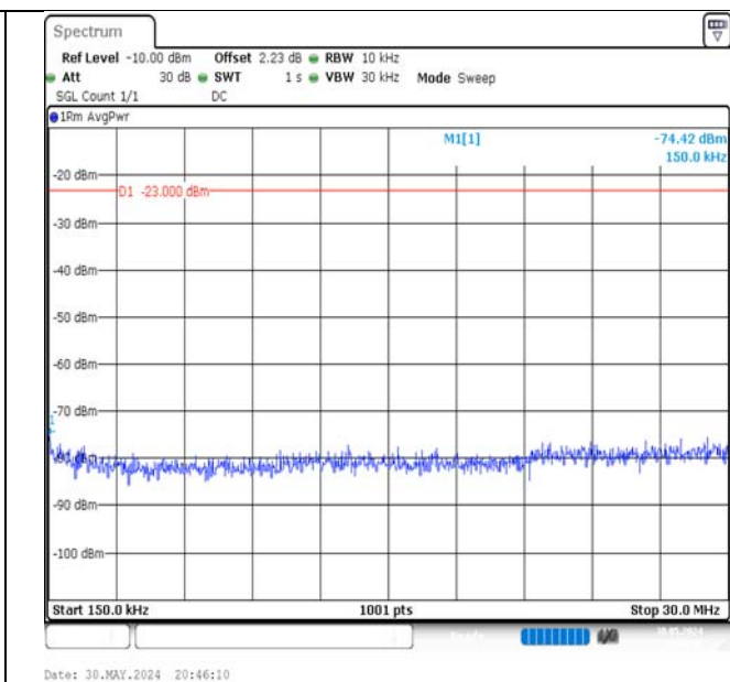
Band5-1.4MHz-QPSK-20407-1RB#0-0.15~30-PASS
