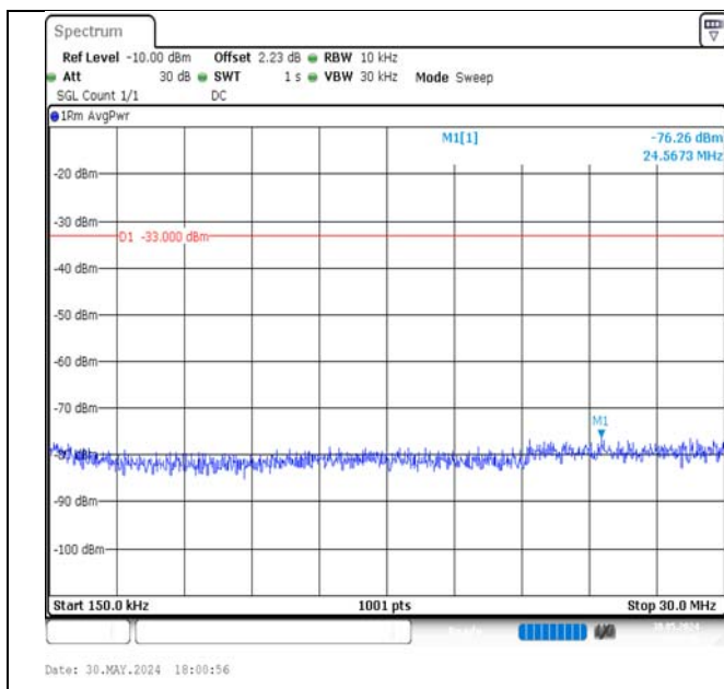
Band4-20MHz-QPSK-20050-100RB#0-0.15~30-PASS
