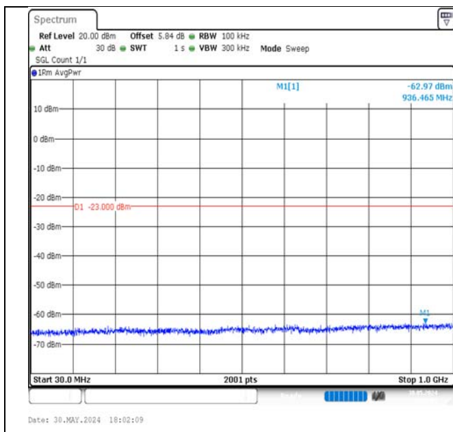
Band4-20MHz-16QAM-20175-1RB#0-30~1000-PASS
