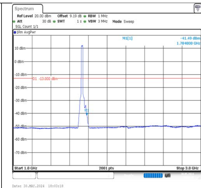
Band4-20MHz-QPSK-20175-100RB#0-1000~3000-PASS
