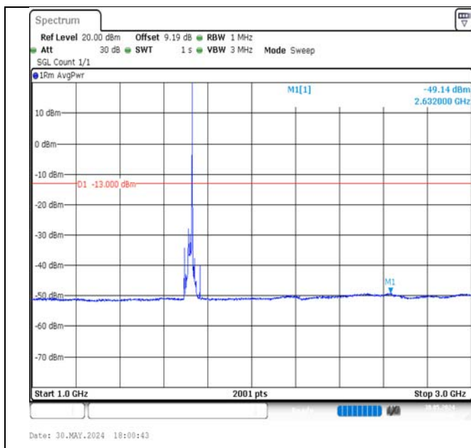
Band4-20MHz-16QAM-20050-1RB#99-1000~3000-PASS
