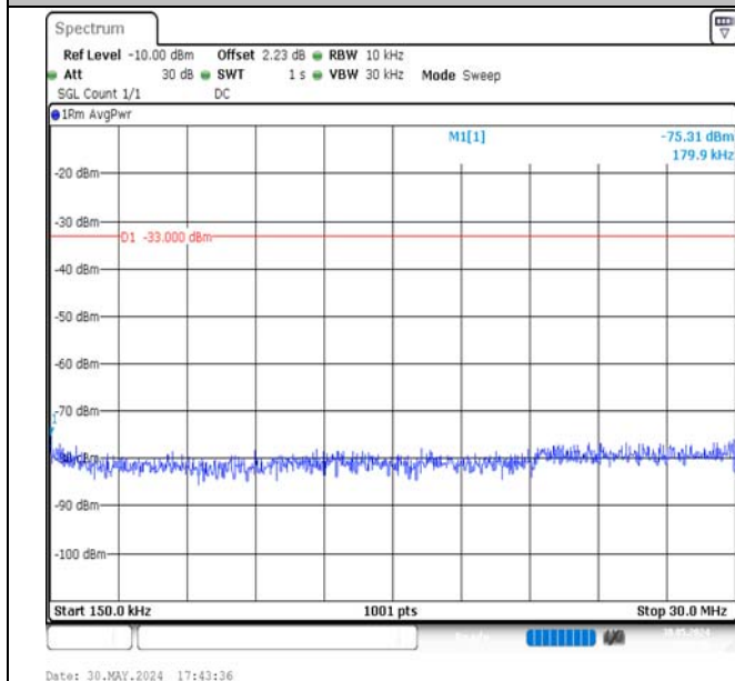
Band4-15MHz-16QAM-20175-75RB#0-0.15~30-PASS
