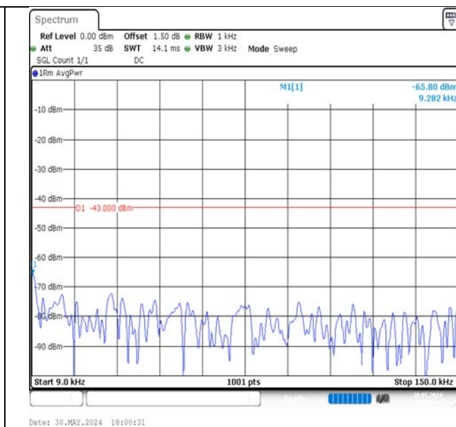
Band4-20MHz-16QAM-20050-1RB#99-0.009~0.15-PASS
