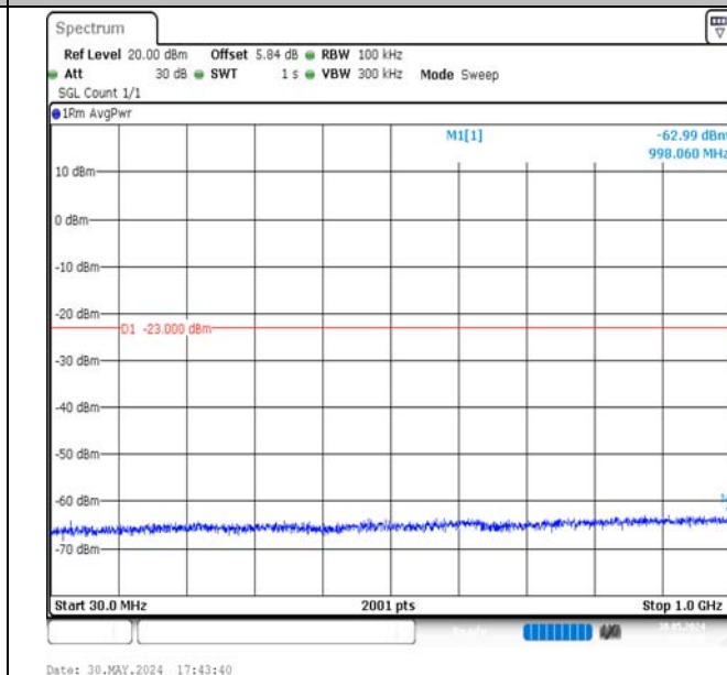
Band4-15MHz-16QAM-20175-75RB#0-30~1000-PASS
