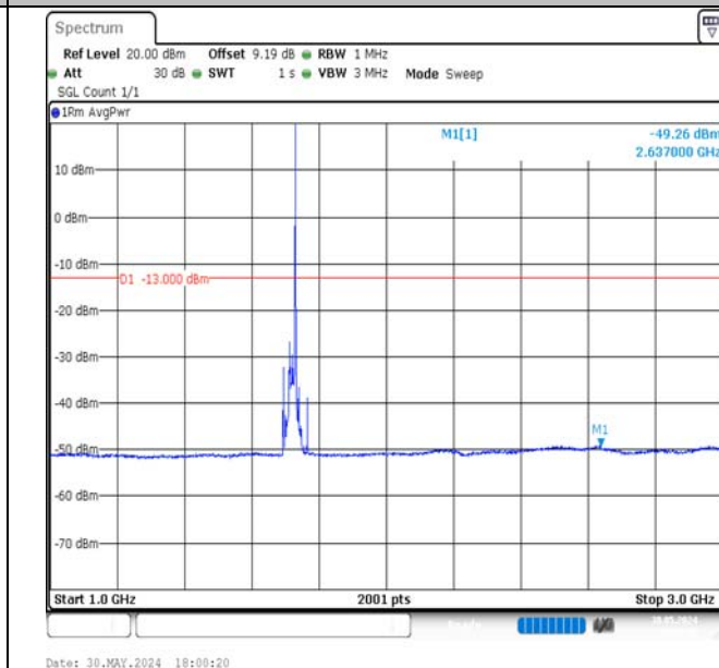
Band4-20MHz-QPSK-20050-1RB#99-1000~3000-PASS
