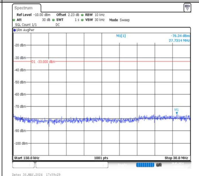
Band4-20MHz-QPSK-20050-1RB#0-0.15~30-PASS
