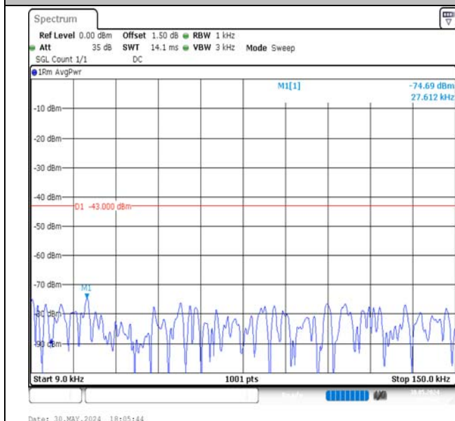
Band4-20MHz-16QAM-20300-100RB#0-0.009~0.15-PASS
