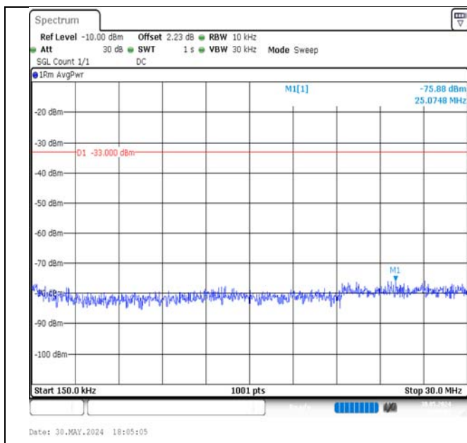
Band4-20MHz-16QAM-20300-1RB#99-0.15~30-PASS
