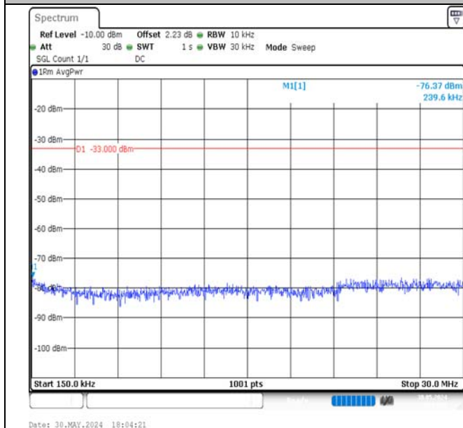
Band4-20MHz-16QAM-20300-1RB#0-0.15~30-PASS
