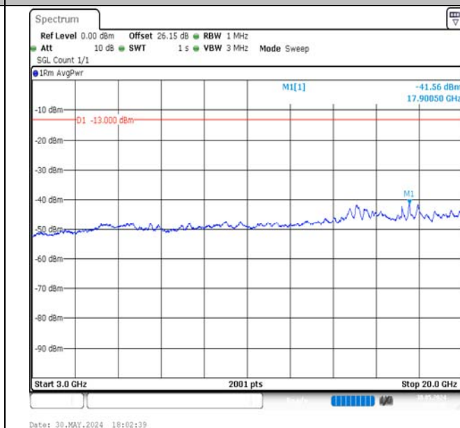
Band4-20MHz-QPSK-20175-1RB#99-3000~20000-PASS
