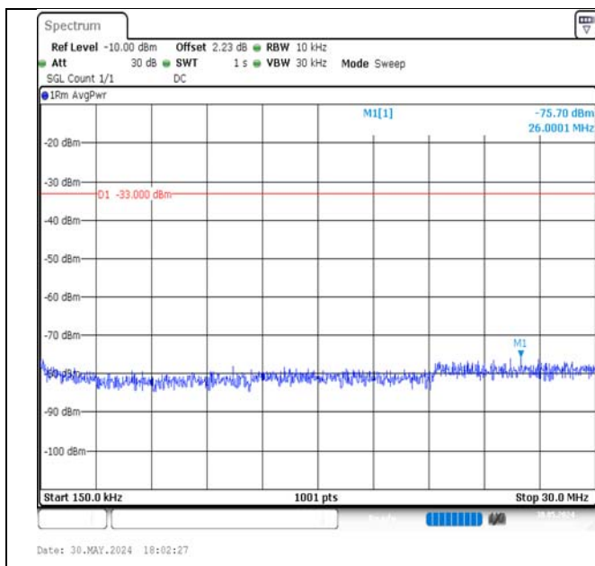
Band4-20MHz-QPSK-20175-1RB#99-0.15~30-PASS
