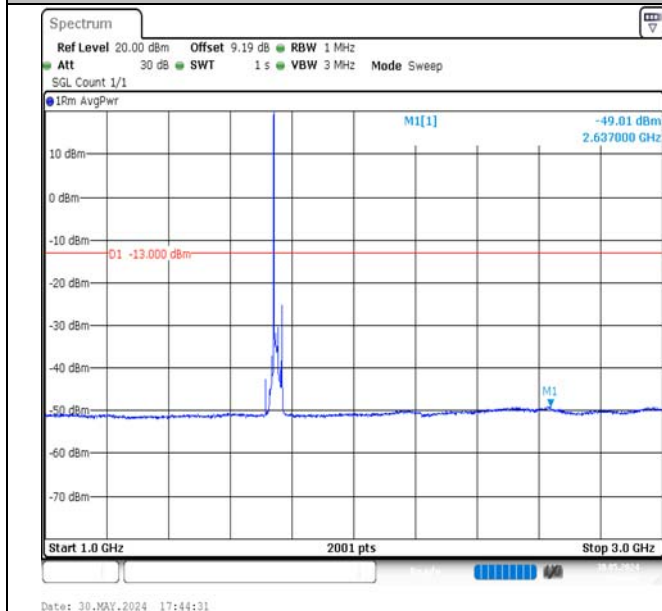
Band4-15MHz-16QAM-20325-1RB#0-1000~3000-PASS
