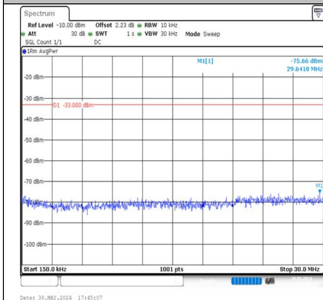
Band4-15MHz-16QAM-20325-1RB#74-0.15~30-PASS
