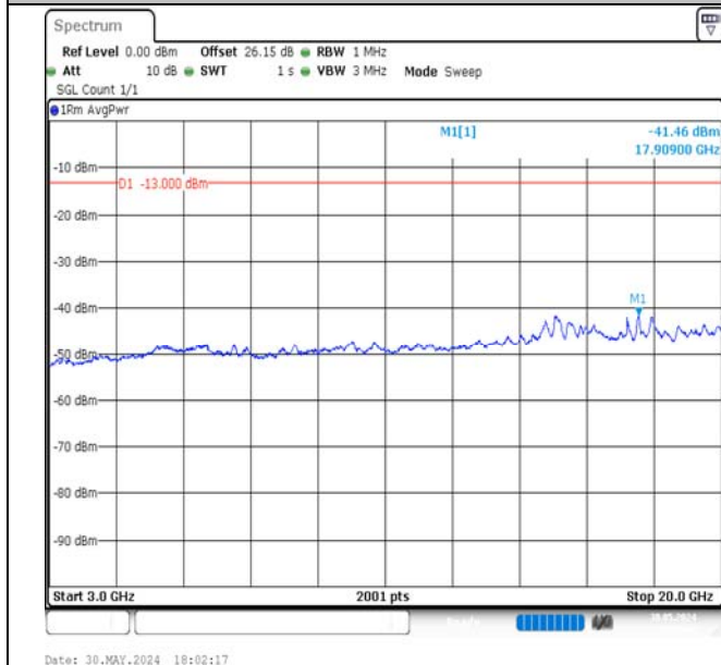
Band4-20MHz-16QAM-20175-1RB#0-3000~20000-PASS
