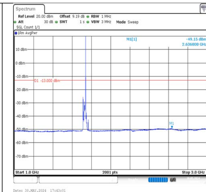
Band4-15MHz-16QAM-20175-1RB#74-1000~3000-PASS
