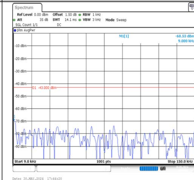
Band4-15MHz-16QAM-20325-1RB#0-0.009~0.15-PASS
