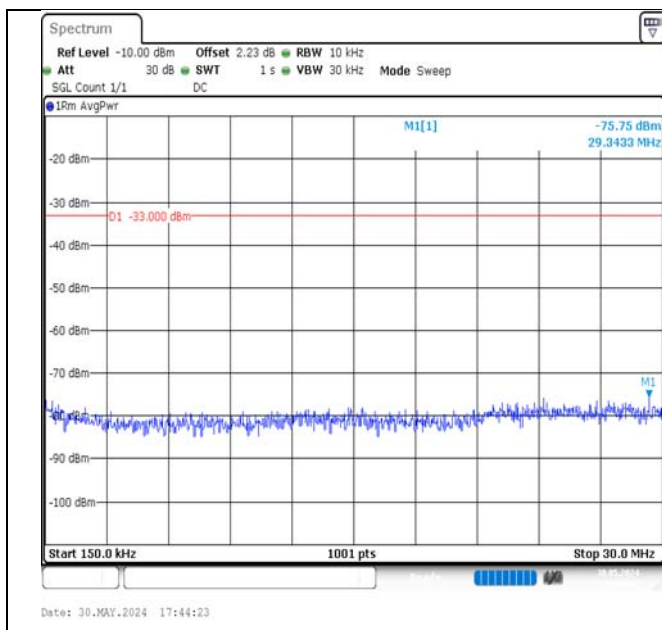
Band4-15MHz-16QAM-20325-1RB#0-0.15~30-PASS
