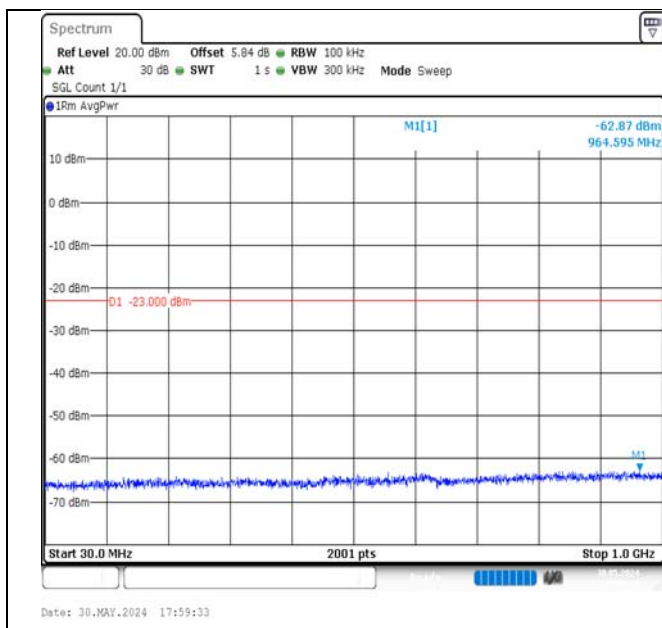
Band4-20MHz-QPSK-20050-1RB#0-30~1000-PASS
