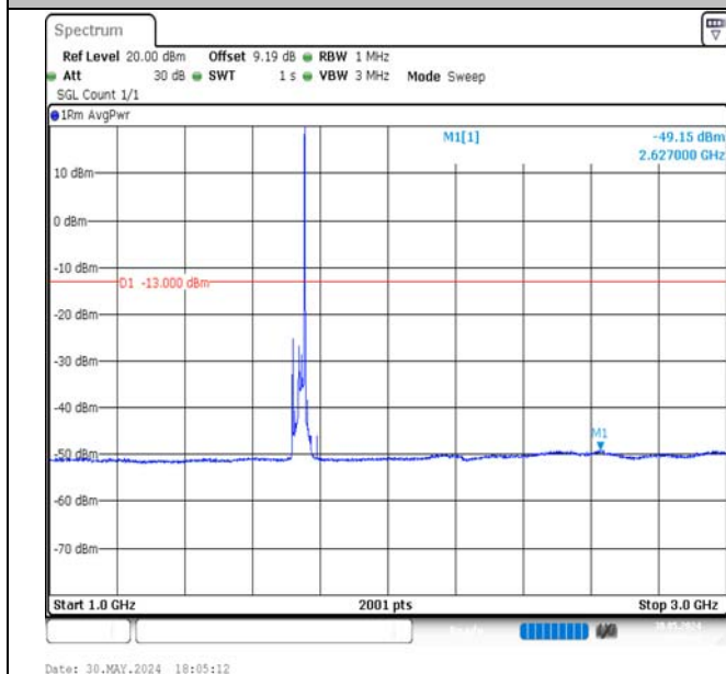
Band4-20MHz-16QAM-20300-1RB#99-1000~3000-PASS
