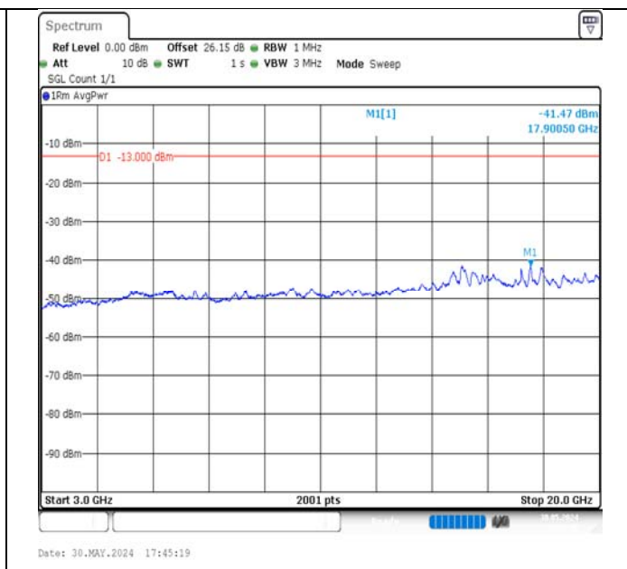
Band4-15MHz-16QAM-20325-1RB#74-3000~20000-PASS
