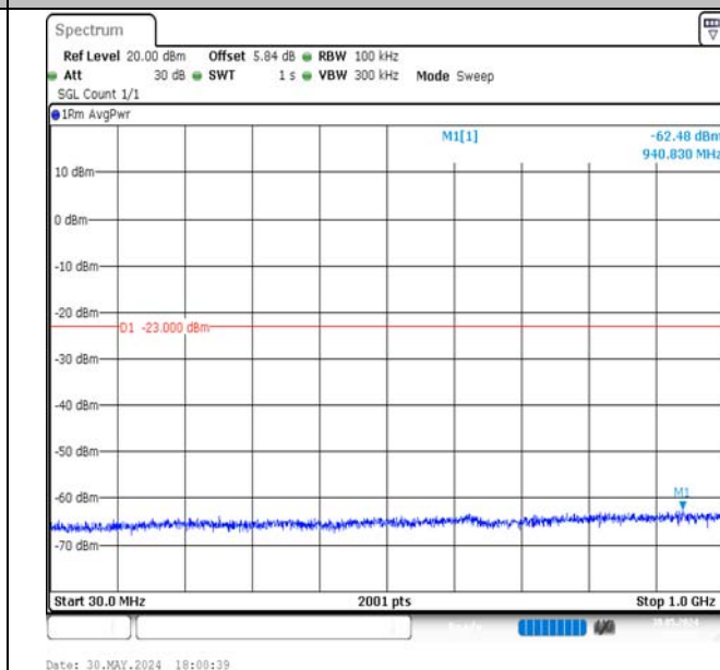
Band4-20MHz-16QAM-20050-1RB#99-30~1000-PASS
