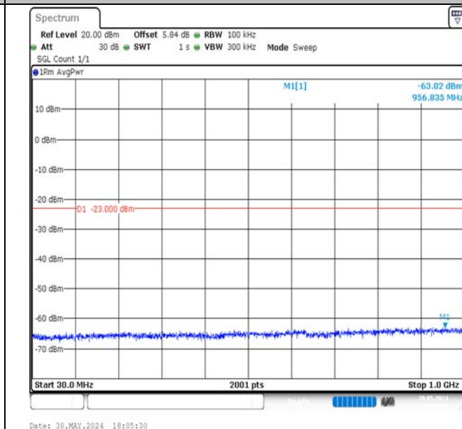
Band4-20MHz-QPSK-20300-100RB#0-30~1000-PASS
