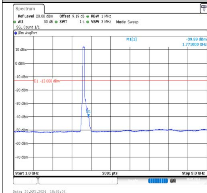
Band4-20MHz-QPSK-20050-100RB#0-1000~3000-PASS
