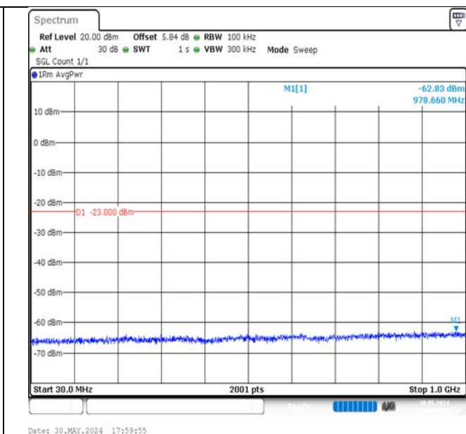
Band4-20MHz-16QAM-20050-1RB#0-30~1000-PASS
