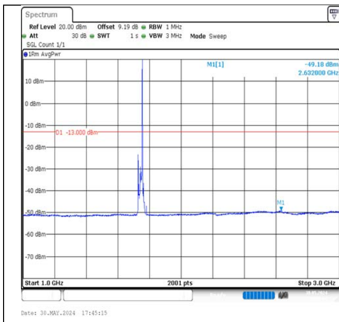
Band4-15MHz-16QAM-20325-1RB#74-1000~3000-PASS
