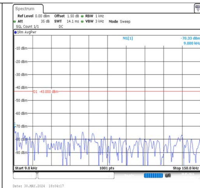
Band4-20MHz-16QAM-20300-1RB#0-0.009~0.15-PASS
