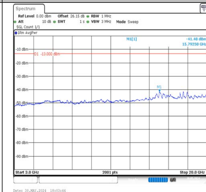
Band4-20MHz-16QAM-20175-100RB#0-3000~20000-PASS
