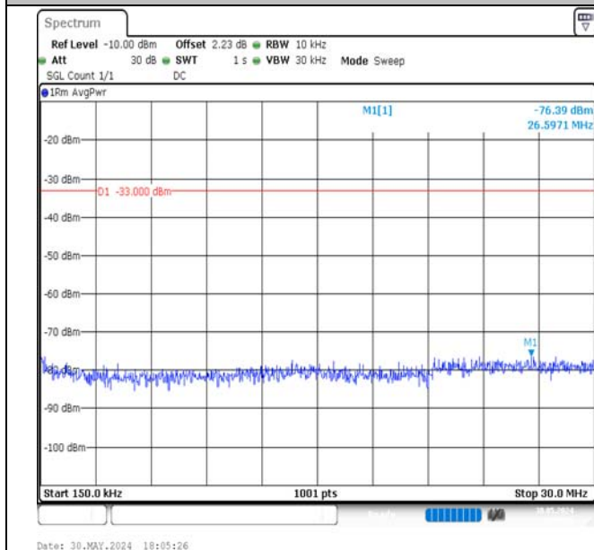
Band4-20MHz-QPSK-20300-100RB#0-0.15~30-PASS
