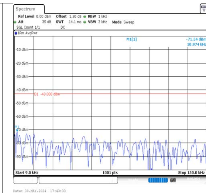
Band4-15MHz-16QAM-20175-75RB#0-0.009~0.15-PASS
