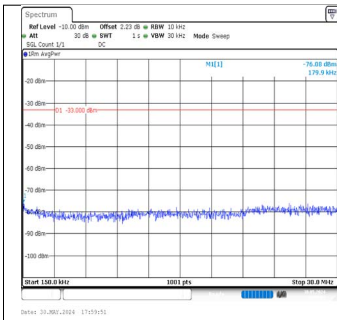
Band4-20MHz-16QAM-20050-1RB#0-0.15~30-PASS
