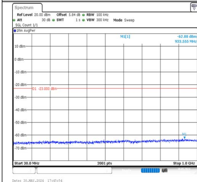
Band4-15MHz-16QAM-20325-75RB#0-30~1000-PASS
