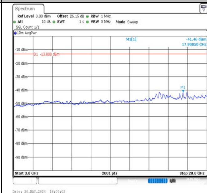
Band4-20MHz-16QAM-20050-1RB#0-3000~20000-PASS
