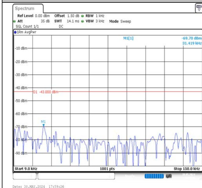
Band4-20MHz-QPSK-20050-1RB#0-0.009~0.15-PASS
