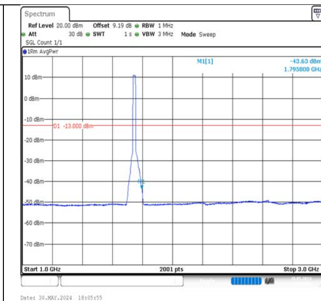
Band4-20MHz-16QAM-20300-100RB#0-1000~3000-PASS
