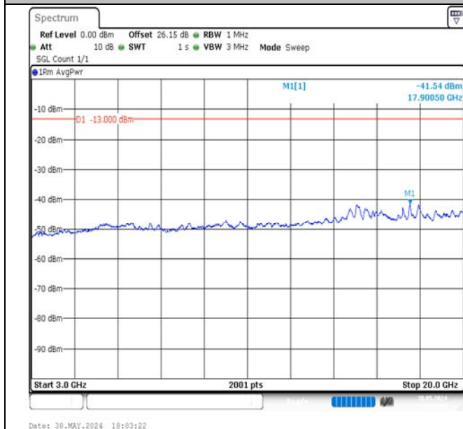
Band4-20MHz-QPSK-20175-100RB#0-3000~20000-PASS
