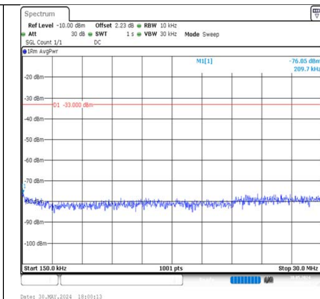
Band4-20MHz-QPSK-20050-1RB#99-0.15~30-PASS
