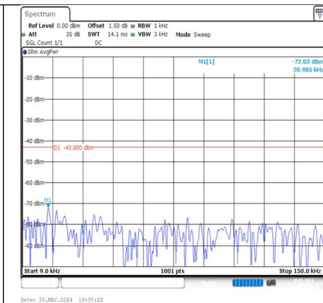
Band4-20MHz-QPSK-20300-100RB#0-0.009~0.15-PASS
