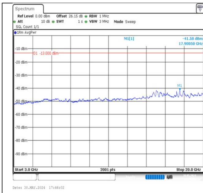
Band4-15MHz-16QAM-20325-75RB#0-3000~20000-PASS
