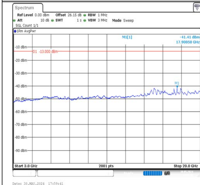
Band4-20MHz-QPSK-20050-1RB#0-3000~20000-PASS
