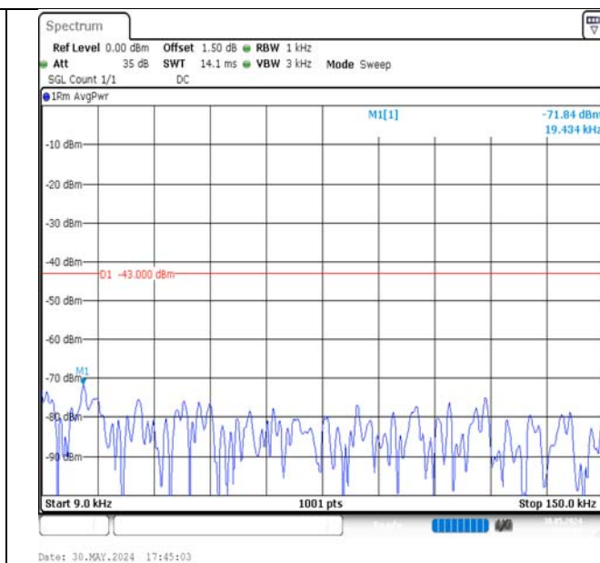
Band4-15MHz-16QAM-20325-1RB#74-0.009~0.15-PASS
