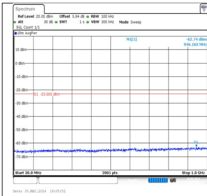
Band4-20MHz-16QAM-20300-100RB#0-30~1000-PASS
