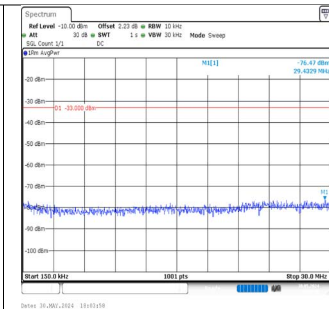
Band4-20MHz-QPSK-20300-1RB#0-0.15~30-PASS
