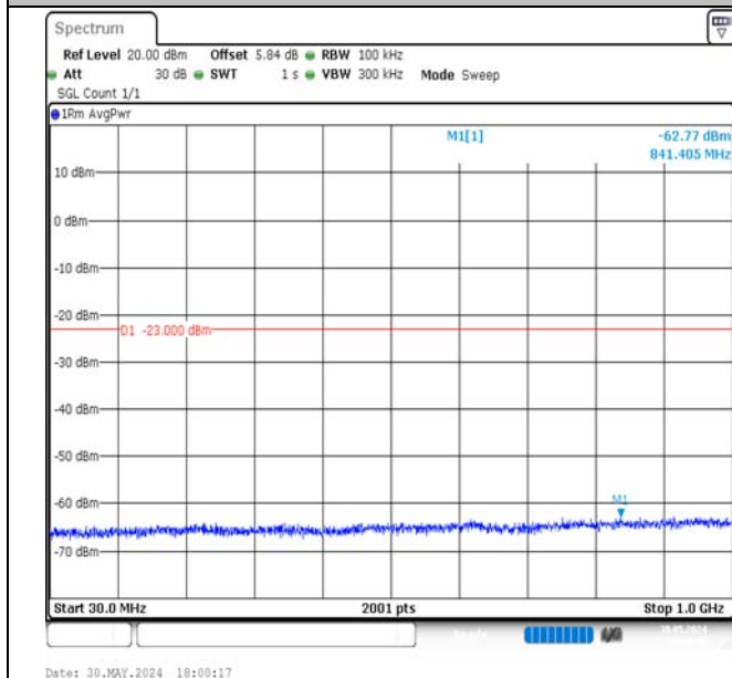
Band4-20MHz-QPSK-20050-1RB#99-30~1000-PASS
