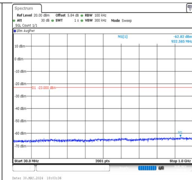
Band4-20MHz-16QAM-20175-100RB#0-30~1000-PASS
