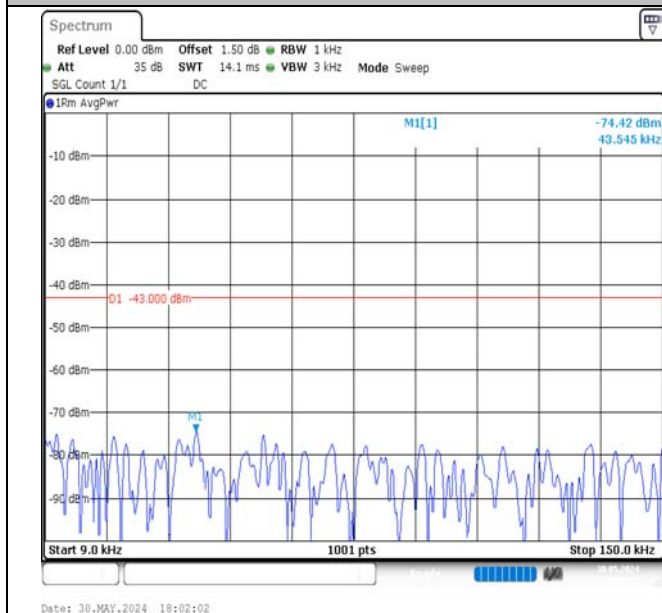
Band4-20MHz-16QAM-20175-1RB#0-0.009~0.15-PASS
