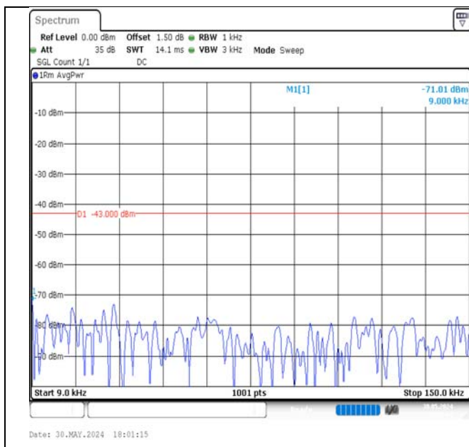
Band4-20MHz-16QAM-20050-100RB#0-0.009~0.15-PASS
