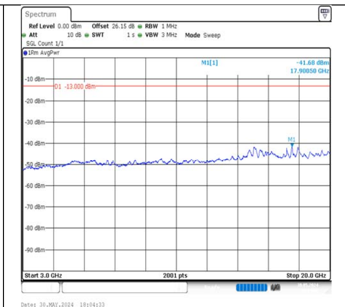
Band4-20MHz-16QAM-20300-1RB#0-3000~20000-PASS
