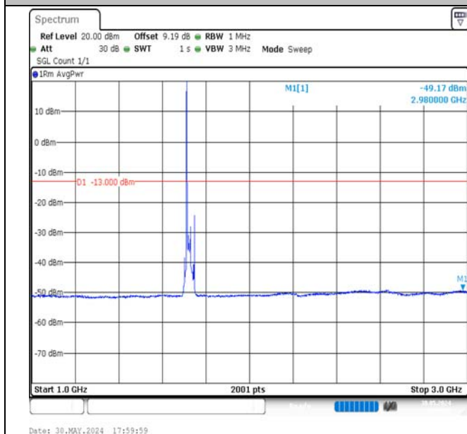
Band4-20MHz-16QAM-20050-1RB#0-1000~3000-PASS
