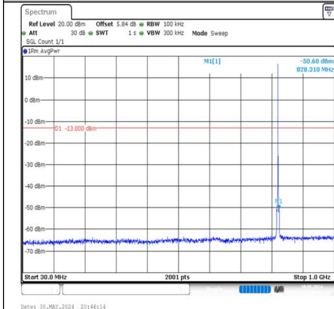
Band5-1.4MHz-QPSK-20407-1RB#0-30~1000-PASS
