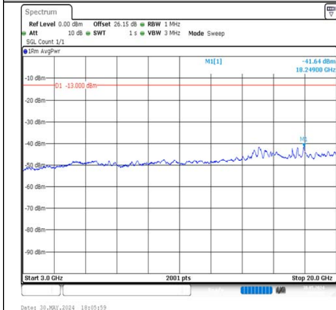
Band4-20MHz-16QAM-20300-100RB#0-3000~20000-PASS
