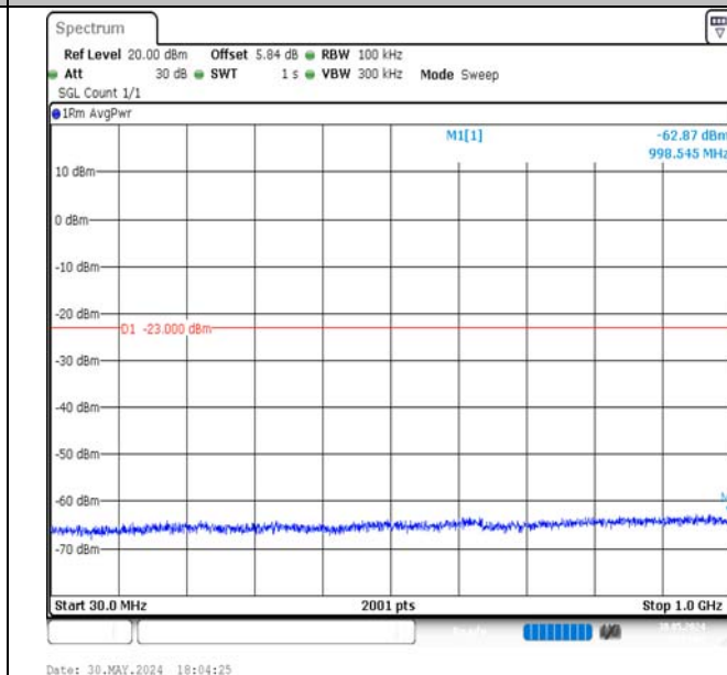
Band4-20MHz-16QAM-20300-1RB#0-30~1000-PASS
