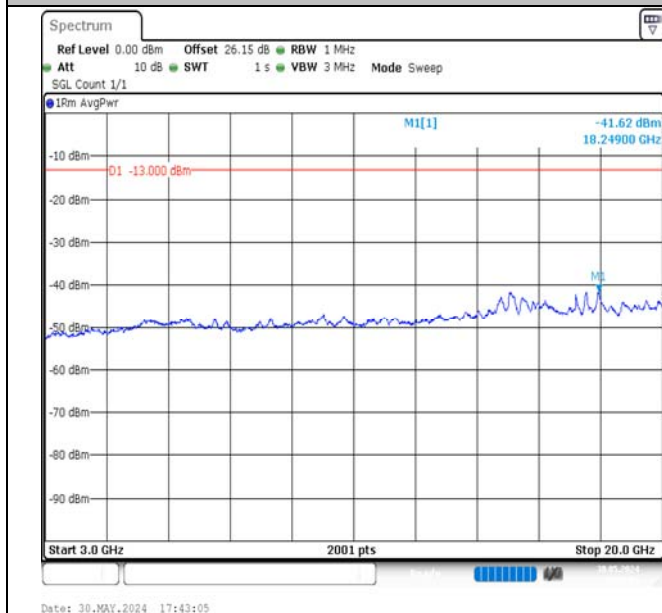
Band4-15MHz-16QAM-20175-1RB#74-3000~20000-PASS
