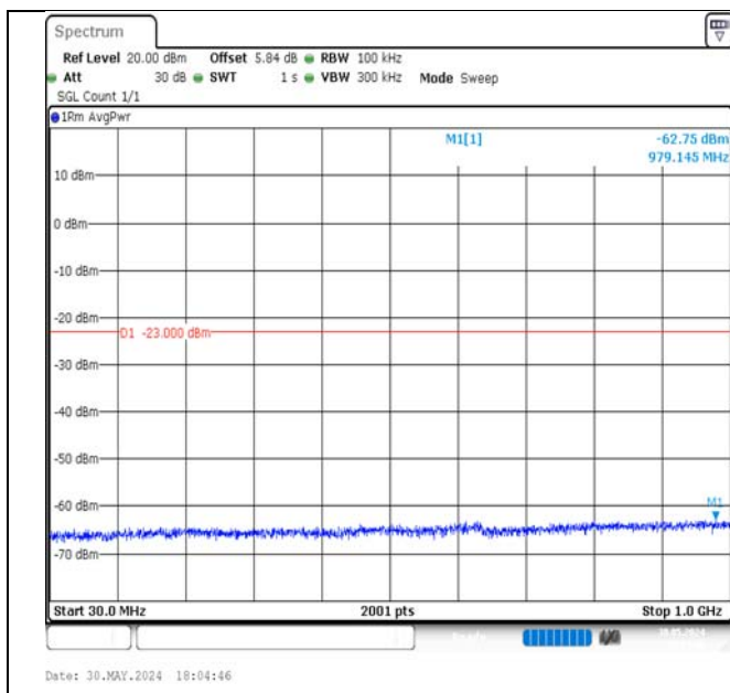
Band4-20MHz-QPSK-20300-1RB#99-30~1000-PASS
