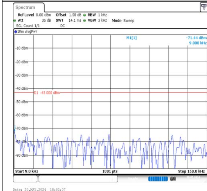
Band4-20MHz-QPSK-20175-100RB#0-0.009~0.15-PASS
