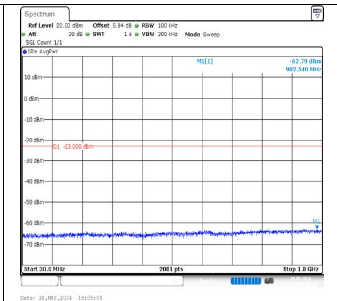
Band4-20MHz-16QAM-20300-1RB#99-30~1000-PASS
