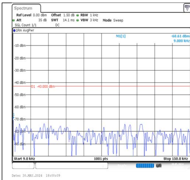
Band4-20MHz-QPSK-20050-1RB#99-0.009~0.15-PASS
