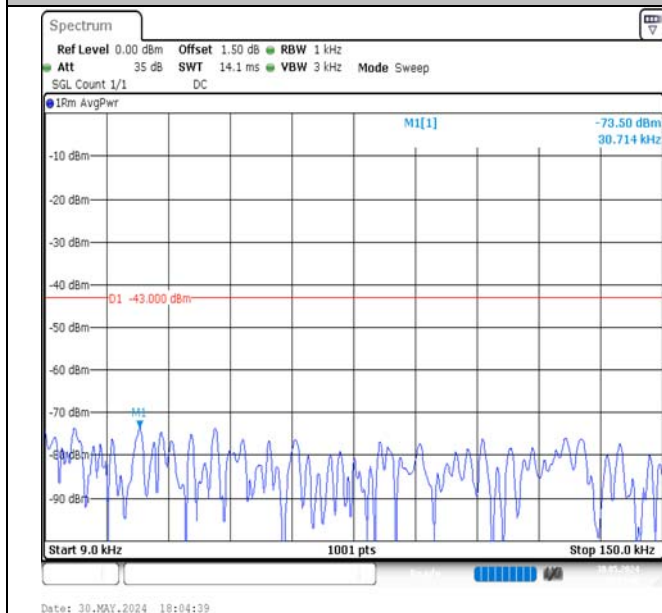
Band4-20MHz-QPSK-20300-1RB#99-0.009~0.15-PASS
