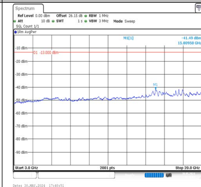
Band4-15MHz-16QAM-20025-1RB#74-3000~20000-PASS
