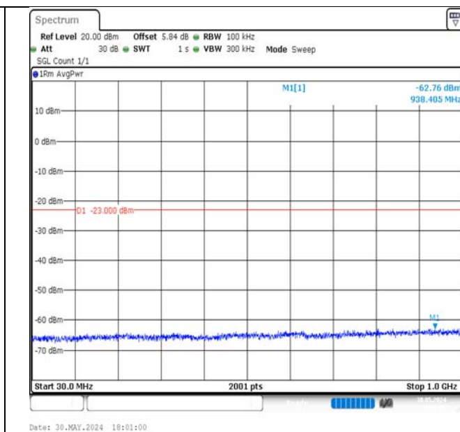
Band4-20MHz-QPSK-20050-100RB#0-30~1000-PASS
