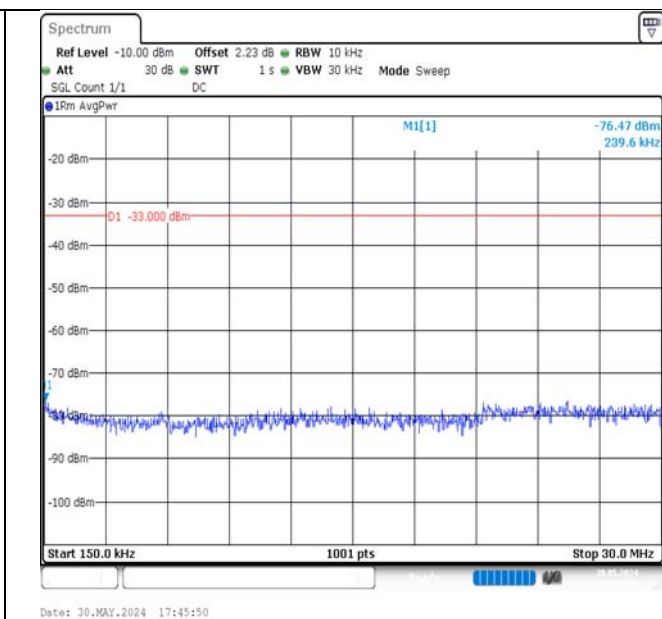
Band4-15MHz-16QAM-20325-75RB#0-0.15~30-PASS
