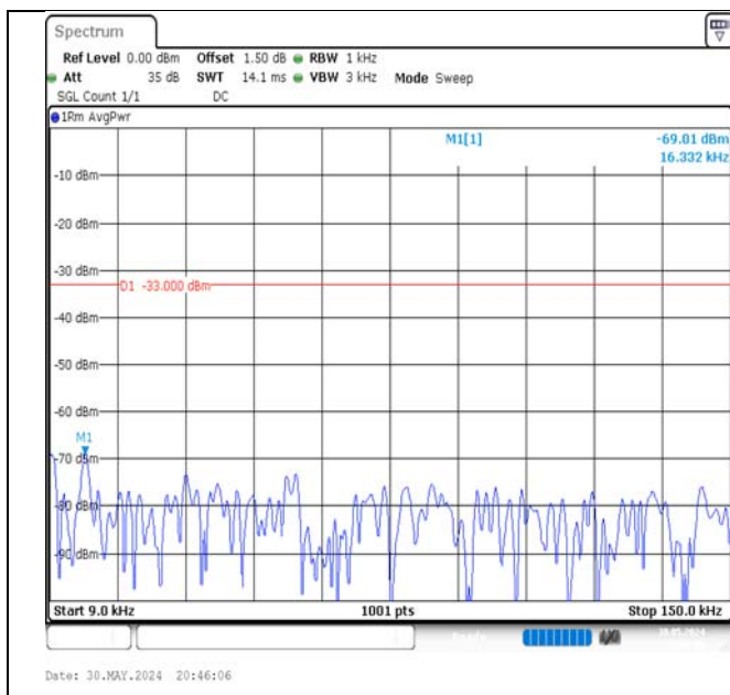
Band5-1.4MHz-QPSK-20407-1RB#0-0.009~0.15-PASS
