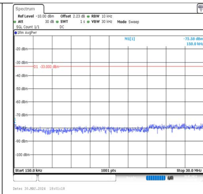
Band4-20MHz-16QAM-20050-100RB#0-0.15~30-PASS
