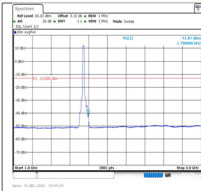
Band4-20MHz-QPSK-20300-100RB#0-1000~3000-PASS
