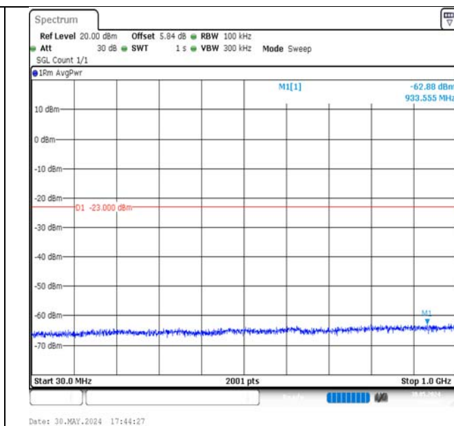
Band4-15MHz-16QAM-20325-1RB#0-30~1000-PASS
