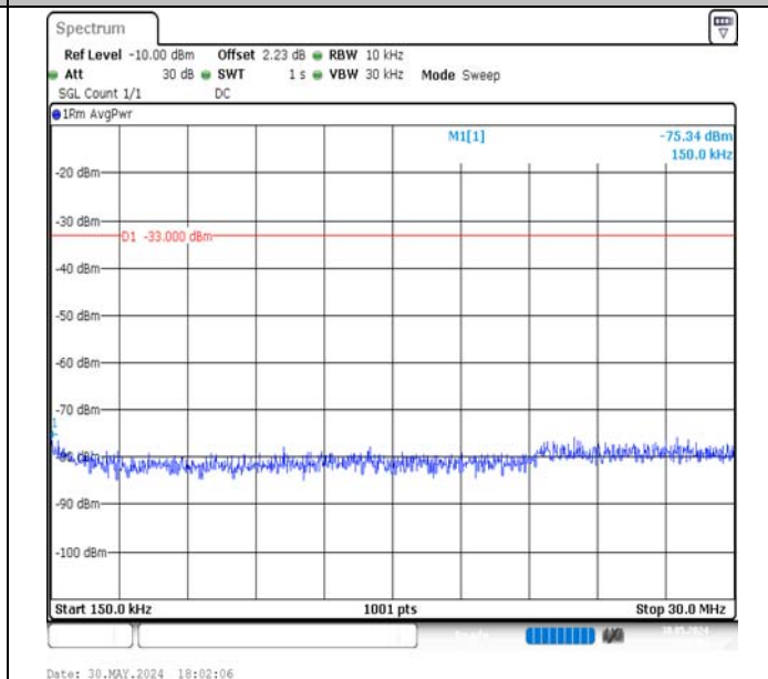
Band4-20MHz-16QAM-20175-1RB#0-0.15~30-PASS
