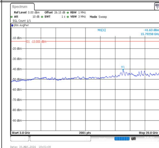
Band4-20MHz-QPSK-20050-100RB#0-3000~20000-PASS
