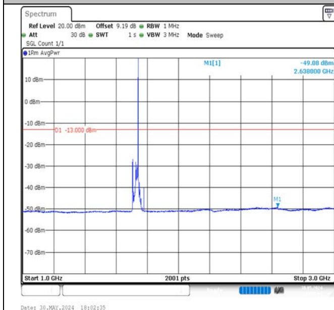
Band4-20MHz-QPSK-20175-1RB#99-1000~3000-PASS
