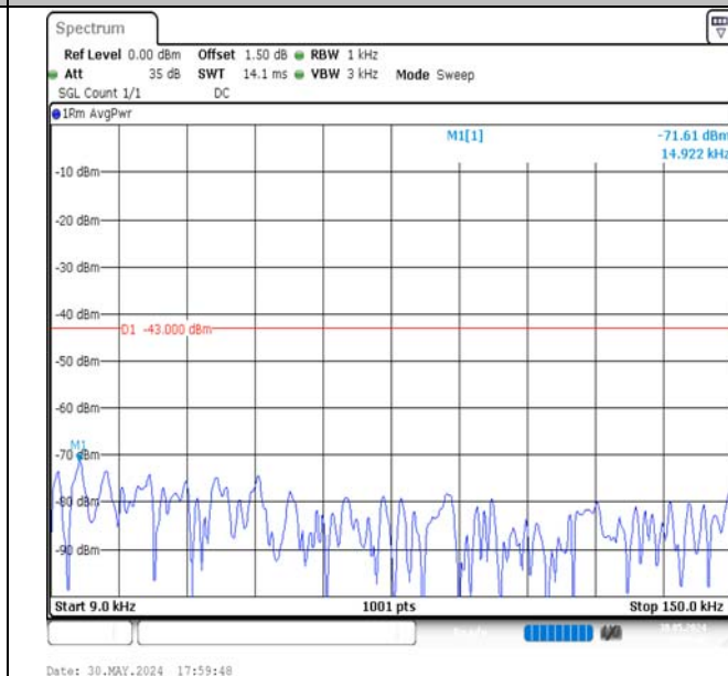
Band4-20MHz-16QAM-20050-1RB#0-0.009~0.15-PASS
