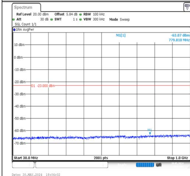
Band4-20MHz-QPSK-20300-1RB#0-30~1000-PASS
