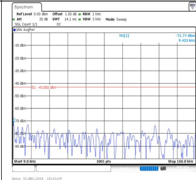
Band4-20MHz-16QAM-20175-100RB#0-0.009~0.15-PASS
