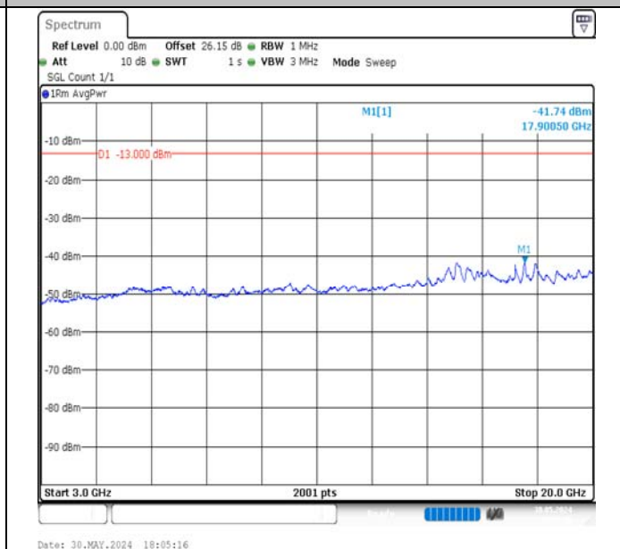
Band4-20MHz-16QAM-20300-1RB#99-3000~20000-PASS
