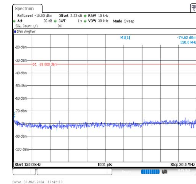
Band4-15MHz-16QAM-20175-1RB#0-0.15~30-PASS
