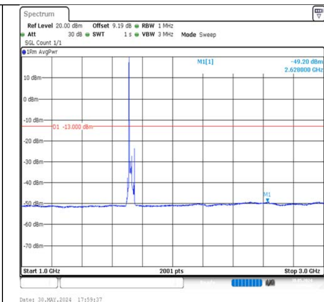
Band4-20MHz-QPSK-20050-1RB#0-1000~3000-PASS
