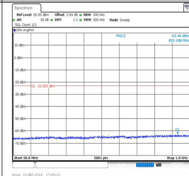
Band4-15MHz-16QAM-20325-1RB#74-30~1000-PASS
