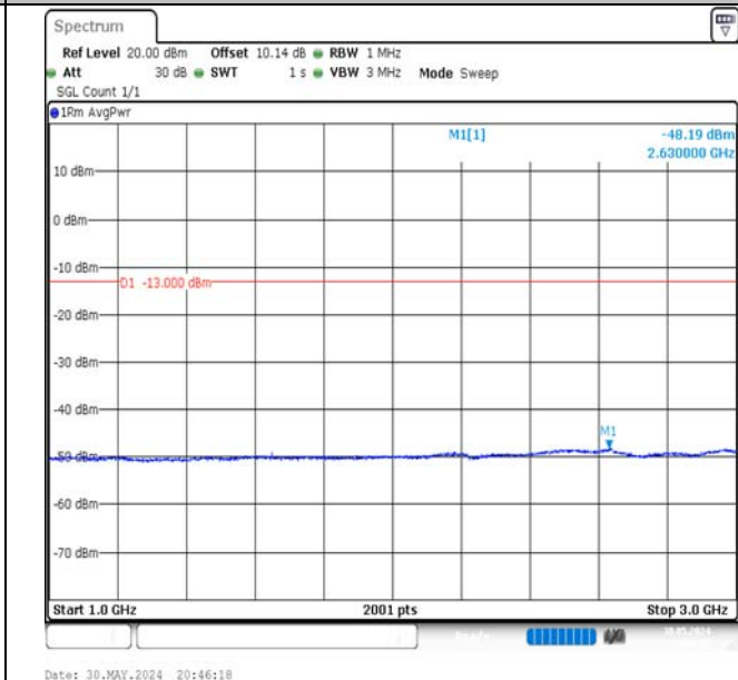
Band5-1.4MHz-QPSK-20407-1RB#0-1000~3000-PASS
