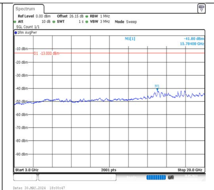
Band4-20MHz-16QAM-20050-1RB#99-3000~20000-PASS
