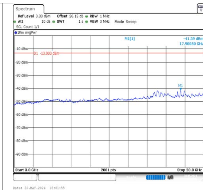
Band4-20MHz-QPSK-20175-1RB#0-3000~20000-PASS
