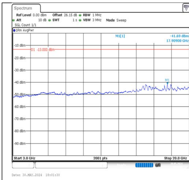
Band4-20MHz-16QAM-20050-100RB#0-3000~20000-PASS
