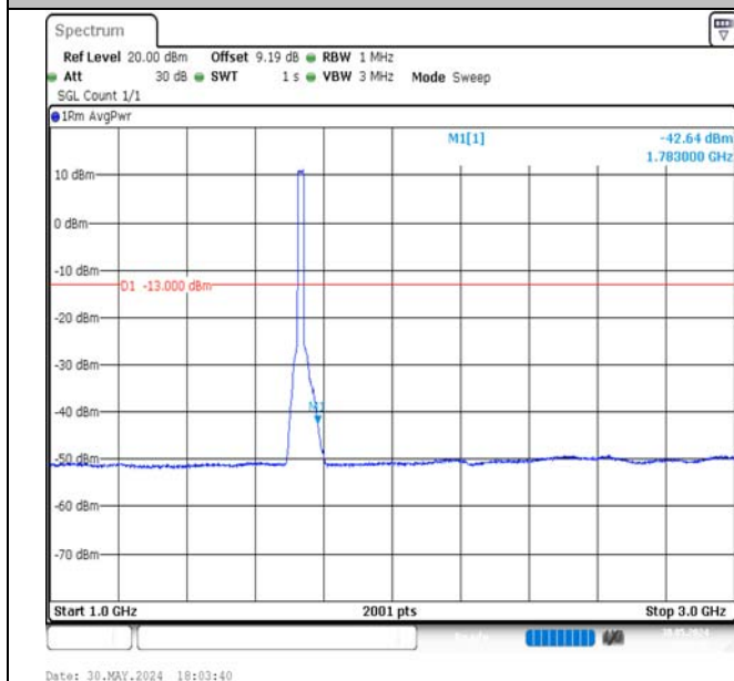
Band4-20MHz-16QAM-20175-100RB#0-1000~3000-PASS
