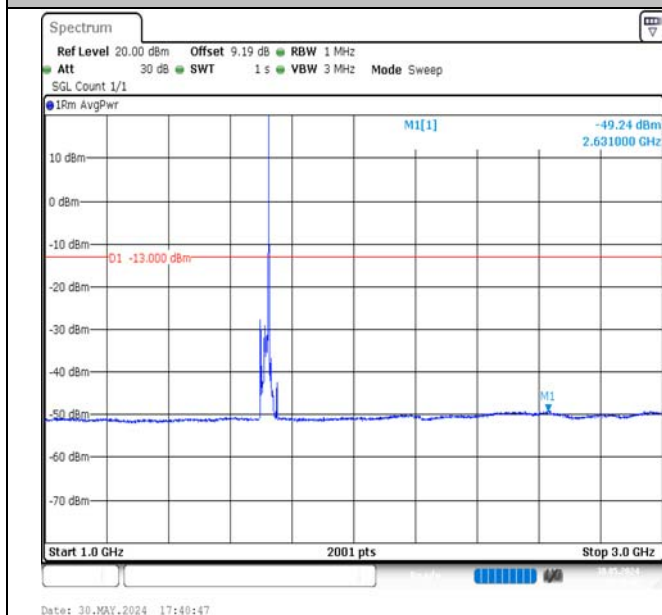
Band4-15MHz-16QAM-20025-1RB#74-1000~3000-PASS
