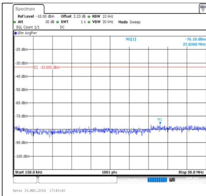
Band4-15MHz-16QAM-20025-1RB#74-0.15~30-PASS
