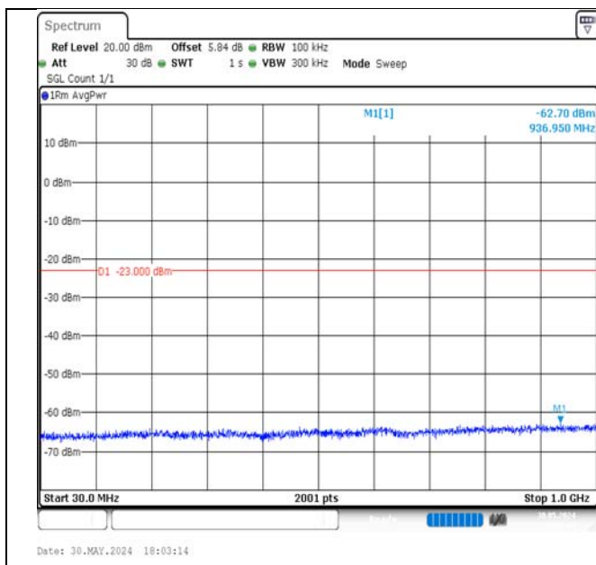
Band4-20MHz-QPSK-20175-100RB#0-30~1000-PASS
