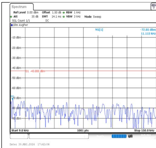
Band4-15MHz-16QAM-20175-1RB#0-0.009~0.15-PASS
