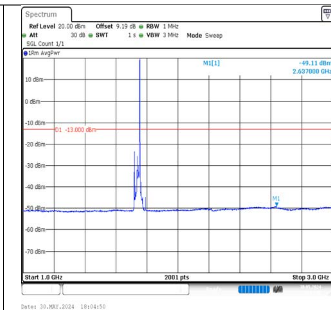
Band4-20MHz-QPSK-20300-1RB#99-1000~3000-PASS
