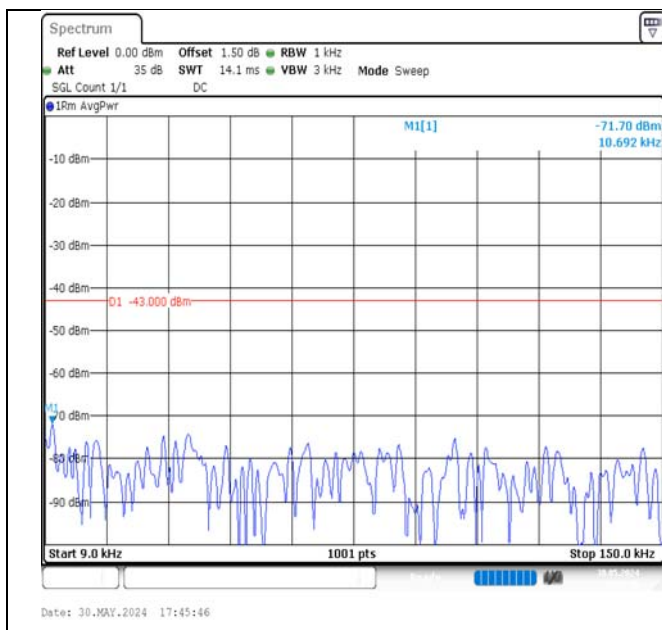
Band4-15MHz-16QAM-20325-75RB#0-0.009~0.15-PASS
