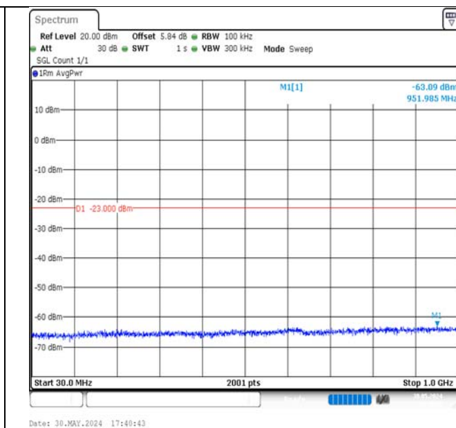
Band4-15MHz-16QAM-20025-1RB#74-30~1000-PASS
