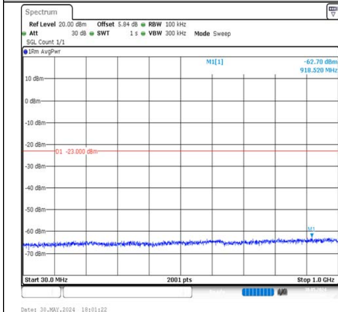
Band4-20MHz-16QAM-20050-100RB#0-30~1000-PASS
