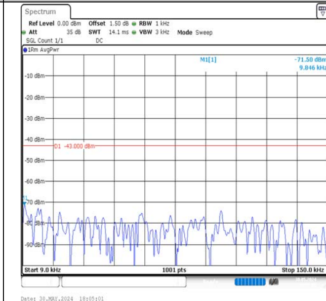
Band4-20MHz-16QAM-20300-1RB#99-0.009~0.15-PASS
