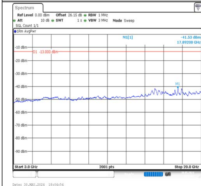
Band4-20MHz-QPSK-20300-1RB#99-3000~20000-PASS
