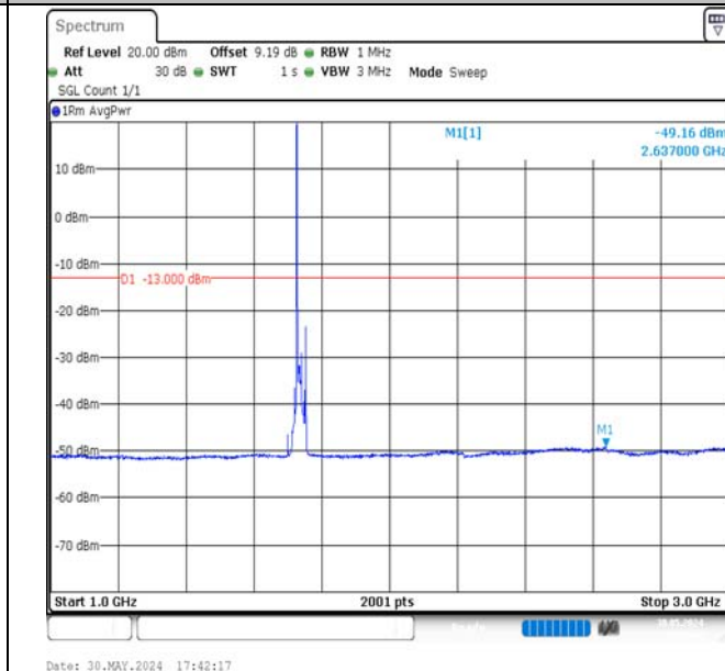
Band4-15MHz-16QAM-20175-1RB#0-1000~3000-PASS
