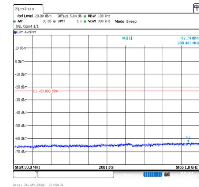
Band4-20MHz-QPSK-20175-1RB#99-30~1000-PASS
