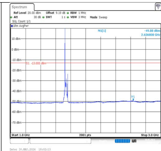
Band4-20MHz-16QAM-20175-1RB#0-1000~3000-PASS
