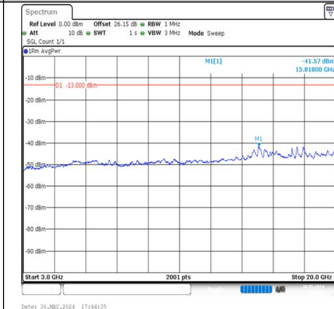
Band4-15MHz-16QAM-20325-1RB#0-3000~20000-PASS
