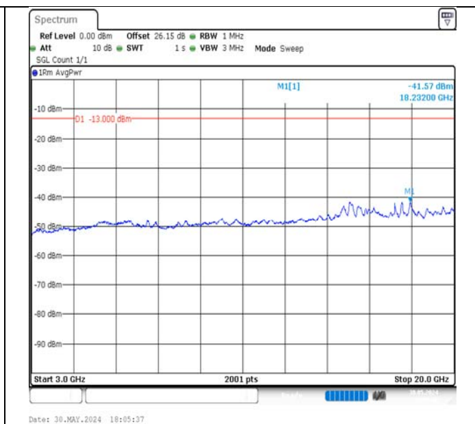
Band4-20MHz-QPSK-20300-100RB#0-3000~20000-PASS
