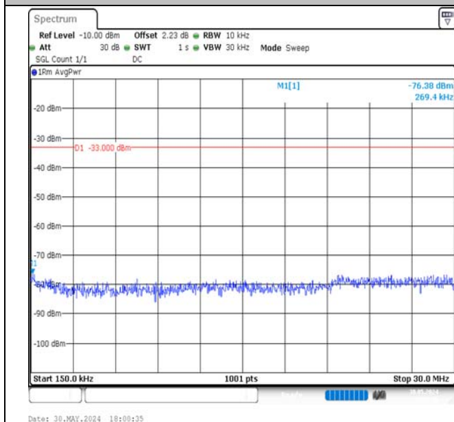
Band4-20MHz-16QAM-20050-1RB#99-0.15~30-PASS
