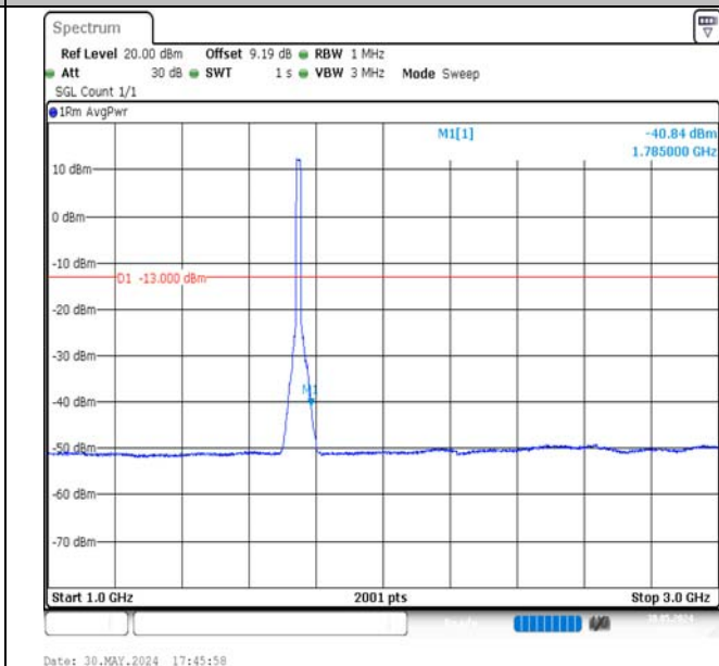
Band4-15MHz-16QAM-20325-75RB#0-1000~3000-PASS
