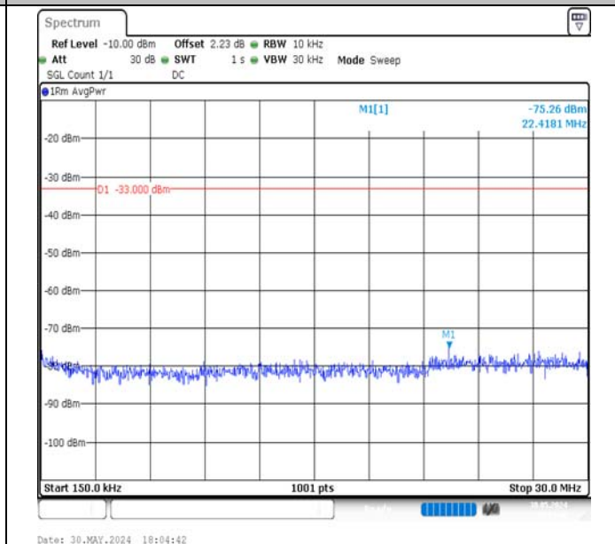
Band4-20MHz-QPSK-20300-1RB#99-0.15~30-PASS
