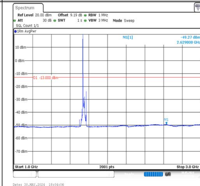
Band4-20MHz-QPSK-20300-1RB#0-1000~3000-PASS
